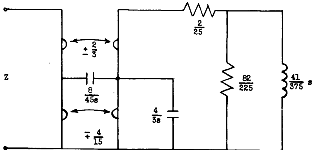
Fig. (3-20) m-Type Rank 4 Capacitive
