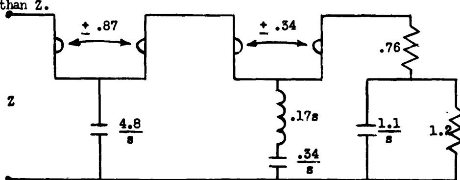
Fig. (5-6) n-Type Transformerless Synthesis
