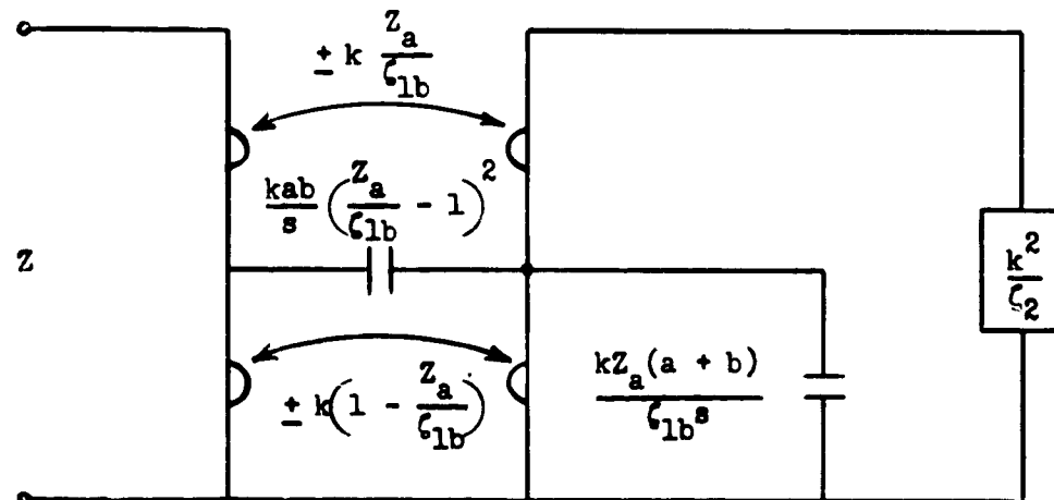
Fig. (3-15) m-Type Rank 4 Capacitive
