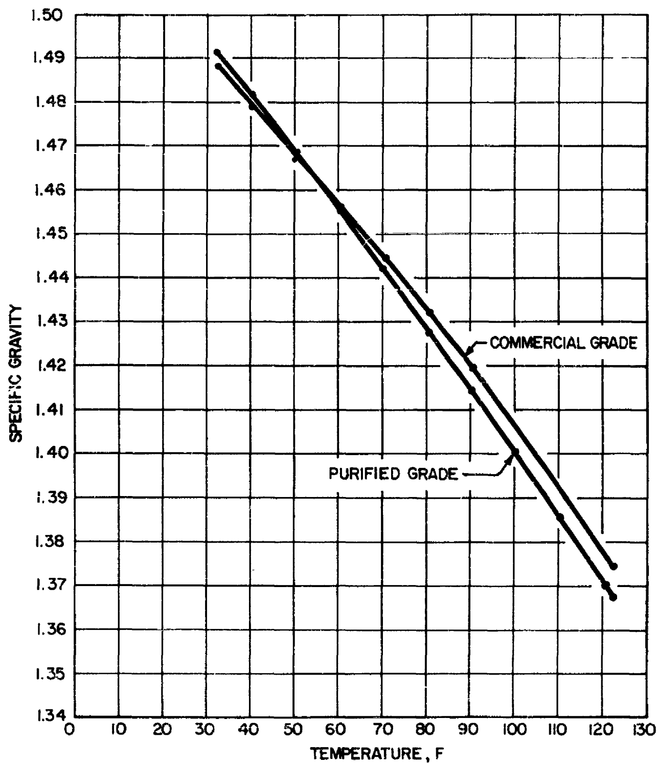
Figure 1. Specific Gravity of Nitrogen Tetroxide
