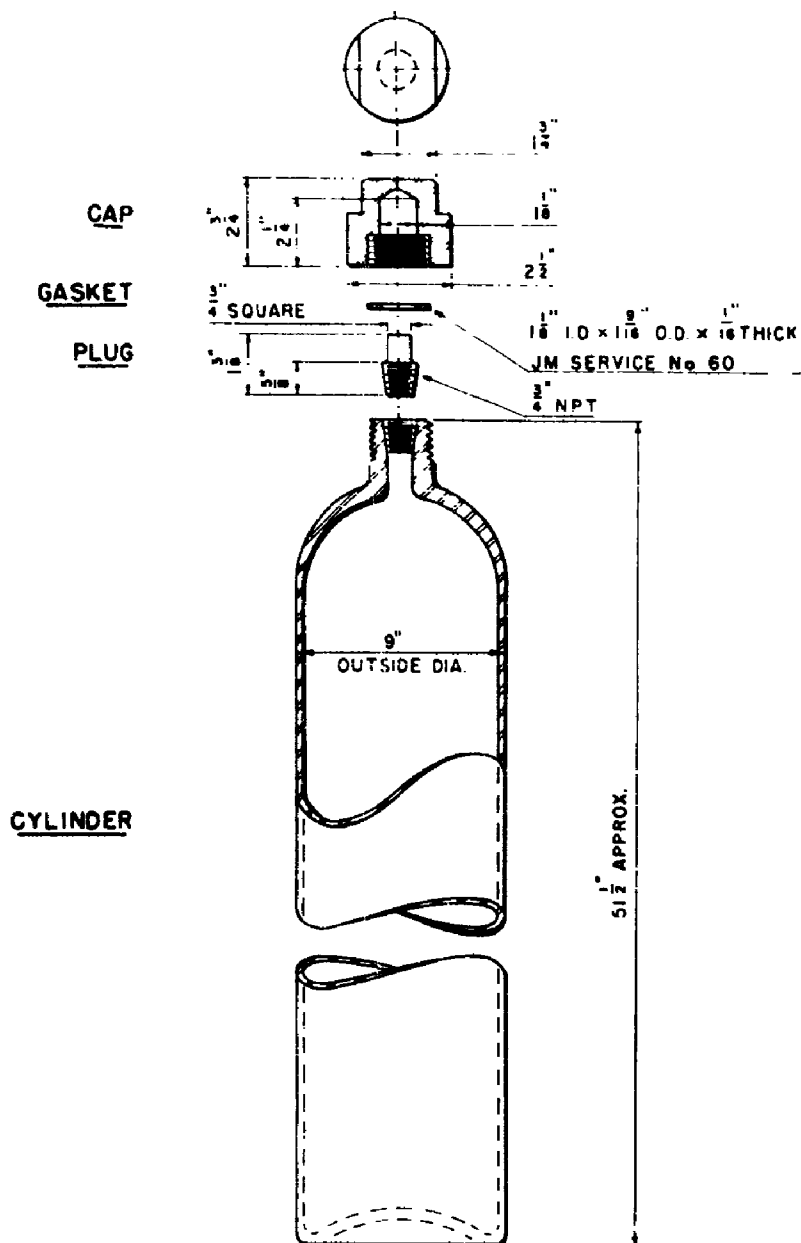
CYLINDER SPECIFICATION ICC-3A1800 TARE WEIGHT (APPROX.) 127 LBS.
