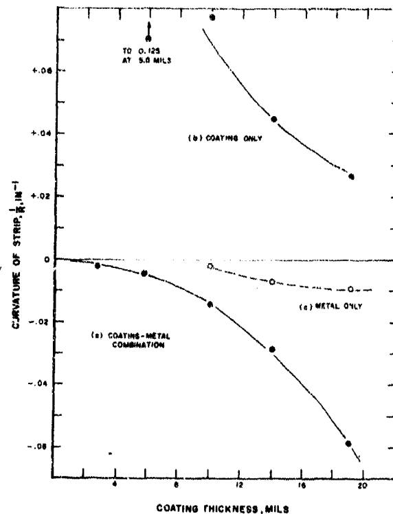
Figure 27. Curvature of strips with thickness. (Negative curvature values in curve (a) signifies coating was on convex side of specimen).
