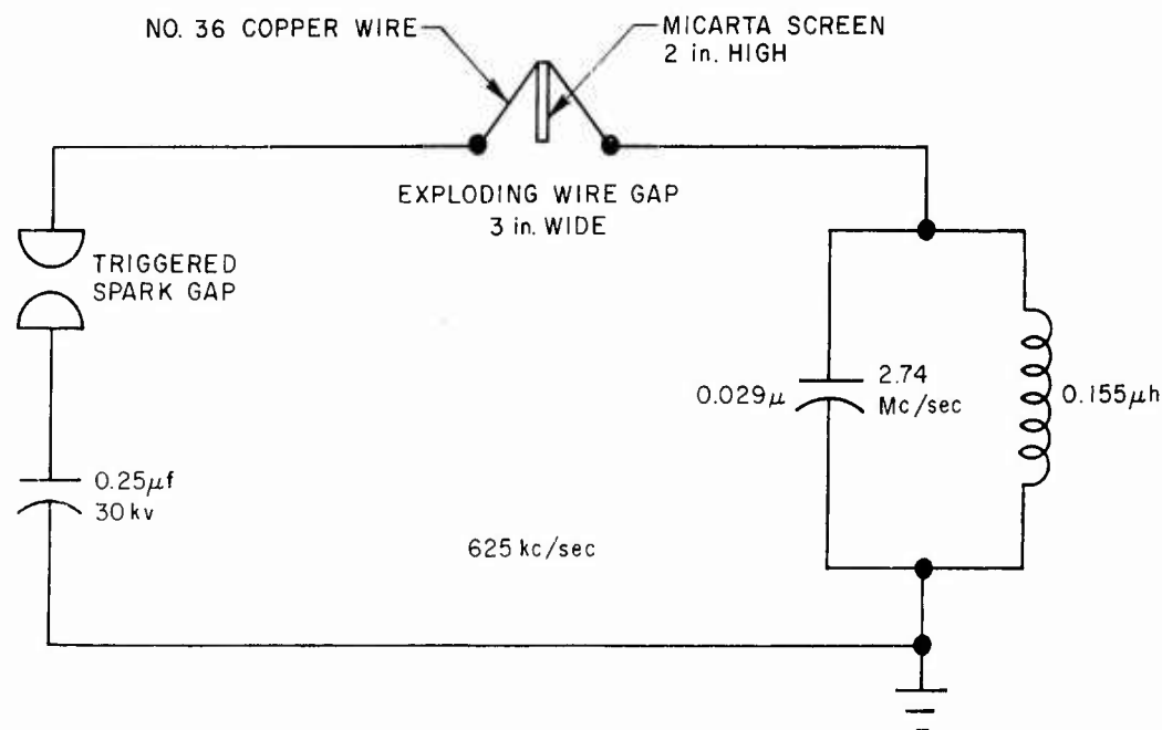
Fig. 1. Circuit diagram.
