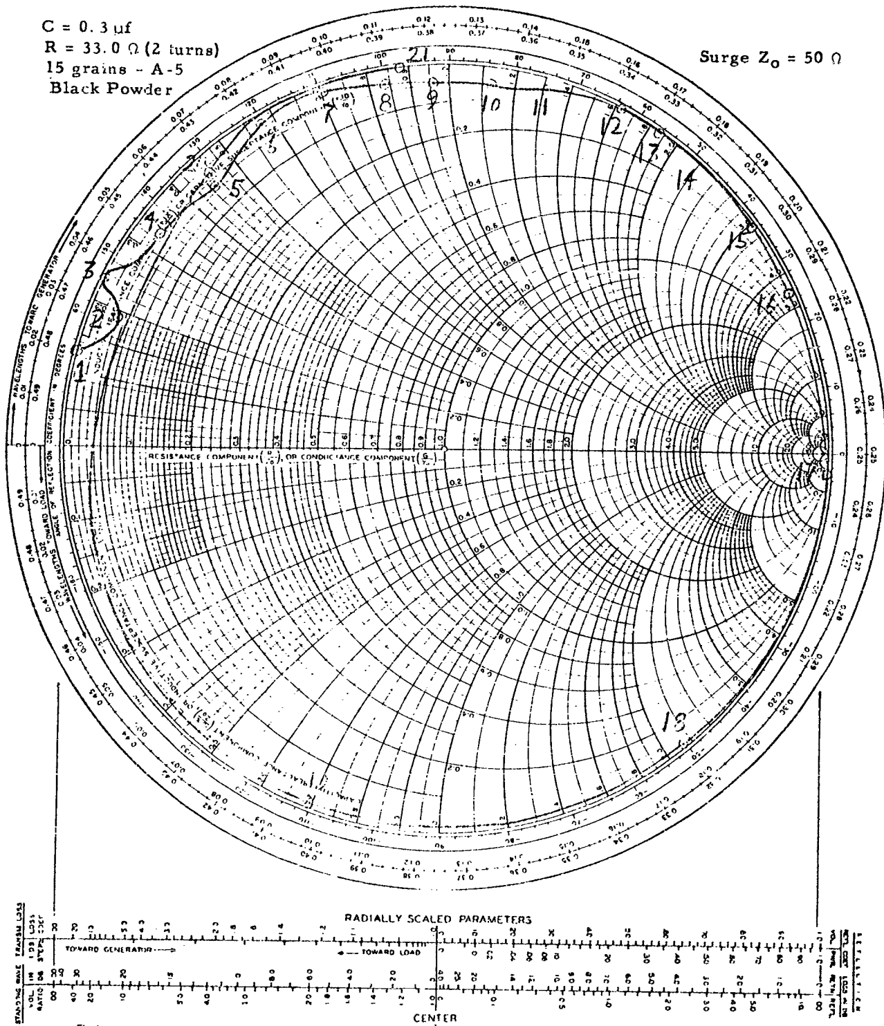
Fig. 46 - Impedance Measurements at Various Frequencies Using a Complete Squib Assembly w/American Lava Corporation Capacitance Assembly
