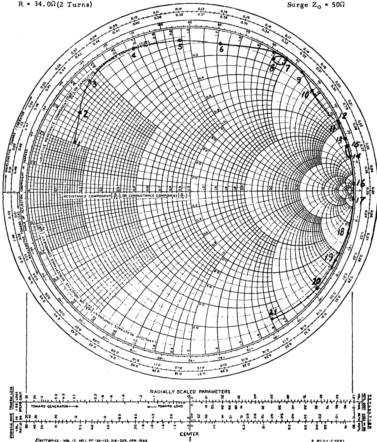
Fig. 35 - Impedance Measurements at Various Frequencies Using Erie Resistor Corporation Capacitance Assembly
