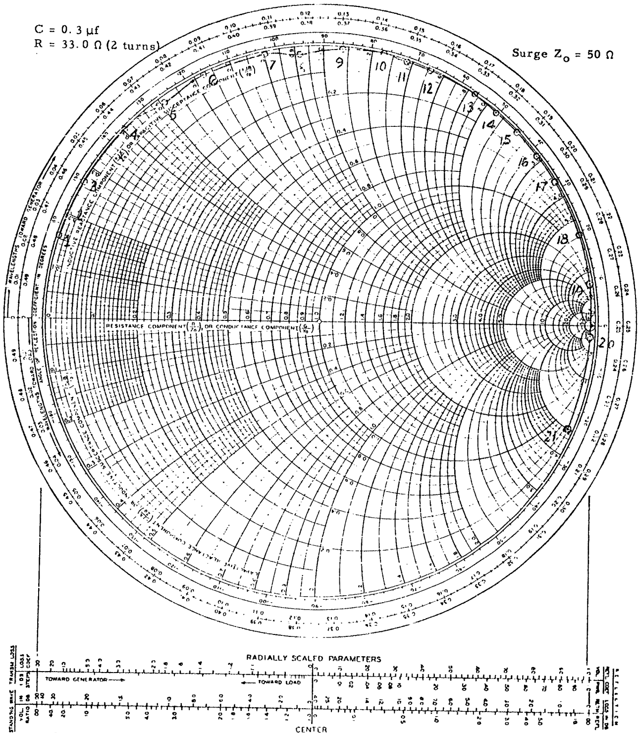
Fig. 44 - Impedance Measurements at Various Frequencies Using American Lava Corporation Capacitance Assembly
