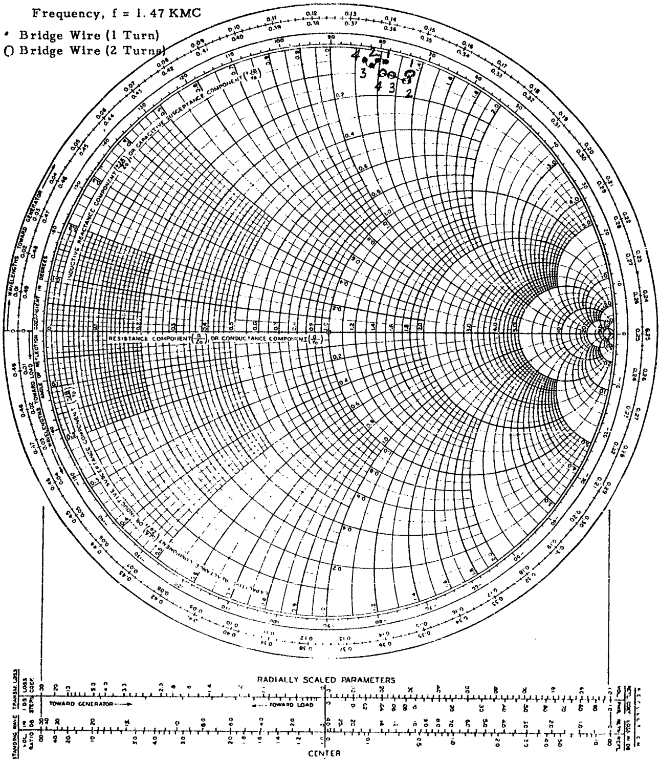
Fig. 55 - Impedance vs Radio-Frequency Power Level Using a Complete Squib Assembly incorporating American Lava Corporation elements.
