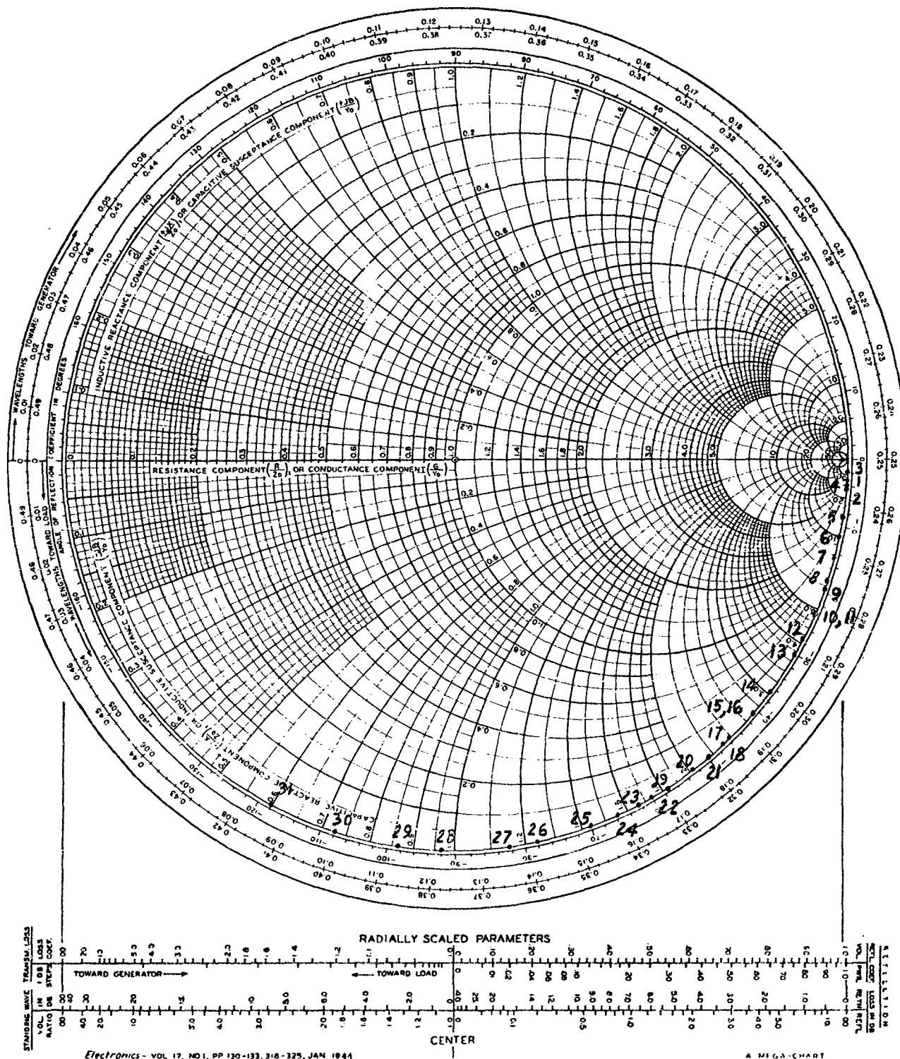
Fig. 30 - Impedance Measurements at Various Frequencies Using the Carborundum Company Ceramic Seal
