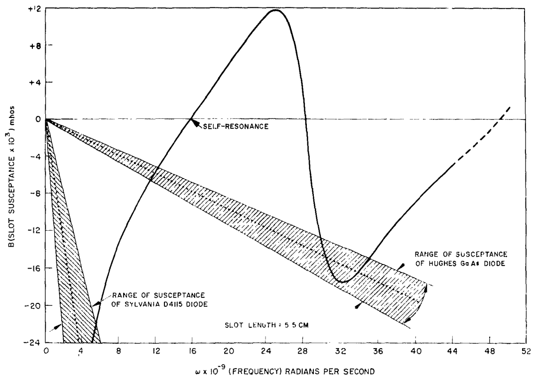
Figure 7a. Slot susceptance as a function of \omega .
