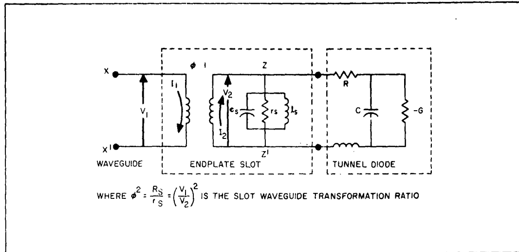
Figure 4a. Equivalent circuit of tunnel diode slot configuration referred to waveguide input terminals.
