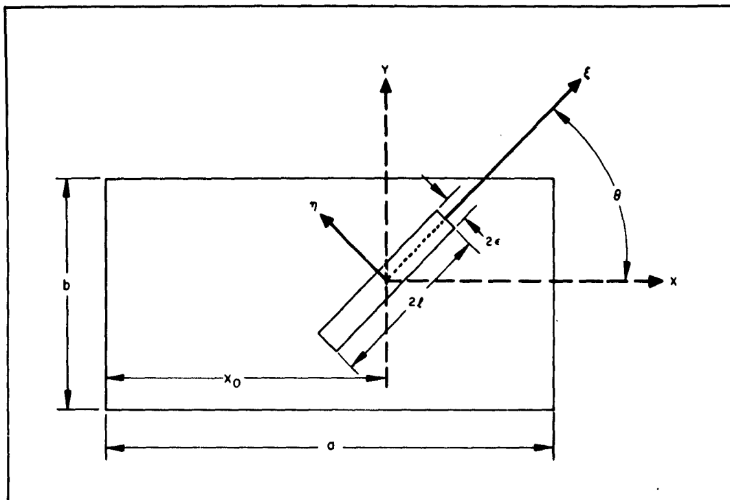
Figure 5a. Endplate slot position and orientation.
