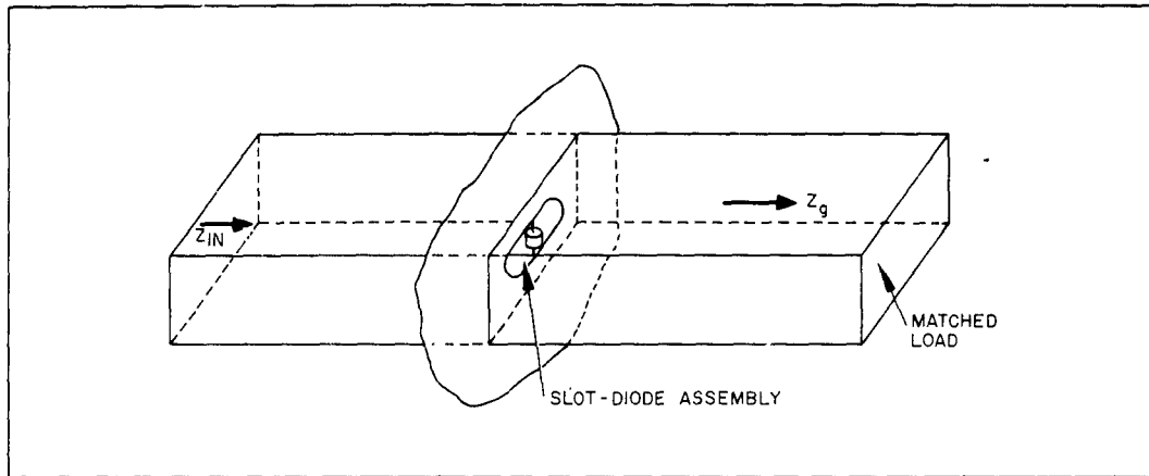
Figure 6a. Sketch of endplate slot-diode assembly acting as a guide-to-guide coupler.
