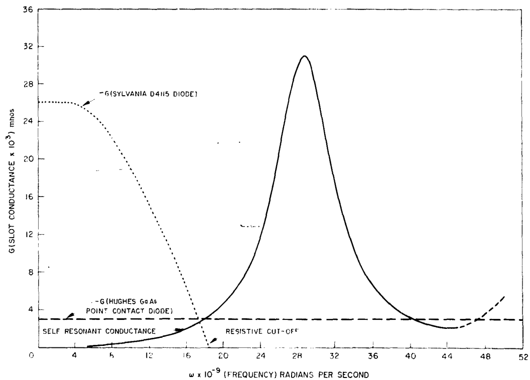
Figure 7b. Slot conductance as a function of \omega .
