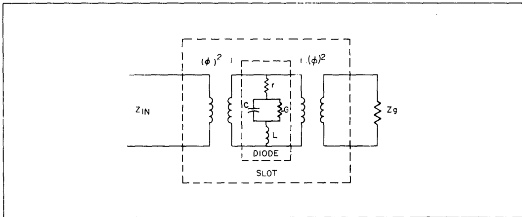
Figure 6b. Equivalent circuit of endplate slot-diode guide-to-guide coupler.
