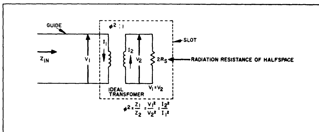
Figure 5b. Equivalent transformer-endplate slot.
