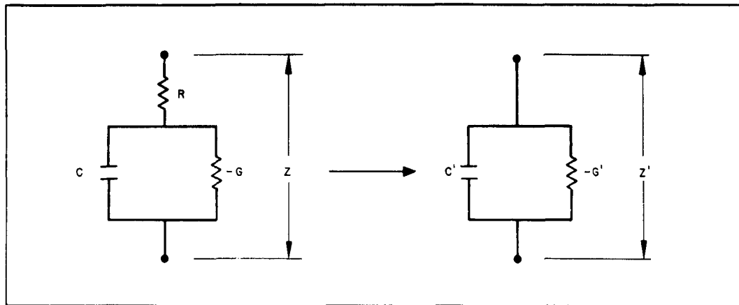
Figure 8a. Tunnel diode simplified equivalent circuits.
