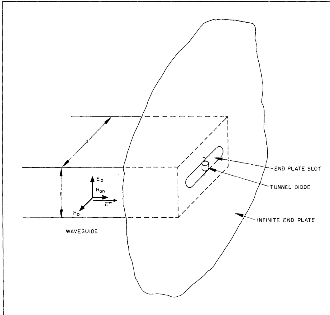
Figure 1. Endplate slot containing a tunnel diode.
