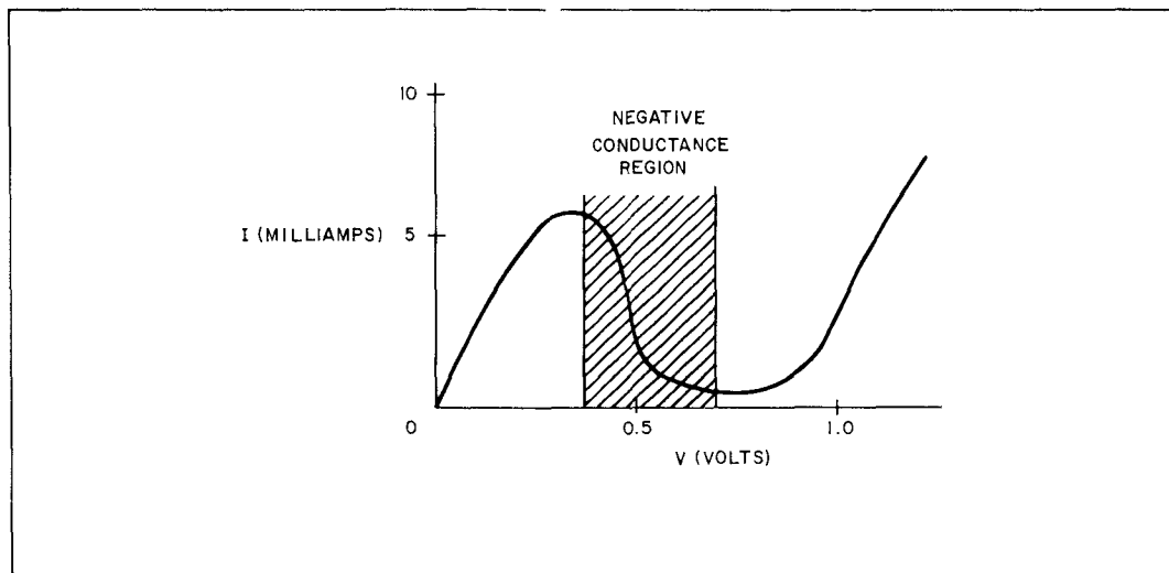
Figure 3b. Typical current versus voltage characteristic of a tunnel diode.
