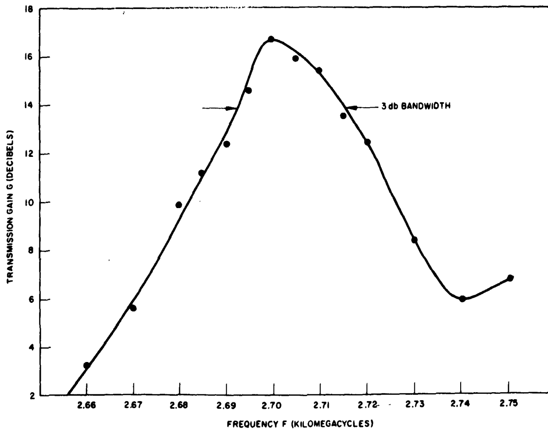
Figure 11. Transmission gain as a function of frequency for the tunnel diode slot amplifier.
