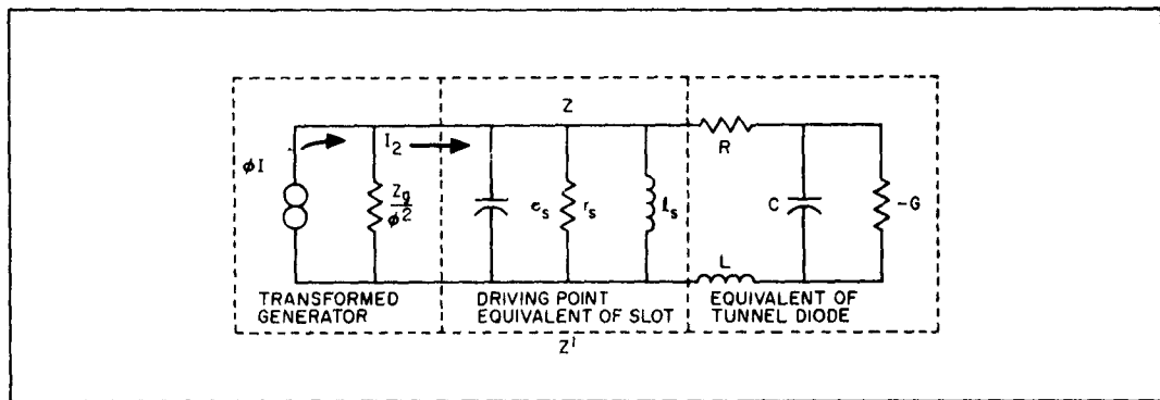
Figure 4b. Equivalent circuit of tunnel diode slot transmission amplifier including matched generator at waveguide input.
