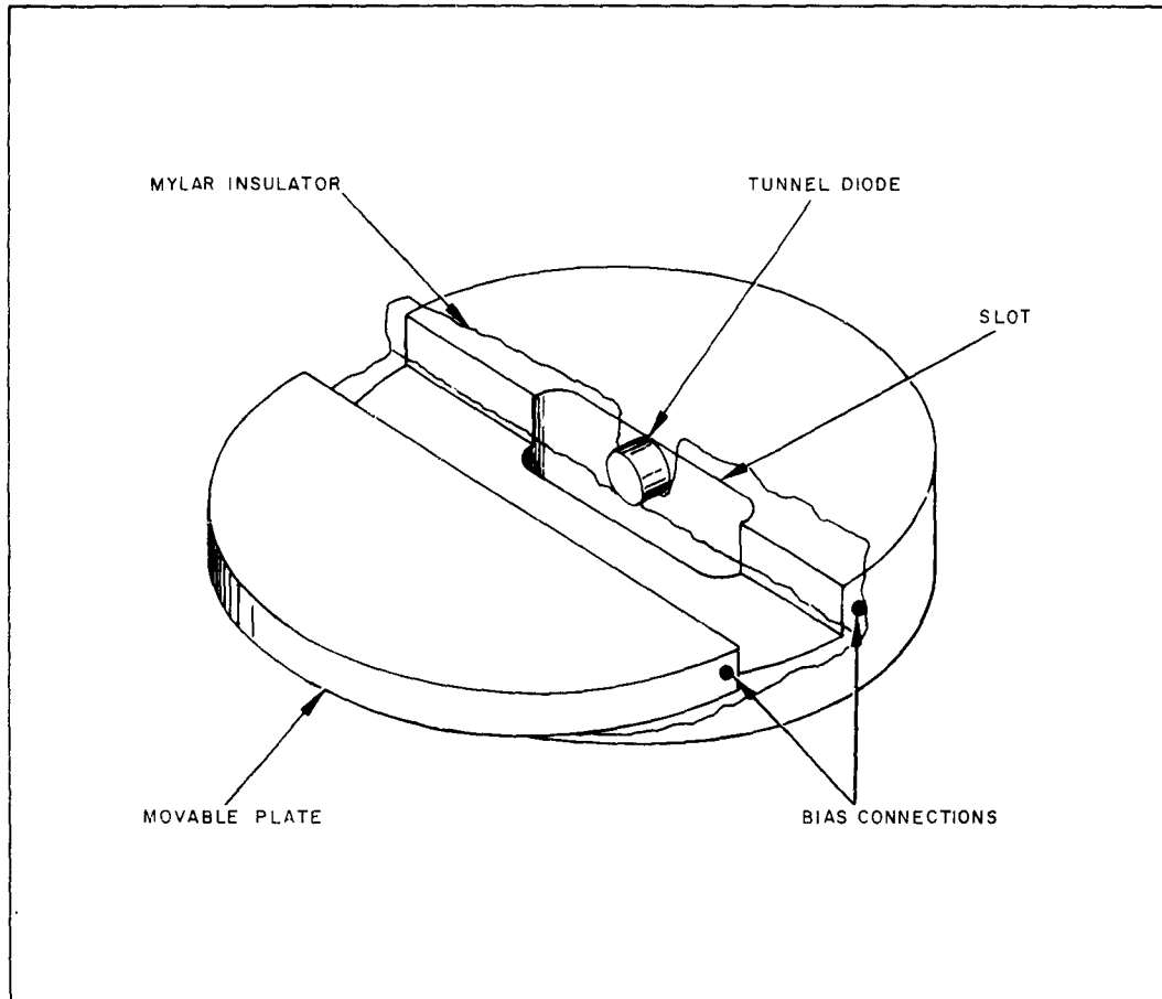
Figure 10. Solid state antenna configuration.
