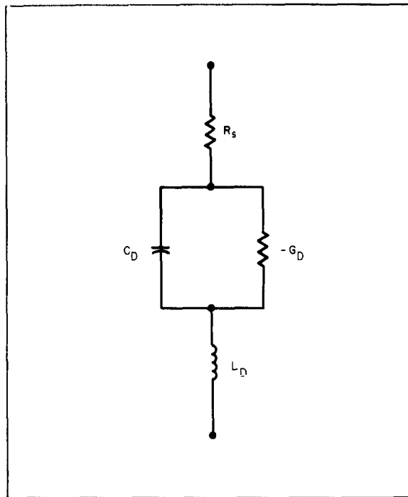
Figure 3a. Equivalent circuit of tunnel diode biased into the negative conductance region
