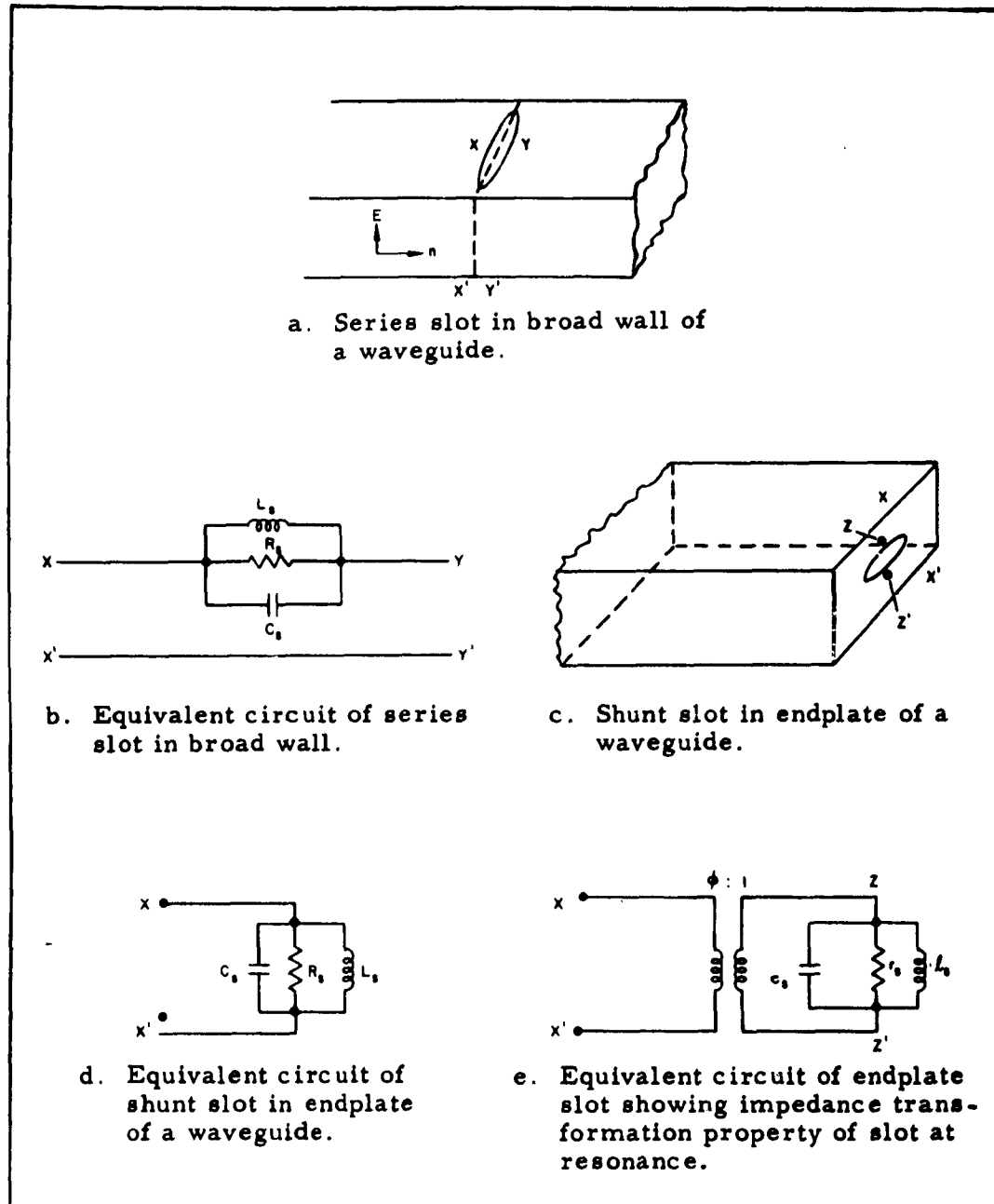
Figure 2. Geometrical representation and circuit equivalents of slots.
