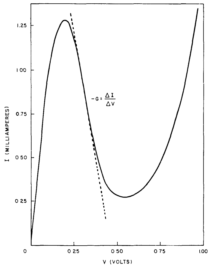
Figure 8b. I-V characteristic of Hughes PC-3 GaAs tunnel diode.
