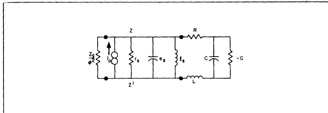
Figure 4c. Equivalent circuit of tunnel diode receiving amplifier.
