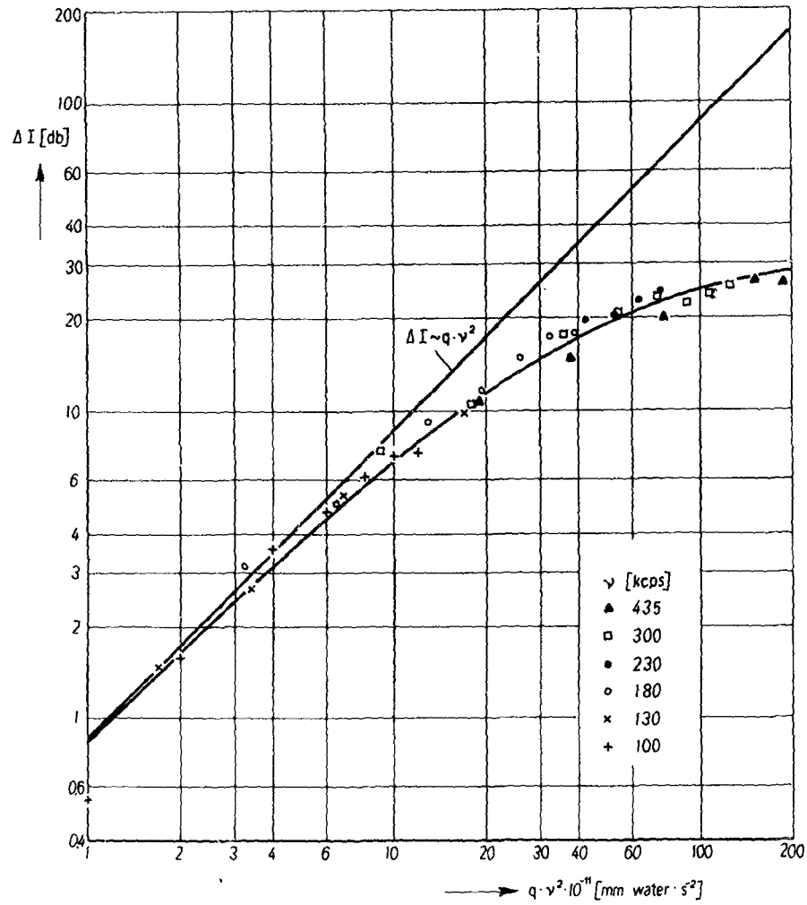
Fig.14: Damping \Delta I of sound vs. the product of the dynamic pressure q of the main flow and the square of the sound frequency \nu . Data of the tests: s = 30.0 cm; D = 0.40 cm; M = 2.50 cm; d = 5.0 cm.
