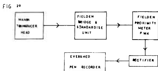
SCHEMATIC DIAGRAM OF CIRCUIT ADOPTED
