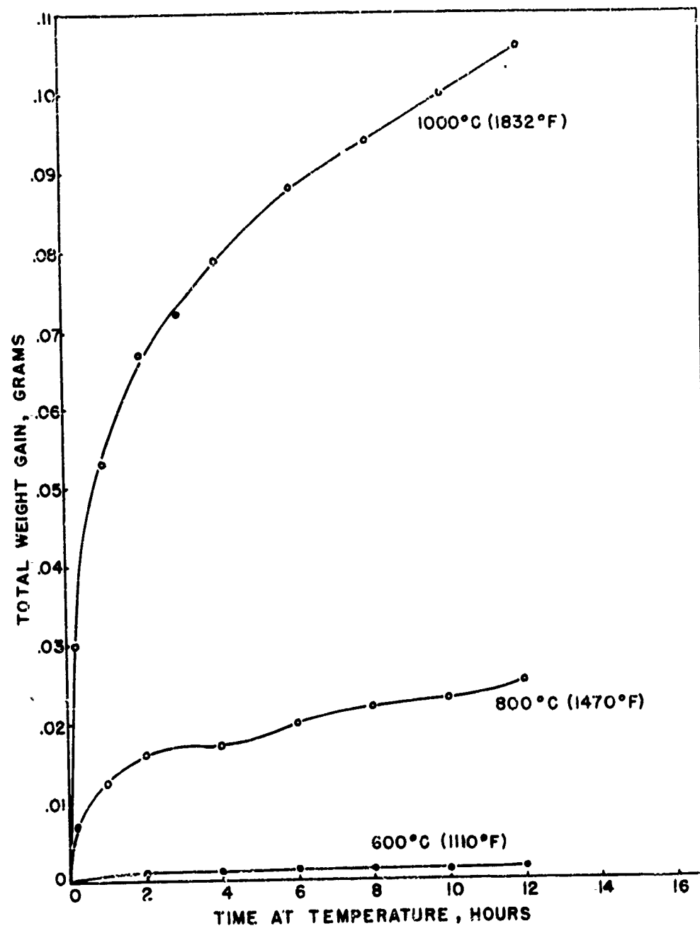
FIG. 35 RATE OF OXIDATION OF TIN AT DIFFERENT TEMPERATURES. INITIAL WEIGHT OF SPECIMENS, APPROXIMATELY 6.5 GRAMS.
