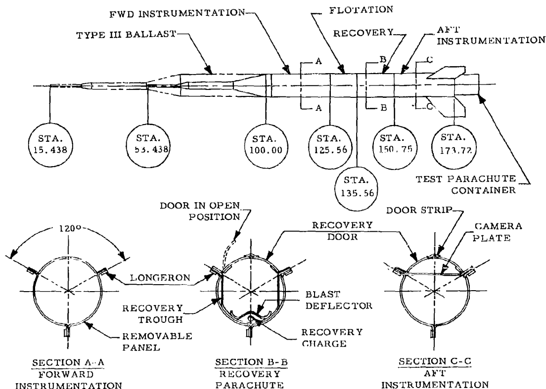
Figure 6. Model 59 Cree Missile Structure
