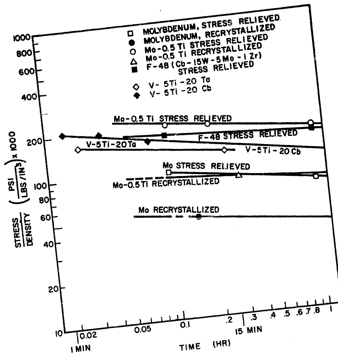
FIG. 9.14 STRESS-DENSITY VS RUPTURE TIME FOR SELECTED VANADIUM, COLUMBIUM, AND MOLYBDENUM ALLOYS AT 2000°F IN HELIUM
