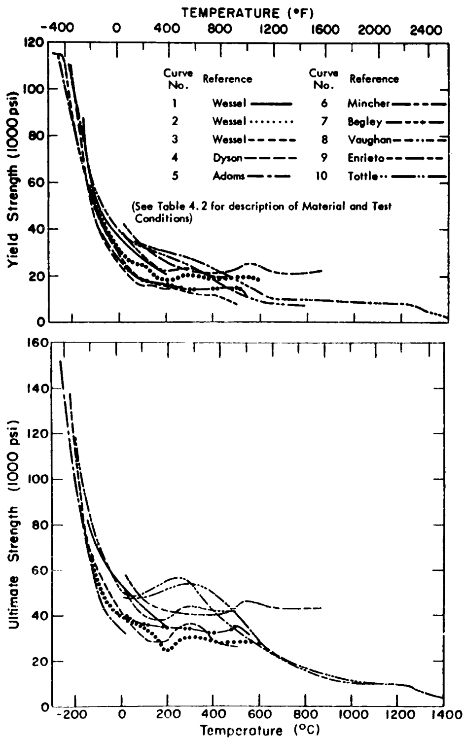
FIG. 4.2 YIELD STRENGTH AND ULTIMATE TENSILE STRENGTH OF COLUMBIUM VS TEST TEMPERATURE 5
