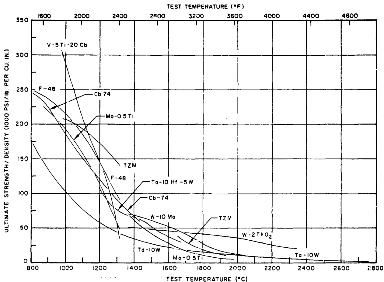
FIG. 2.11 ULTIMATE TENSILE STRENGTH - DENSITY RATIO VS. TEST TEMPERATURE FOR SELECTED REFRACTORY ALLOYS
