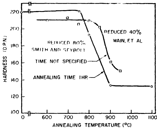
FIG. 3.6 HARDNESS OF CHROMIUM VS ANNEALING TEMPERATURE AFTER ROLLING 40% AND 80% AT 600°C
