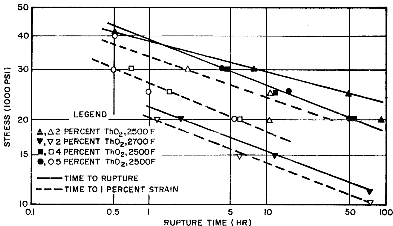
FIG. 8.28 CREEP STRESS VS RUPTURE TIME FOR THORIATED TUNGSTEN BAR ALLOYS (41) 4 AFTER 19
