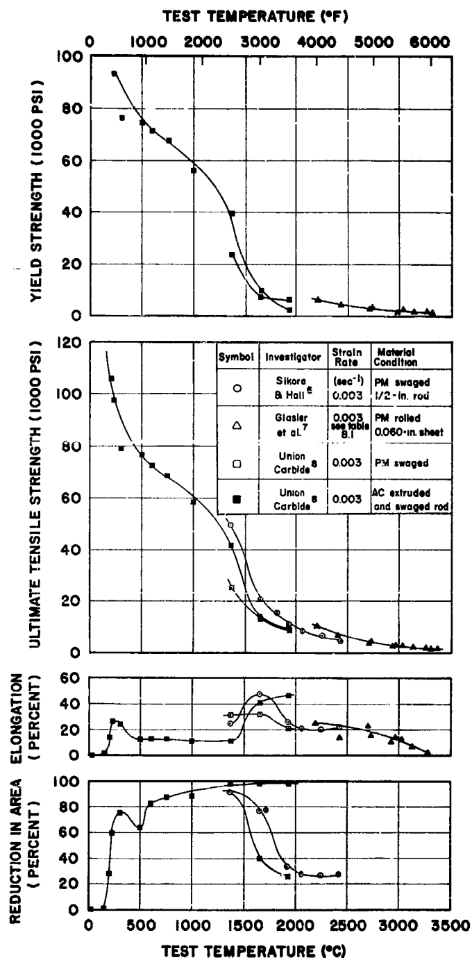
FIG. 8.2 TENSILE PROPERTIES OF WROUGHT TUNGSTEN FROM 25 TO 3400° C (75 TO 6150° F) IN AN INERT ATMOSPHERE
