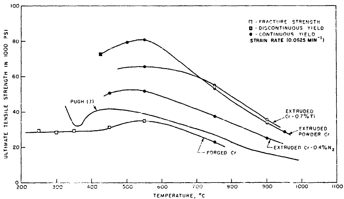
FIG. 3.9 YIELD AND ULTIMATE TENSILE STRENGTH OF CHROMIUM ALLOYS VS TEST TEMPERATURE 5
