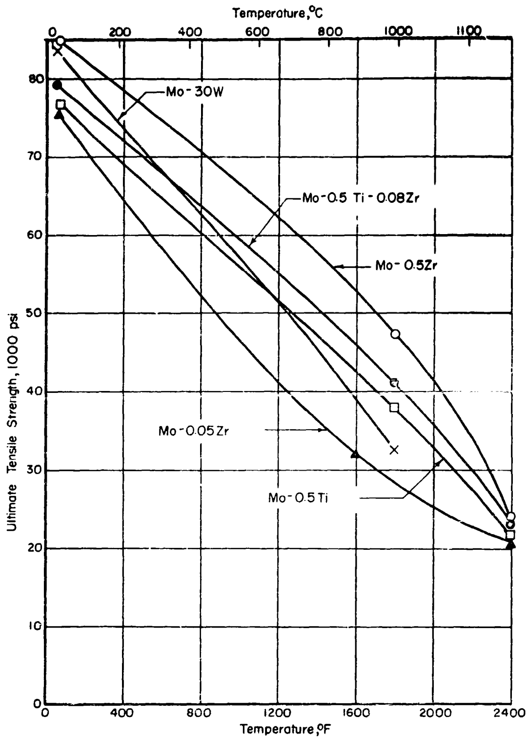
FIG. 5.19 ULTIMATE TENSILE STRENGTH BETWEEN 75 AND 2400° F FOR SELECTED MOLYBDENUM-BASE ALLOY BAR STOCK IN THE RECRYSTALLIZED CONDITION 3
