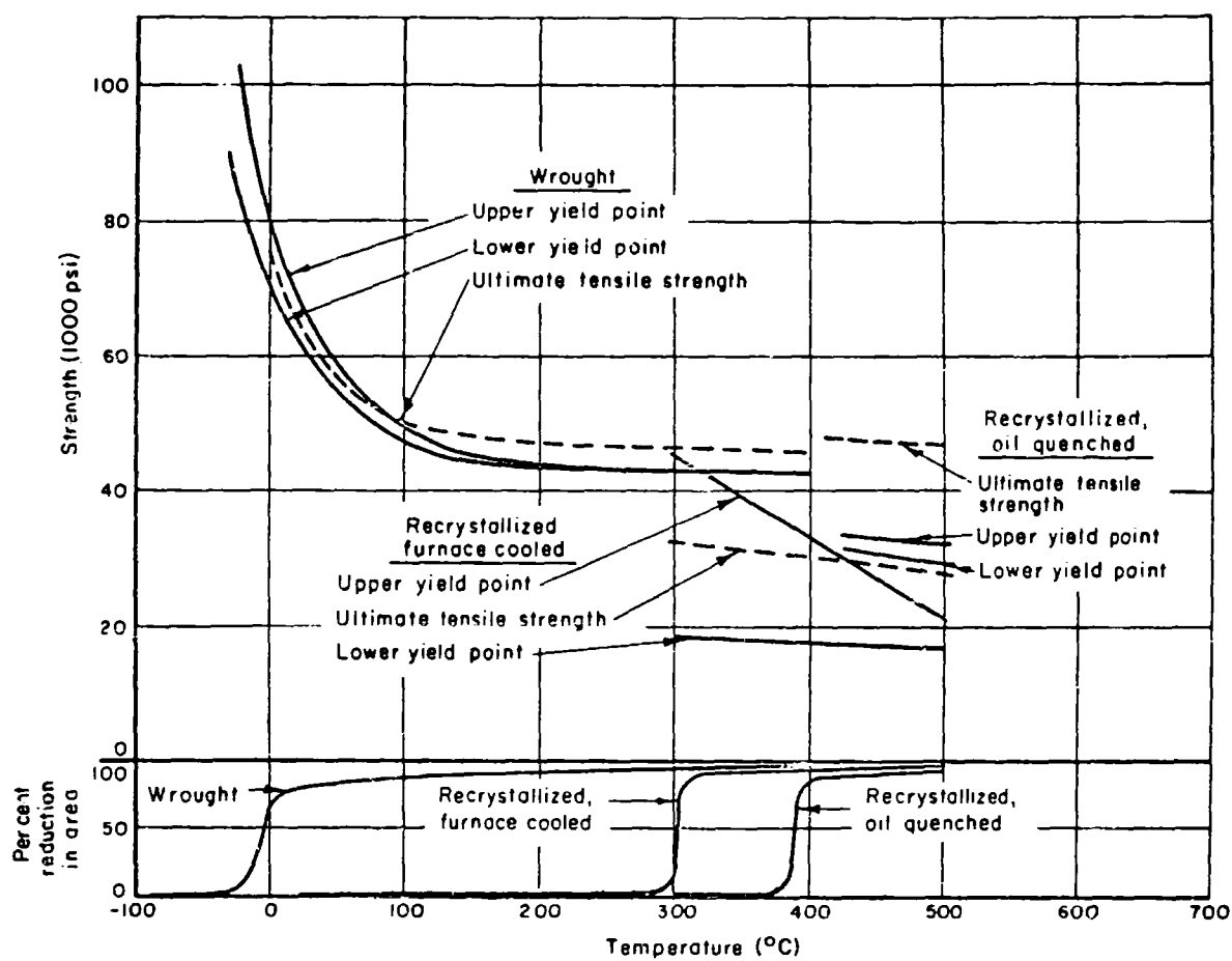
FIG. 3.5 TENSILE PROPERTIES OF UNALLOYED IODIDE CHROMIUM, ICr-2
