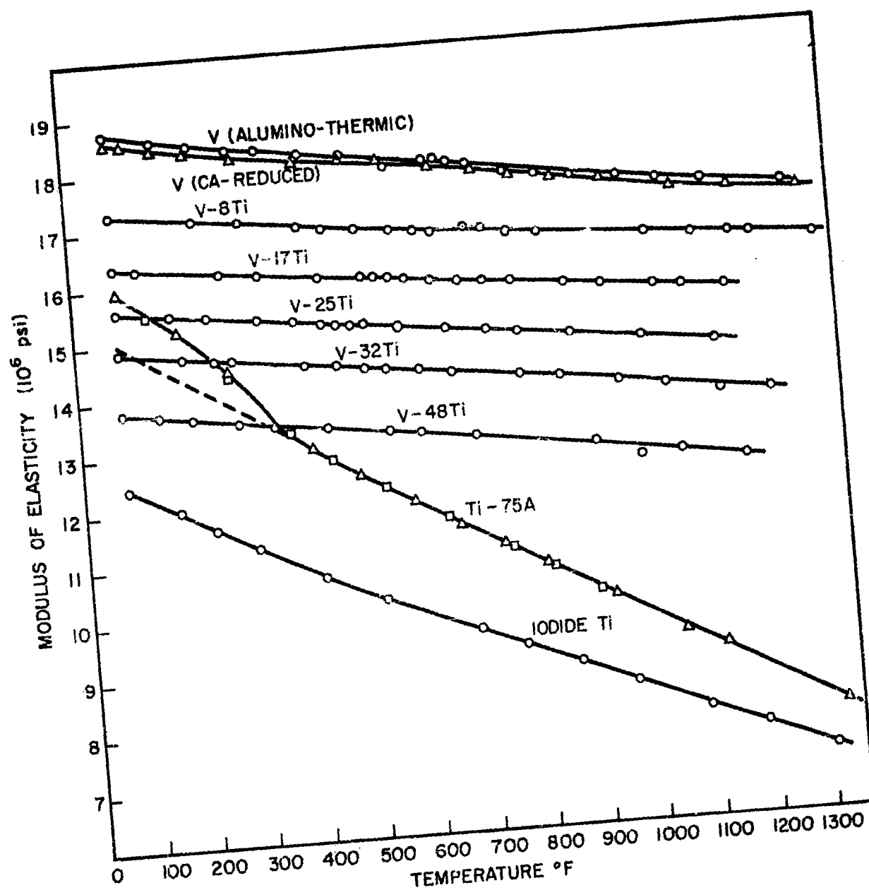
FIG. 9.9 MODULUS OF ELASTICITY OF VANADIUM, TITANIUM AND V-Ti ALLOYS FROM 70-1300°F 7
