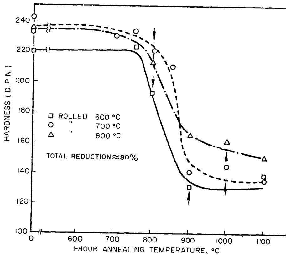
FIG. 3.7 HARDNESS OF IODIDE CHROMIUM VS ANNEALING TEMPERATURE AFTER ROLLING 80% AT 600, 700, AND 800°C 2 (Arrows indicate beginning and end of recrystallization)
