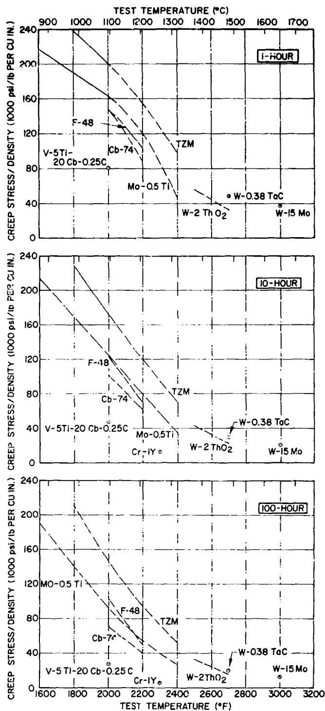
FIG. 2.15 CREEP STRESS-DENSITY RATIO FOR 1, 10, and 100 RUPTURE LIFE FOR SELECTED ALLOYS FROM 1600 TO 3000°F
