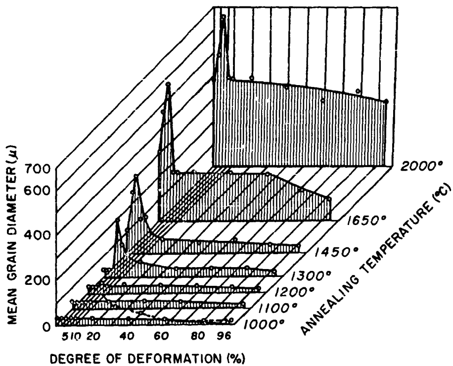
FIG. 4.9 RECRYSTALLIZATION DIAGRAM FOR COLUMBIUM 21
