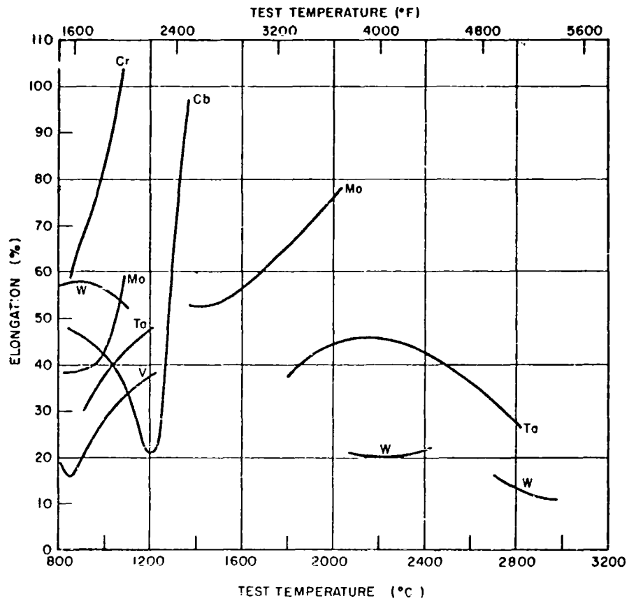
FIG. 2.8 ELONGATION OF SIX REFRACTORY METALS FROM 800 TO 3000 °C
