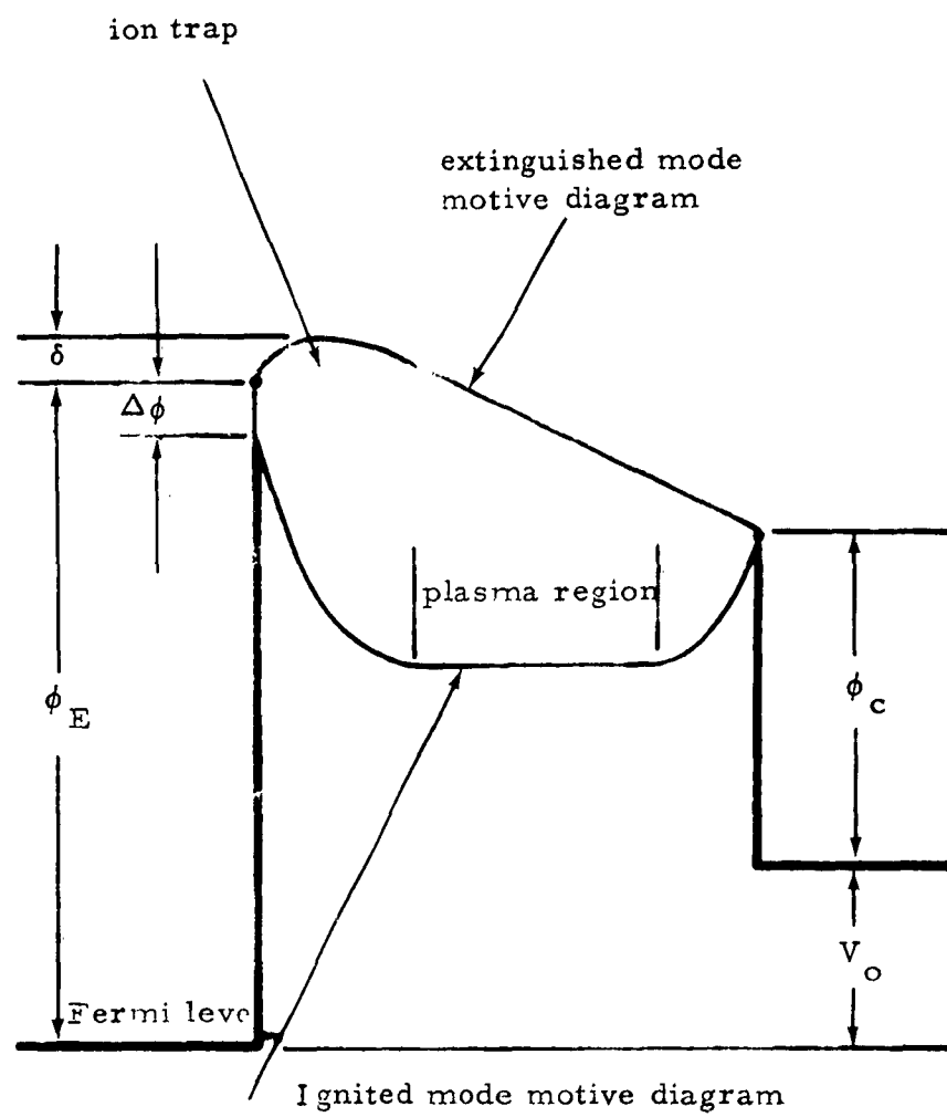
Fig. 3-7. Motive diagram
