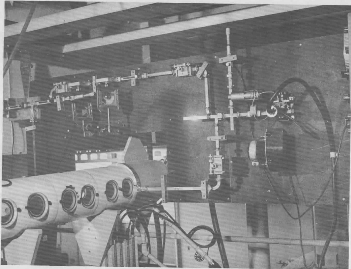
Fig. 3 View Of Plasma Tunnel Showing Microwave Interferometer
