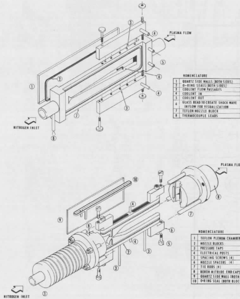
Fig. 4 Details Of Two-Dimensional Nozzle Construction
