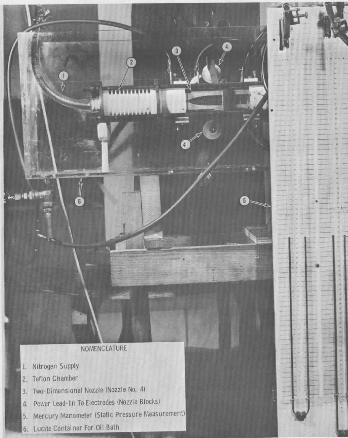
Fig. 6 Petrolatum Oil Bath With Nozzle Blocks In Place
