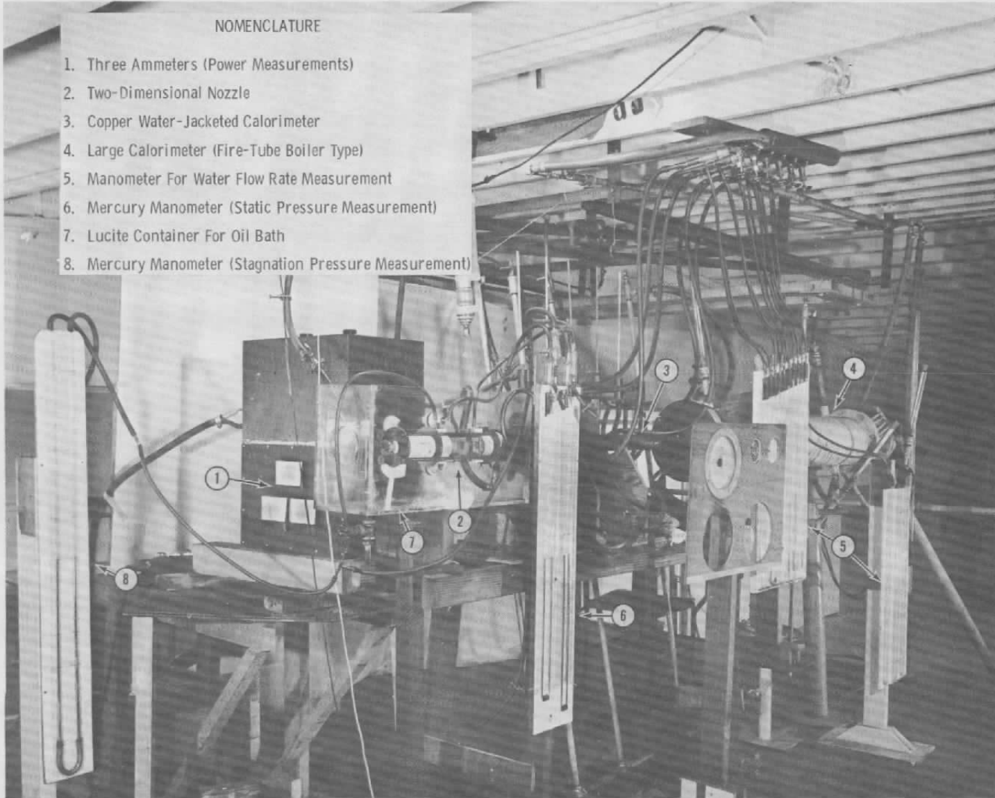
Fig. 7 Two-Dimensional Nozzle RF Heating Apparatus
