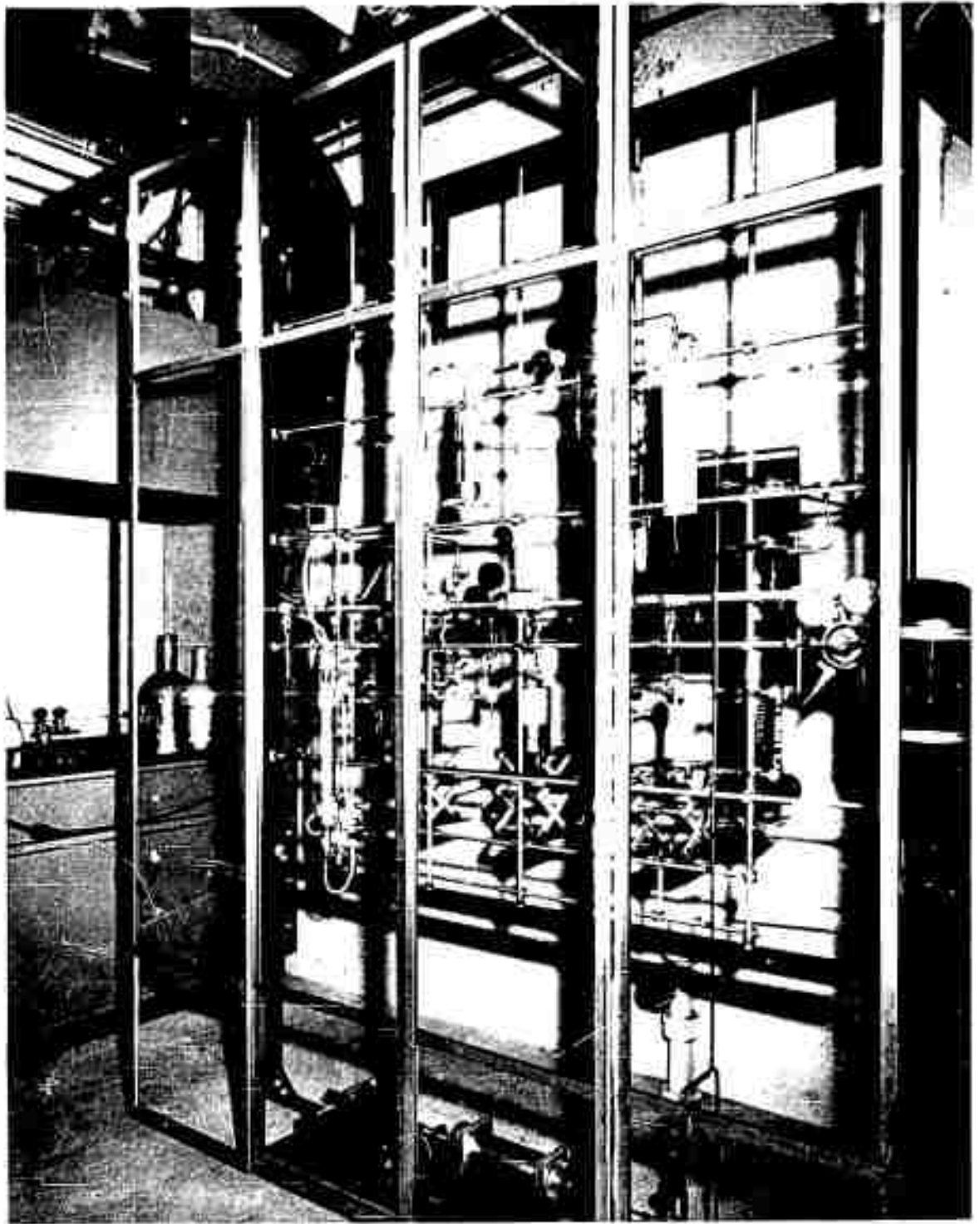
FIGURE 5. APPARATUS FOR SYNTHESIS OF \text{NO}_3\text{F} AND \text{ClO}_4\text{F} MATERIALS
