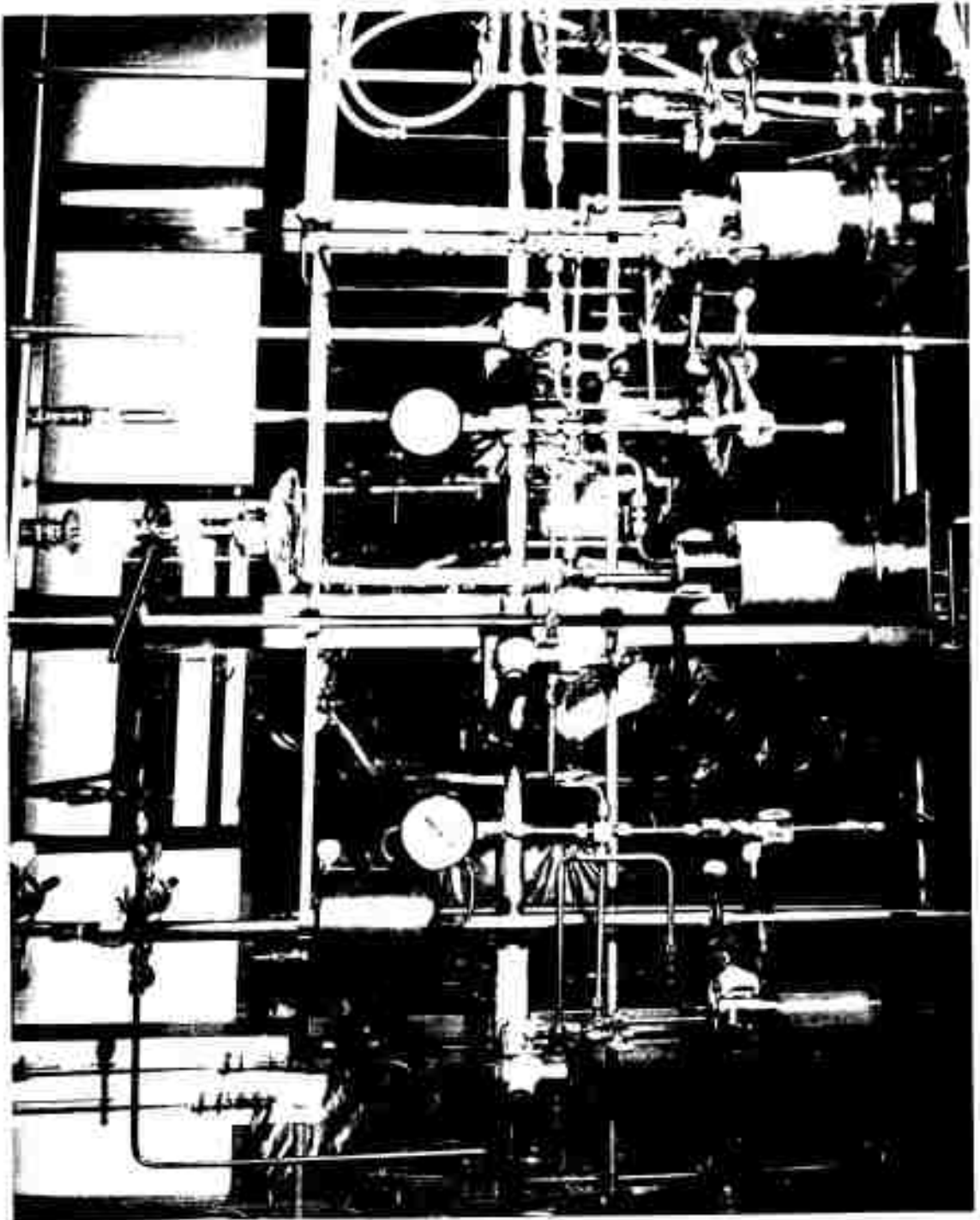
FIGURE 6. CLOSE UP OF ALL APPLS FOR SYNTHESIS OF C_{60} AND C_{70}
