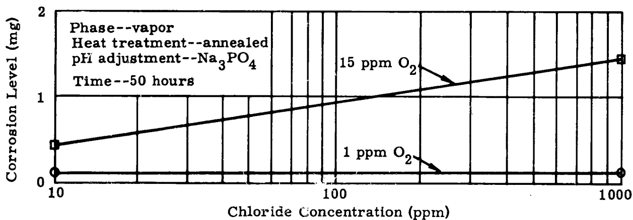
Fig. 18. Corrosion Level Versus Chloride Concentration for Monel
