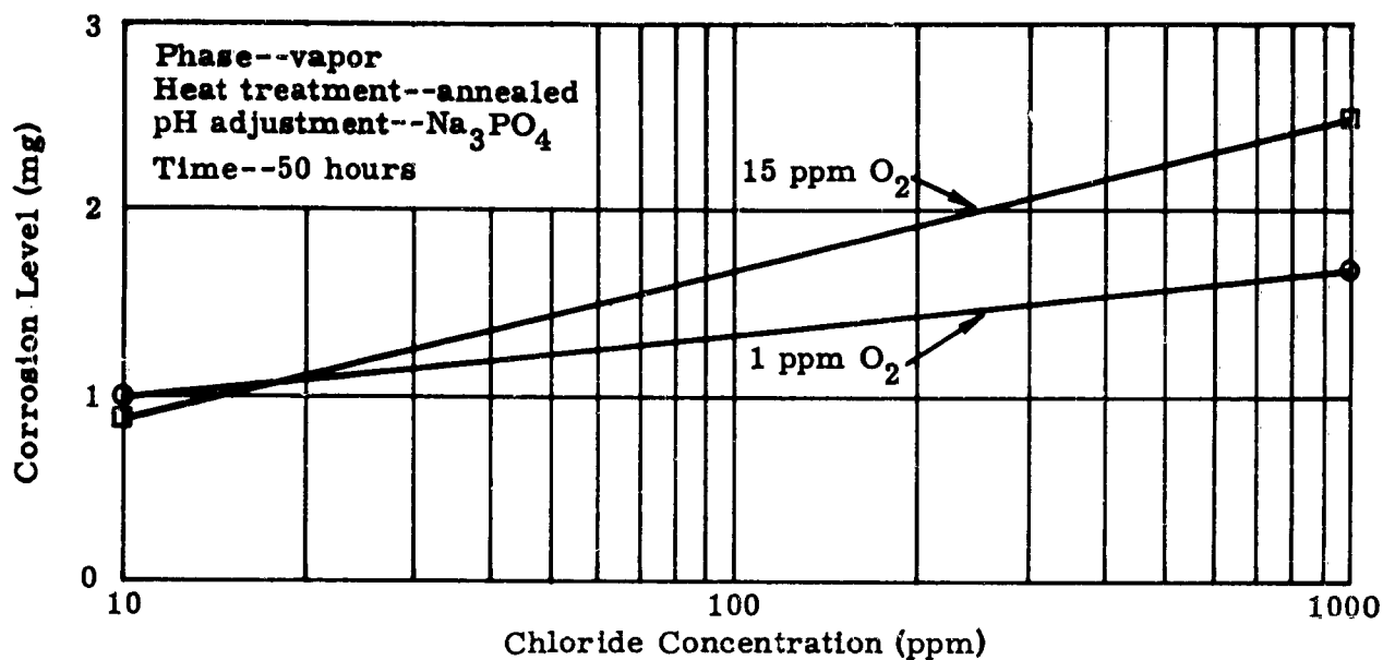
Fig. 17. Corrosion Level Versus Chloride Concentration for Nickel
