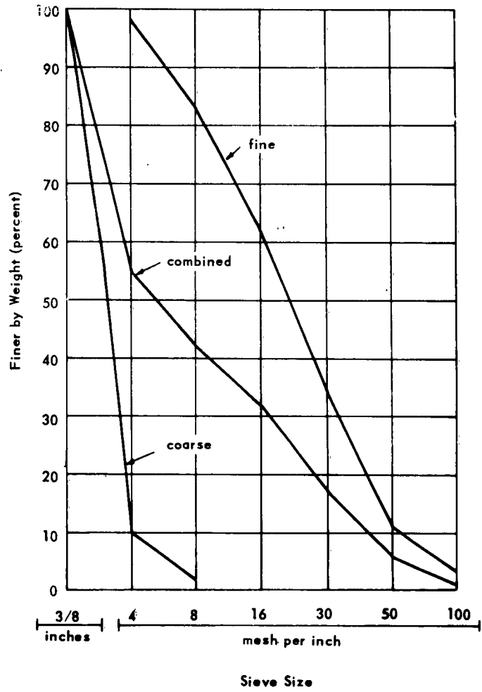
Figure 20. Sieve analysis of aggregates.
