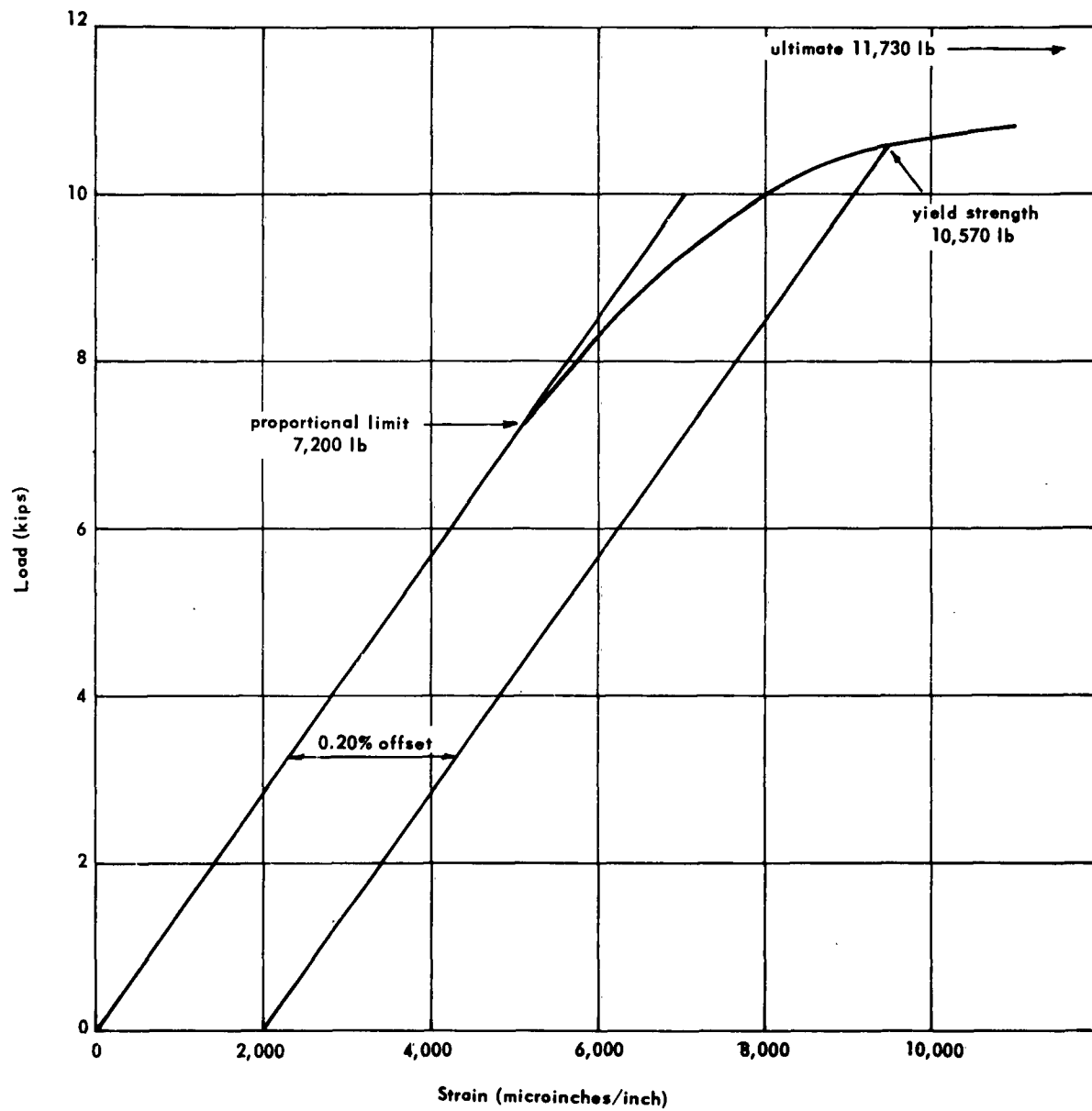
Figure 19. Typical load-strain curve for prestressing wires.
