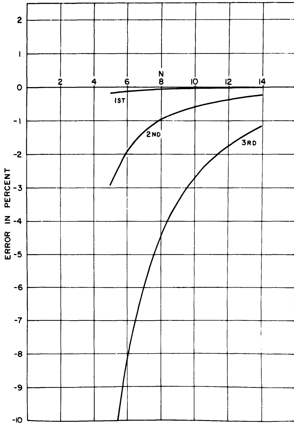
Fig 23. Tapered cantilever, h^2 approximation.
