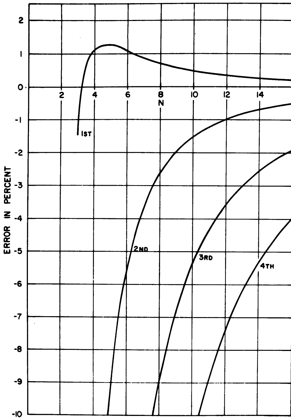
Fig. 13. Built-in, h^2 approximation.
