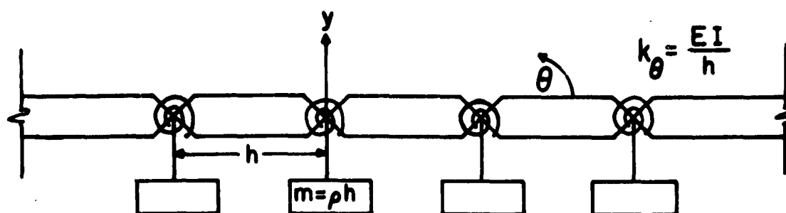
a. Mechanical representation of the simple finite difference approximation to a uniform beam.
