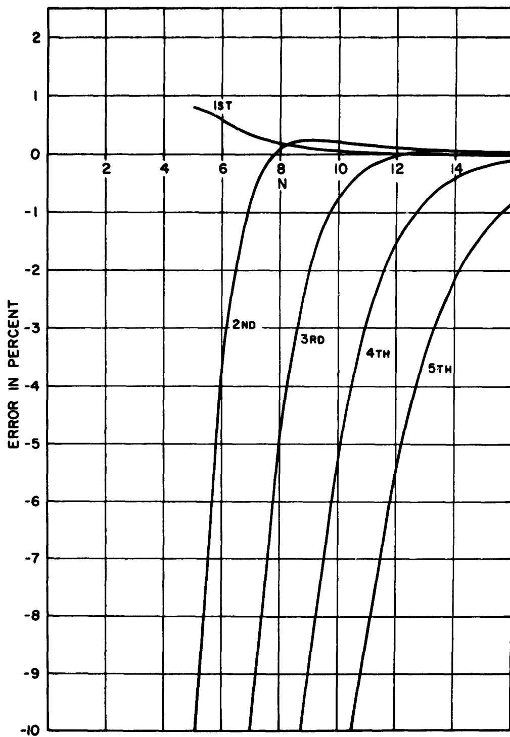
Fig. 15. Built-in, h^4 approximation.
