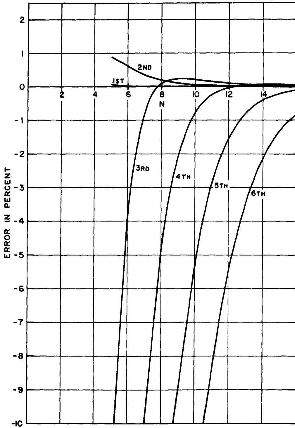
Fig. 16. Cantilever, h^4 approximation.
