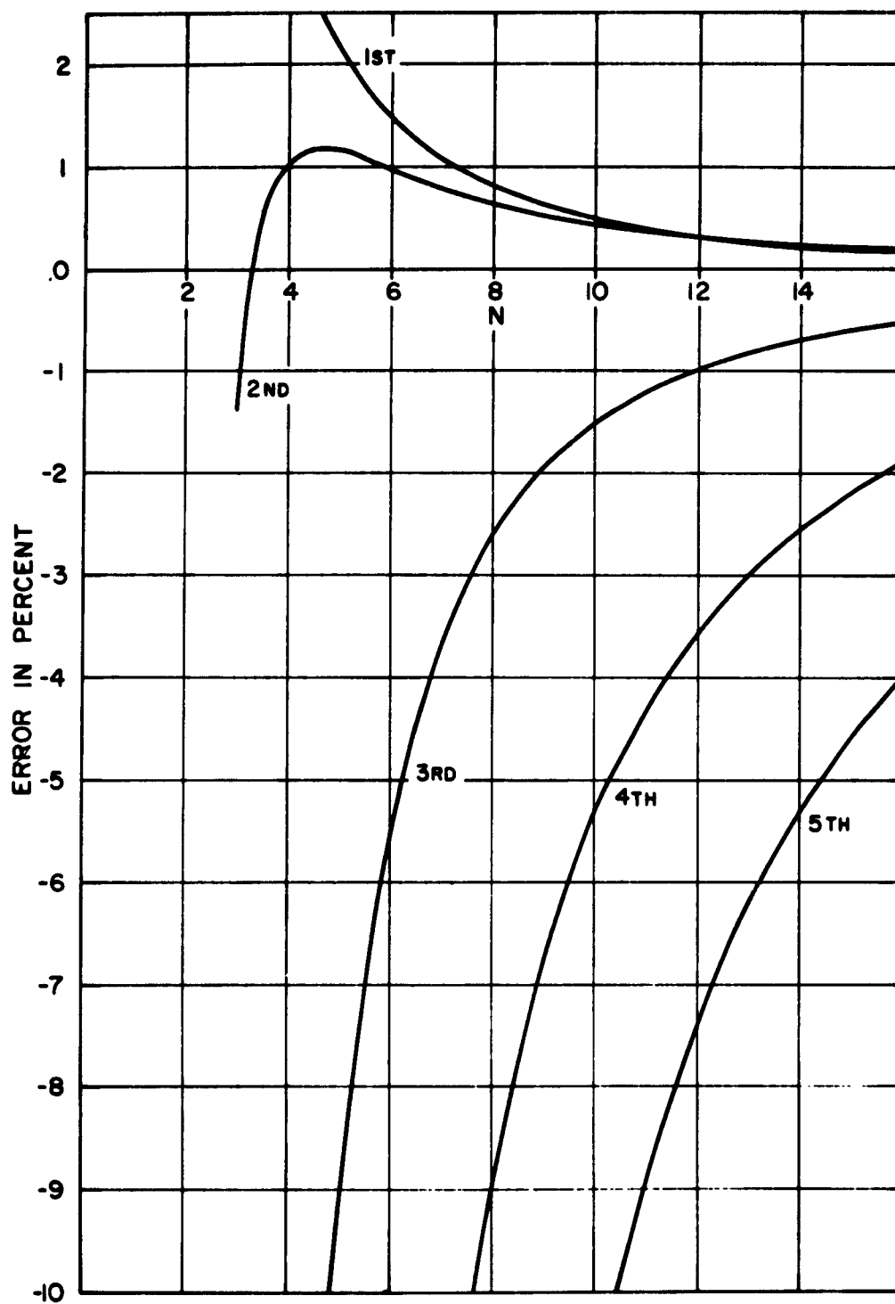
Fig. 14. Cantilever, h^2 approximation.
