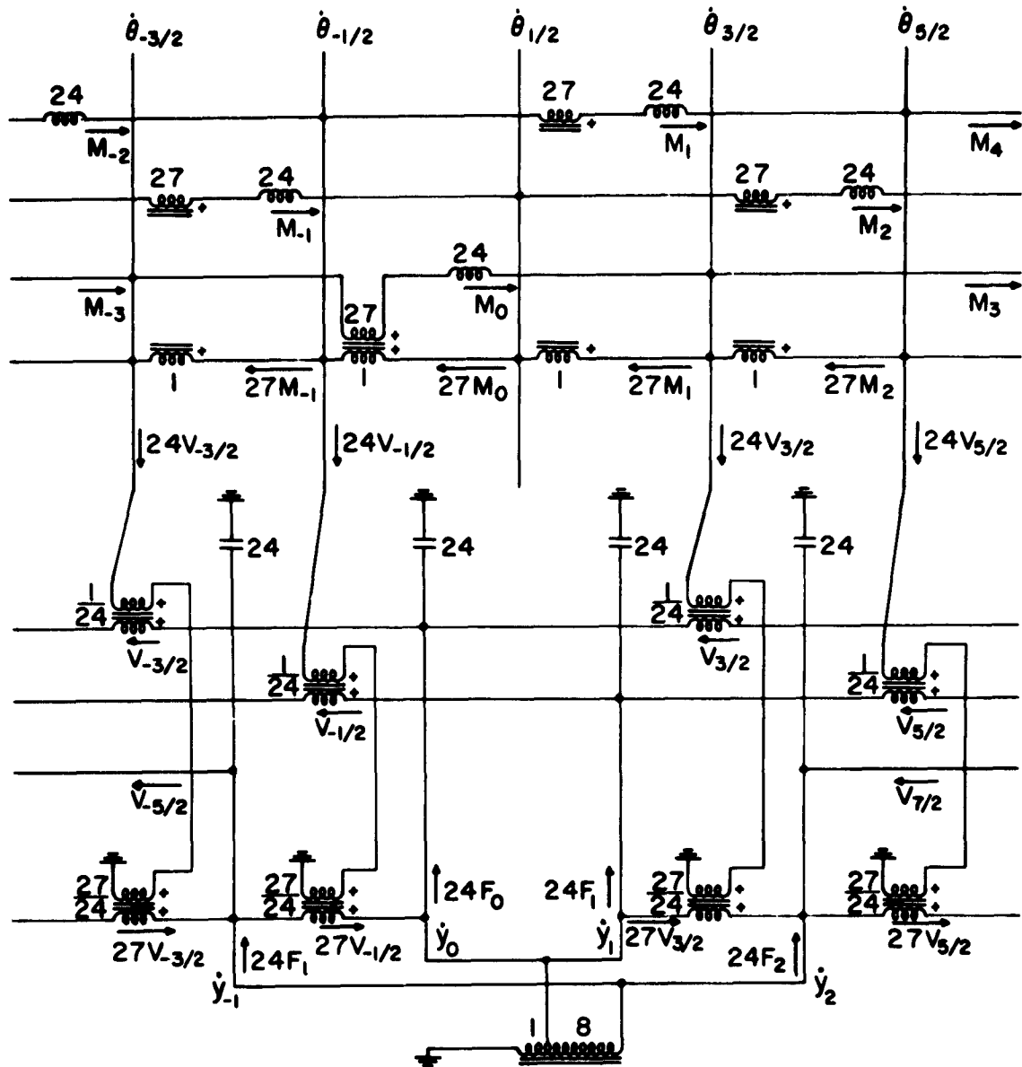
Fig. 12. Passive circuit analogy for a built-in end at station 1/2.
