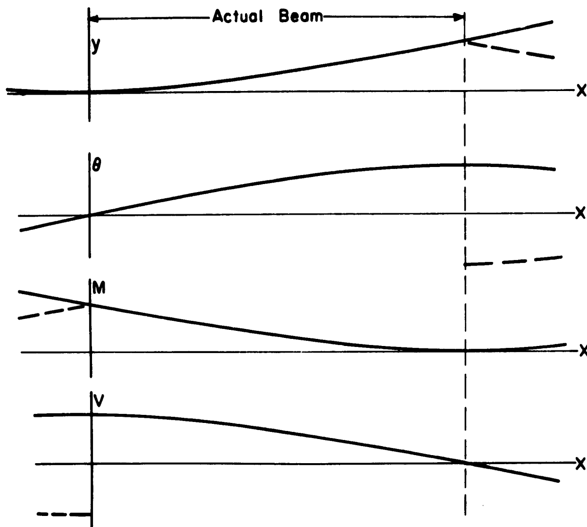
Fig. 10. Symmetry assumptions for a cantilever beam. Solid lines show assumptions used in computations. Dashed lines indicate deviations giving a physically consistent set of assumptions.
