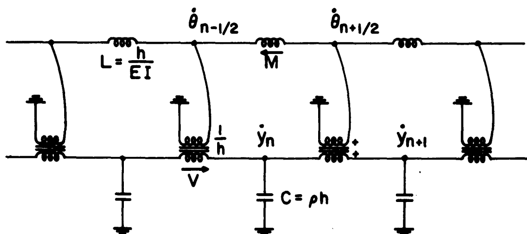
b. Electrical representation of the simple finite difference approximation to a uniform beam.
