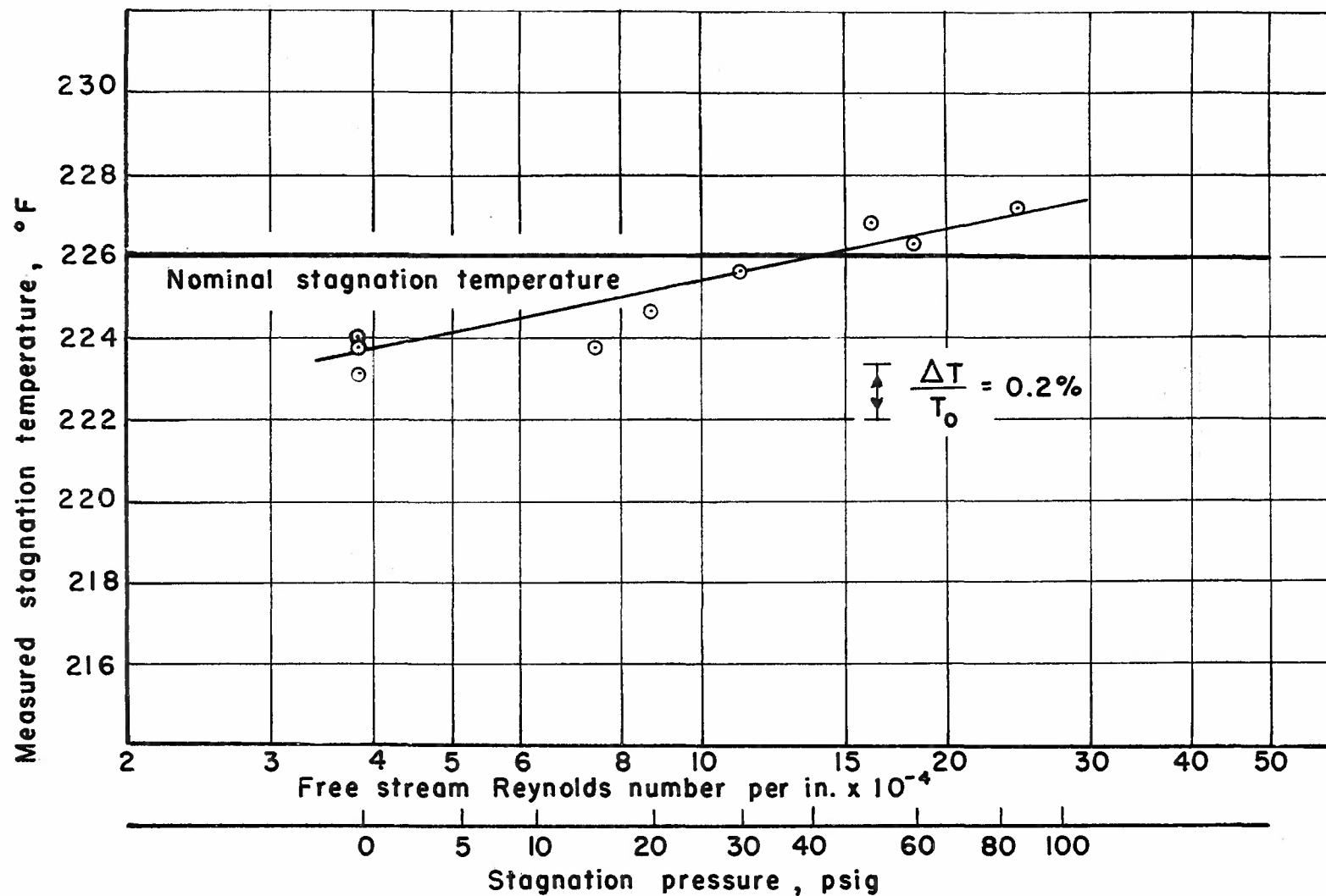
FIG.2 VARIATION OF STAGNATION TEMPERATURE WITH TUNNEL PRESSURE
