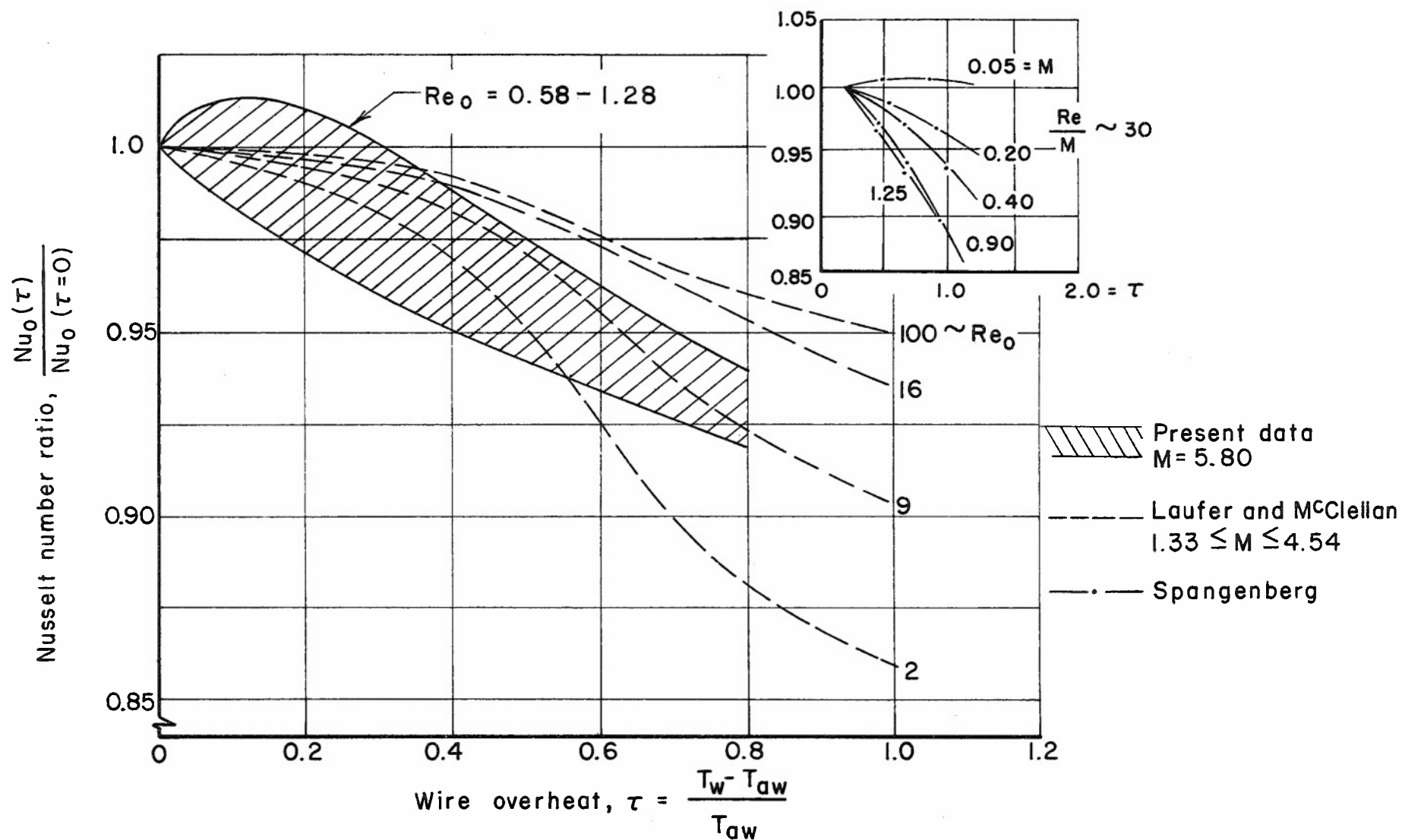
FIG. 16 - VARIATION OF NUSSELT NUMBER WITH OVERHEAT
