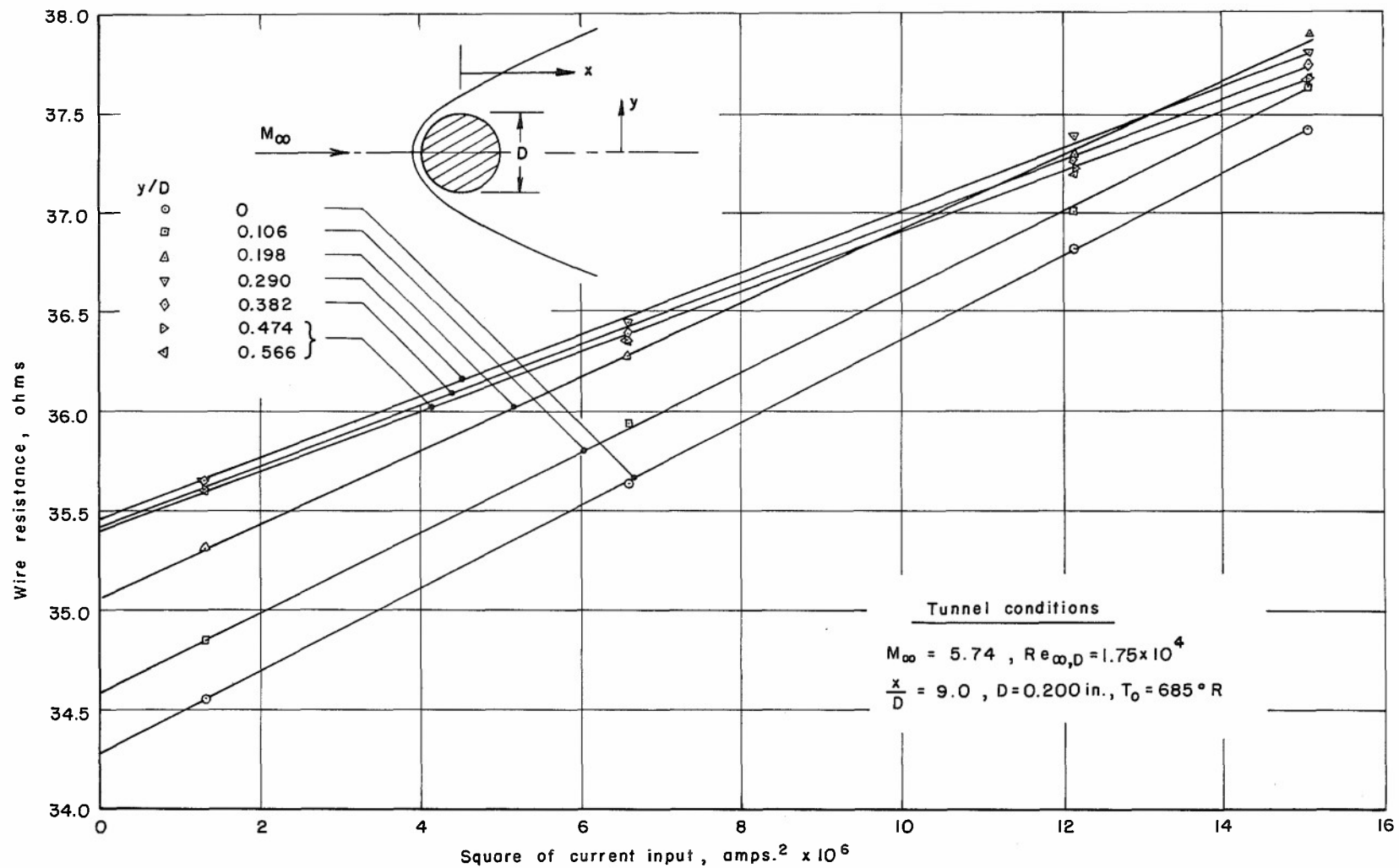
FIG.II - DATA OBTAINED FROM CYLINDER WAKE TRAVERSE
