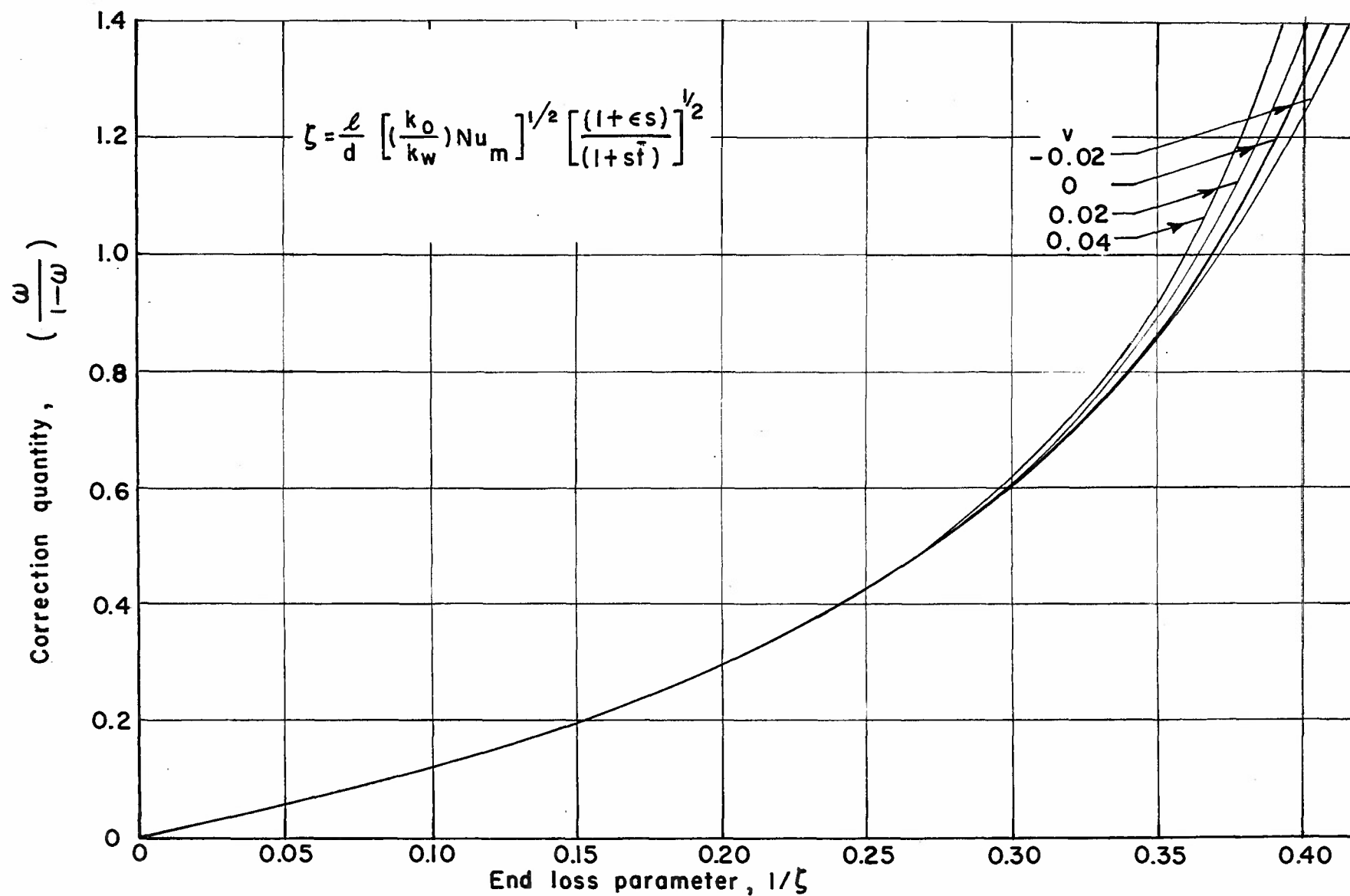
FIG.14 END LOSS RELATIONS FOR RECOVERY TEMPERATURE CORRECTION
