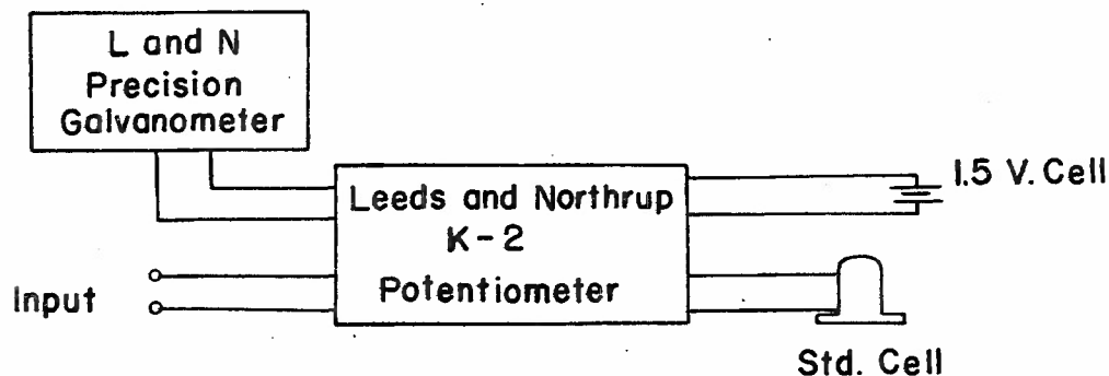
FIG. 6 ELECTRICAL CIRCUIT DIAGRAM
