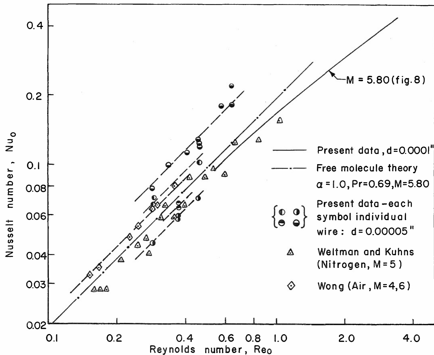
FIG.17 NUSSELT NUMBER-REYNOLDS NUMBER RELATION APPROACHING FREE MOLECULE FLOW
