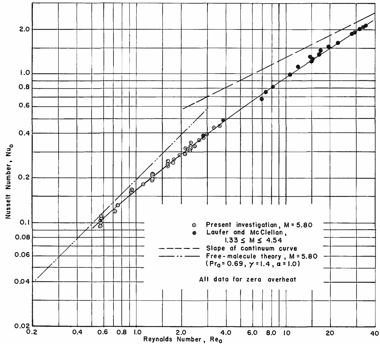
FIG. 8 NUSSELT NUMBER — REYNOLDS NUMBER RELATION FOR SUPERSONIC AND HYPERSONIC FLOW
