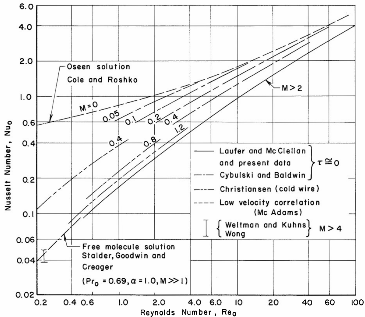
FIG. 7 EMPIRICAL CORRELATION OF HOT-WIRE HEAT TRANSFER AT LOW REYNOLDS NUMBERS
