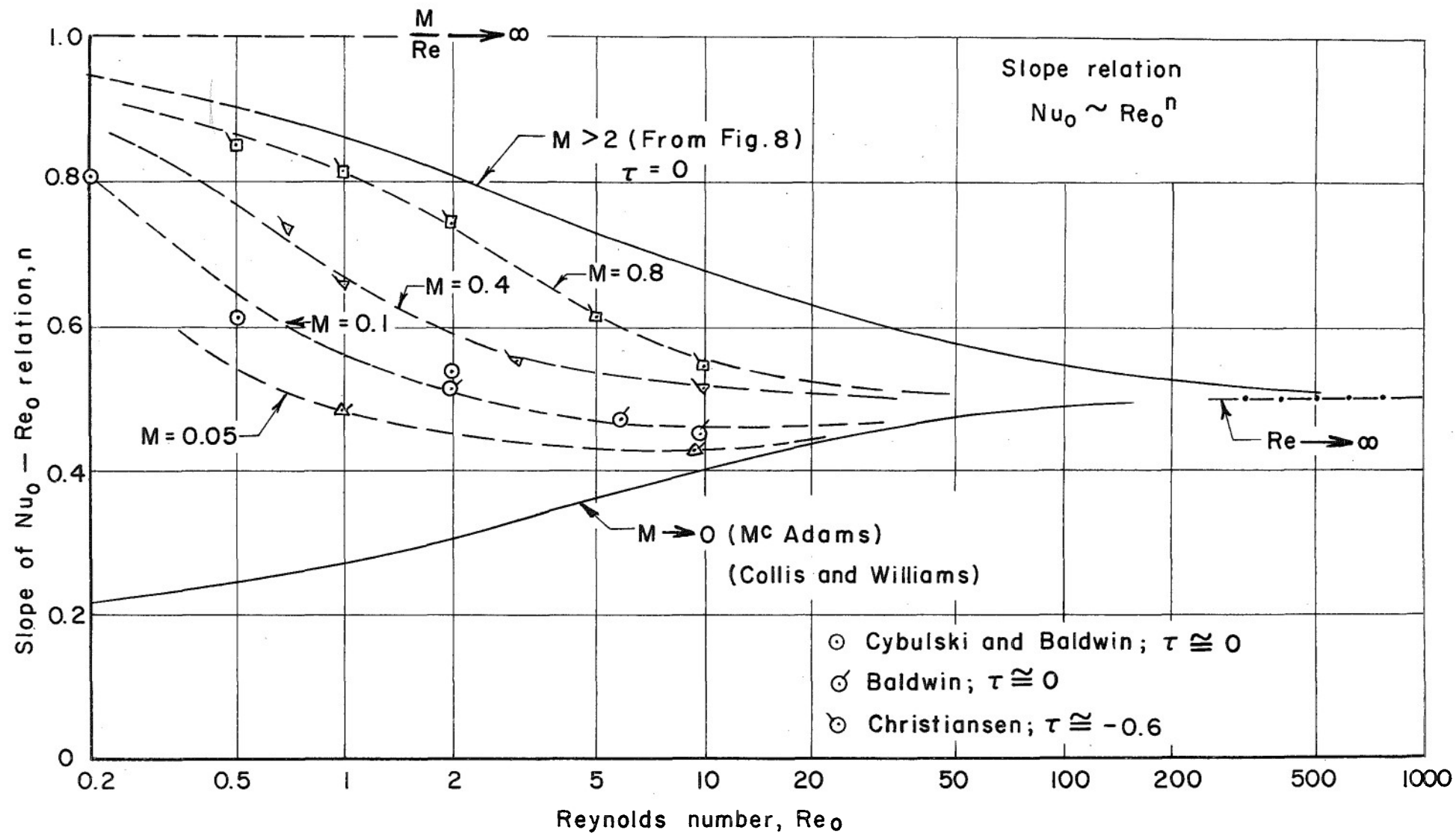
FIG. 9 - SLOPE OF NUSSELT NUMBER-REYNOLDS NUMBER RELATION AS A FUNCTION OF REYNOLDS NUMBER
