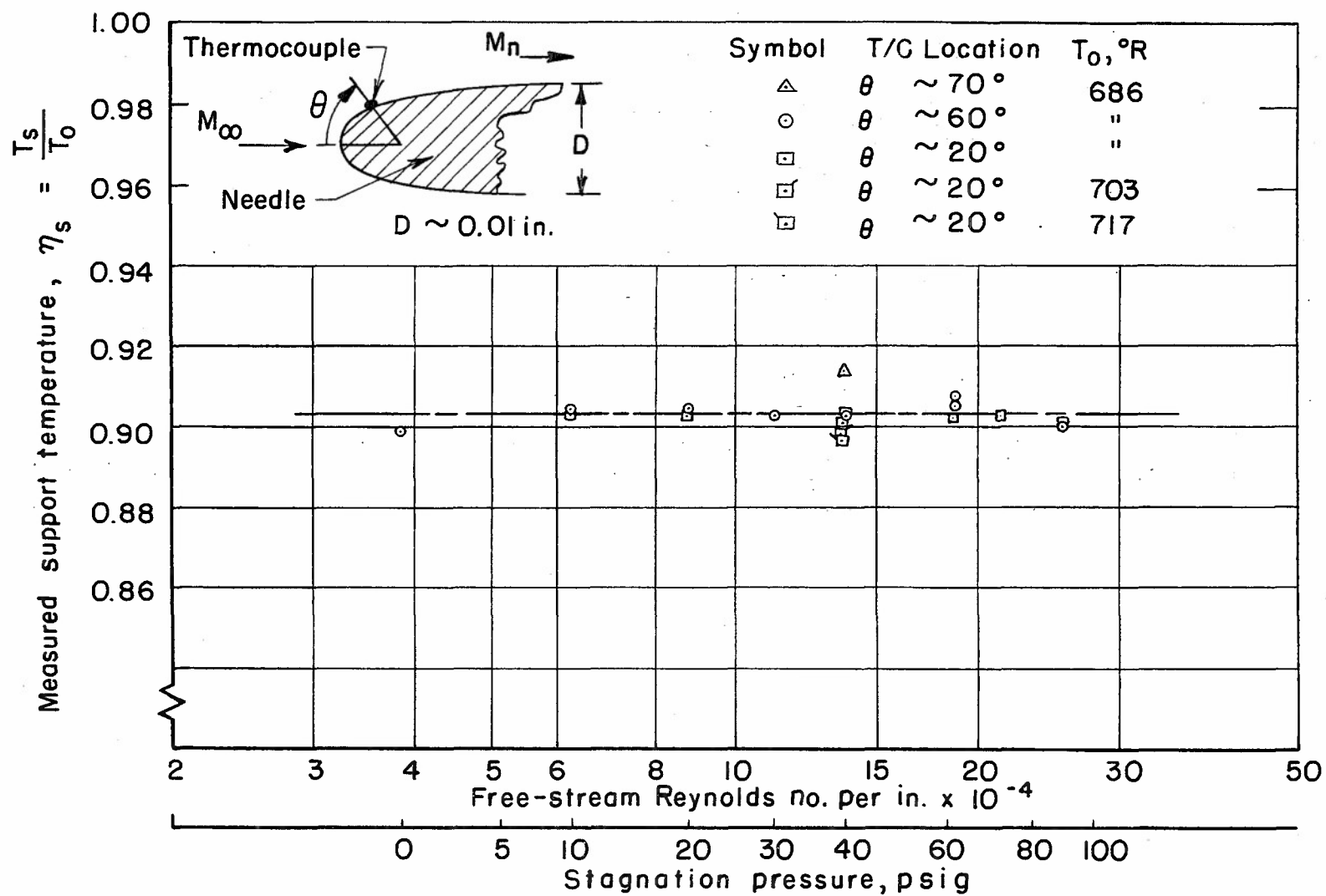
FIG. 15 WIRE SUPPORT TEMPERATURE AS A FUNCTION OF TUNNEL PRESSURE
