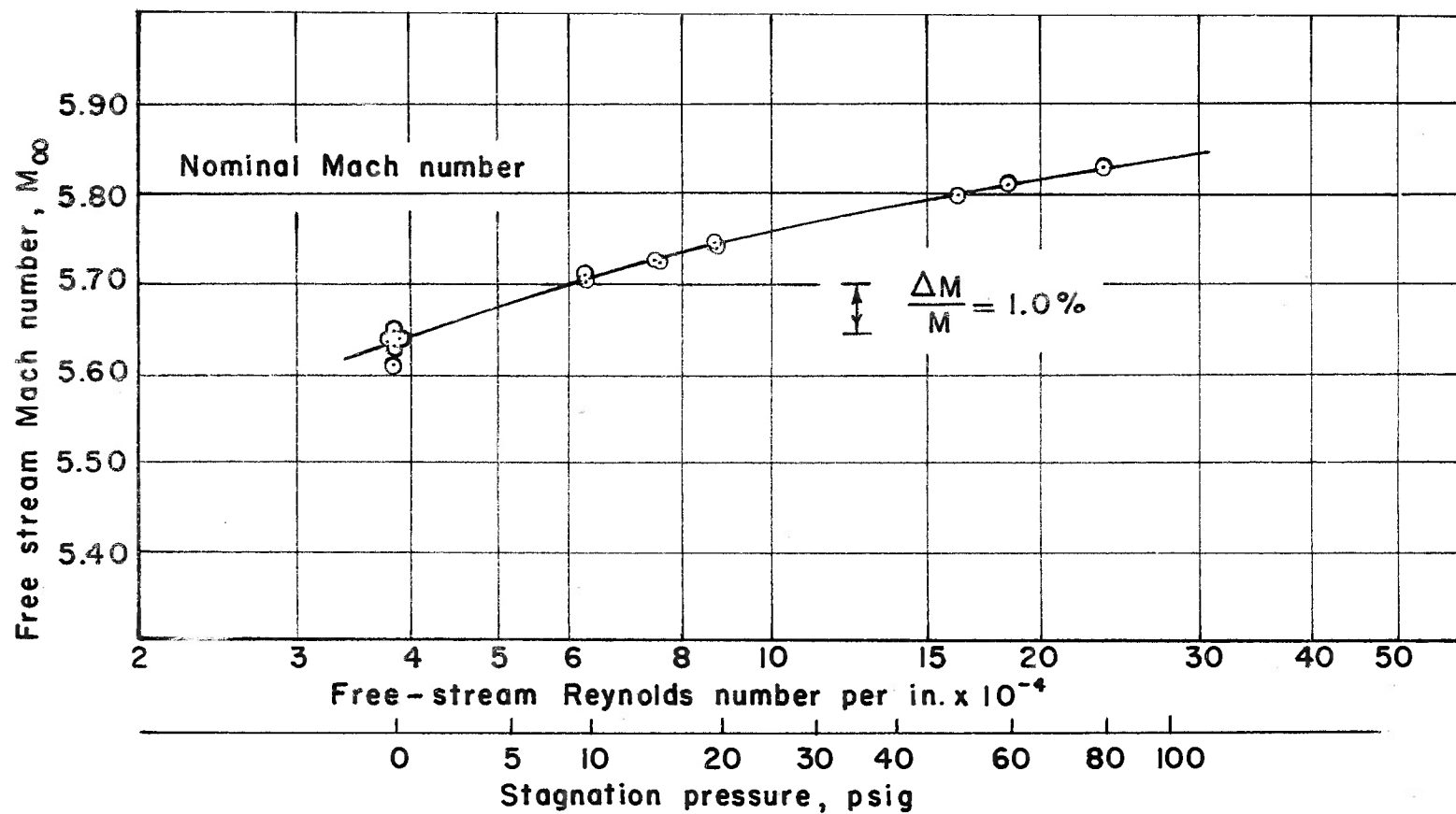
FIG. 1 VARIATION OF FREE STREAM MACH NUMBER WITH TUNNEL PRESSURE
