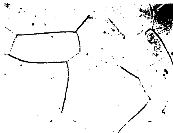
FIG. 1. MICRO-STRUCTURES OF THE STARTING MATERIAL & OF TYPICAL RE-CRYSTALLIZED SPECIMENS. ETCHED 30 SECS. IN 1:1 HF/HNO 3 . 200 X.
