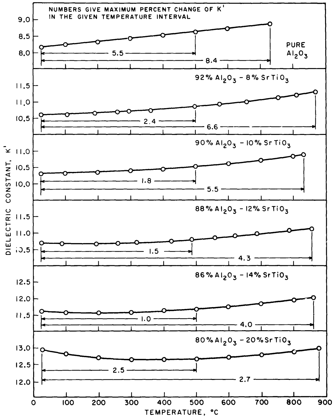
FIG. 1 TEMPERATURE VARIATION OF K' AT 4 \times 10^9 C/S FOR Al_2O_3 - SrTiO_3 COMPOSITIONS.
