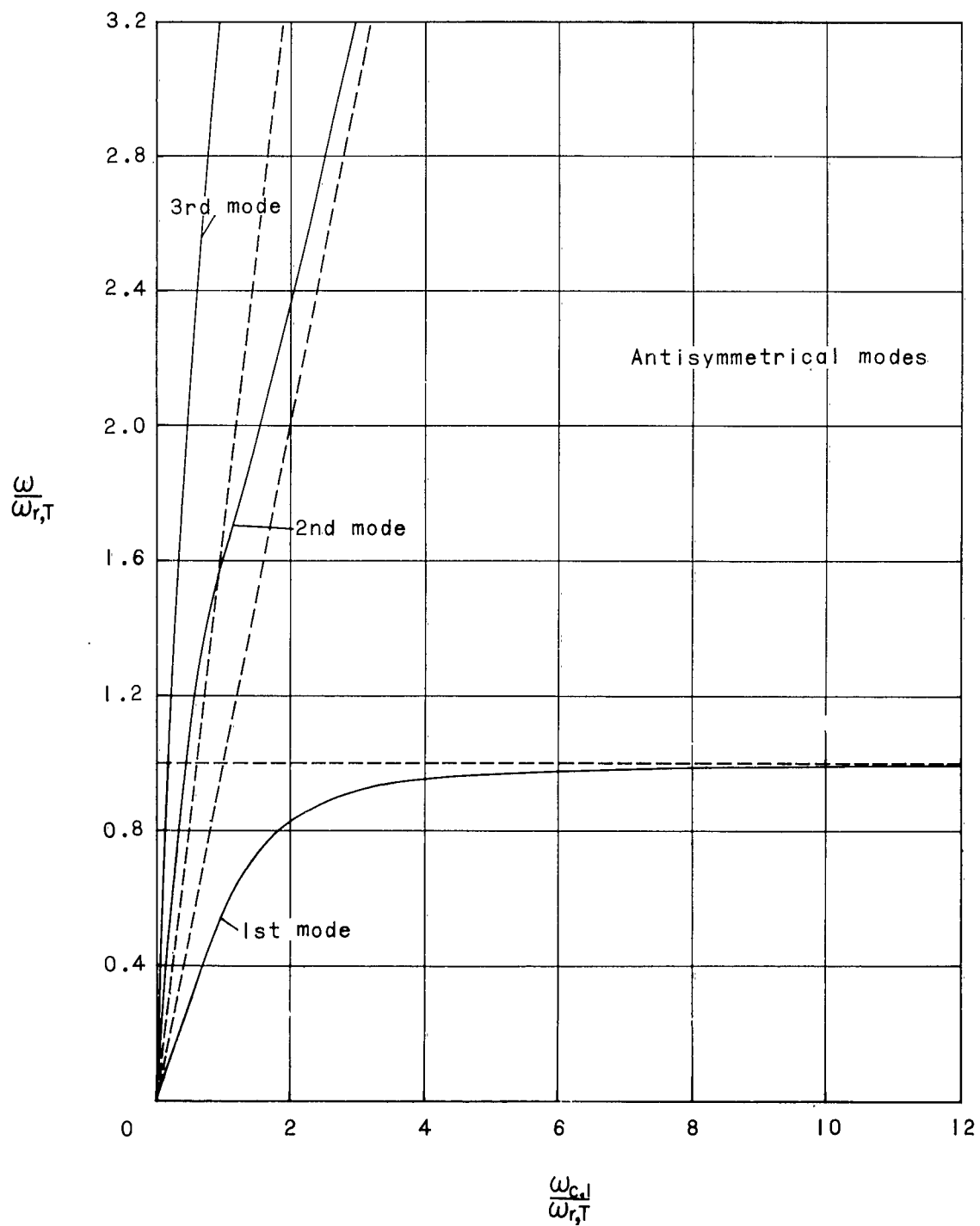
Figure 8.- Variation of \omega/\omega_{r,T} with \omega_{c,1}/\omega_{r,T} for antisymmetrical modes.
