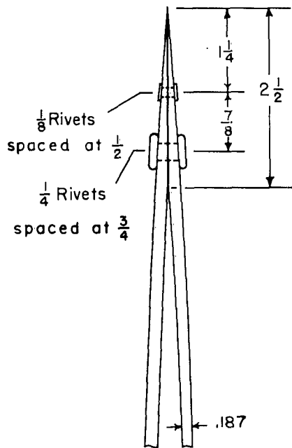
Detail A-Beam 1
