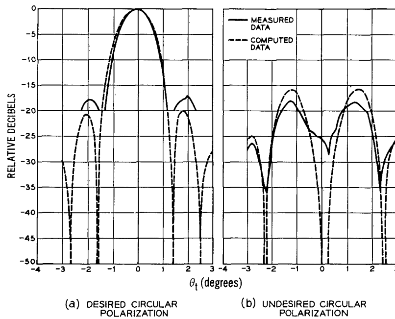
Figure 8 – Circularly polarized radiation patterns in the transverse plane (2390 Mc)
