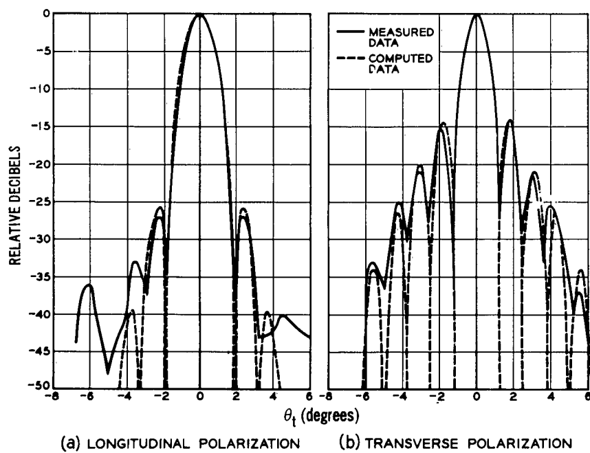
Figure 5 — Principal radiation patterns in the transverse plane (2390 Mc)
