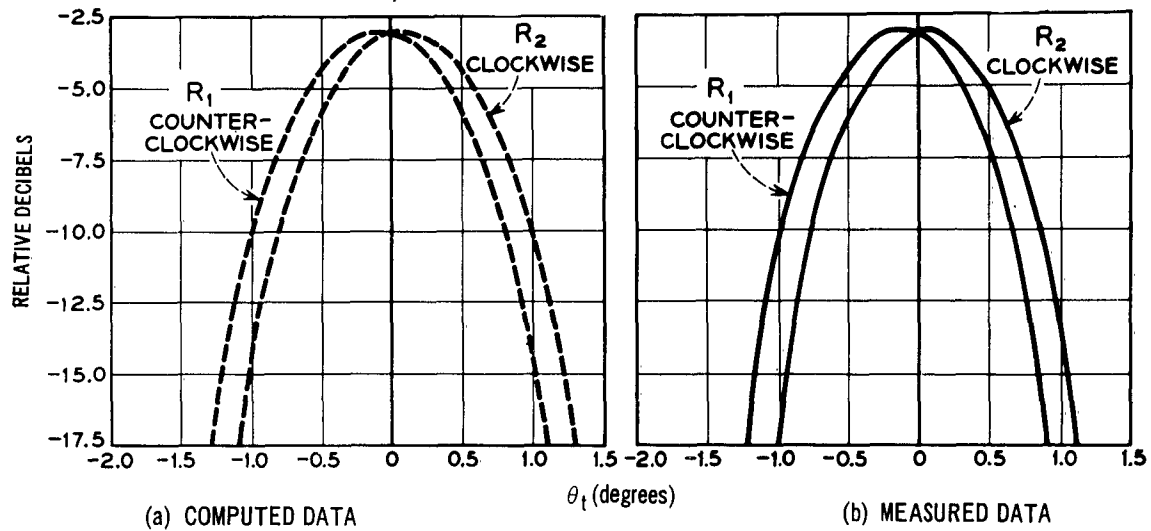
Figure 9 — Circularly polarized radiation patterns in the transverse plane, showing dependence of beam displacement on sense of polarization
