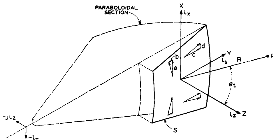
Figure B1 —Aperture field components for calculation of circular polarization; distant point, P, is the transverse plane
