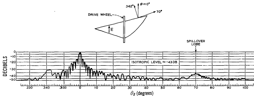
Figure 11 — Extended radiation pattern; longitudinal plane, longitudinal polarization
