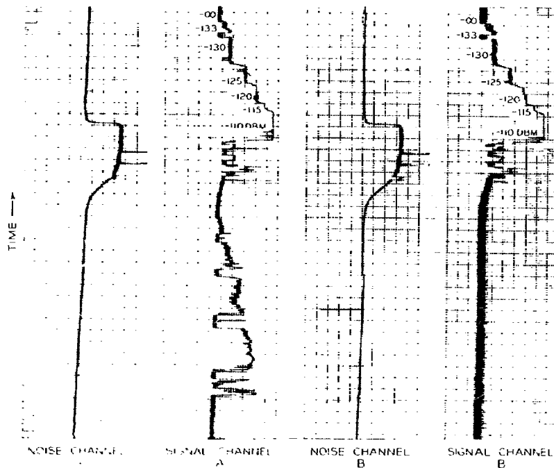
Figure 14—Recording of signal levels received by the parametric amplifier system from Goldstone Lake, pass 93
