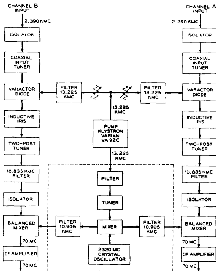
Figure 2—The parametric amplifier system
