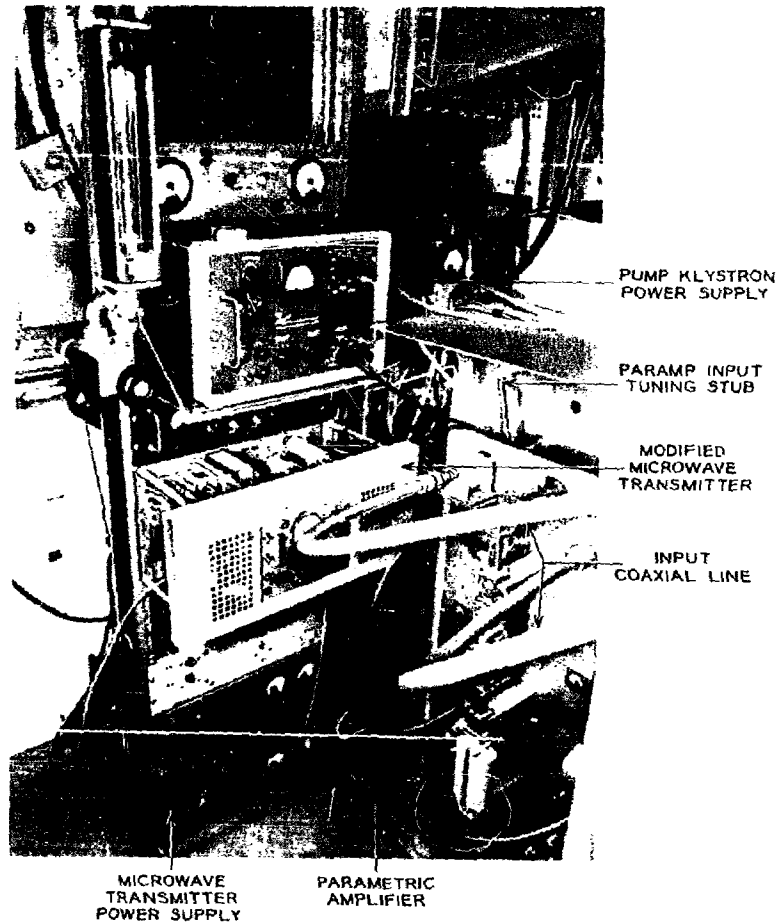
Figure 12—Parametric amplifier coaxial input lines, power supply mountings, and microwave transmitter
