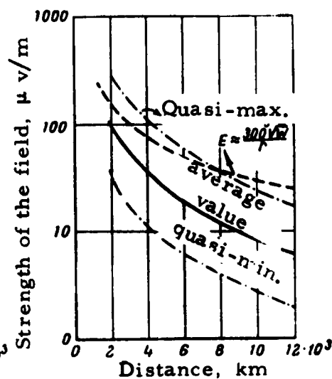
Fig 236 - Averaged results of measurements of field strength showing dependence with distance and range (diapasone) 12.5 - 30 kc/s (solid line).
