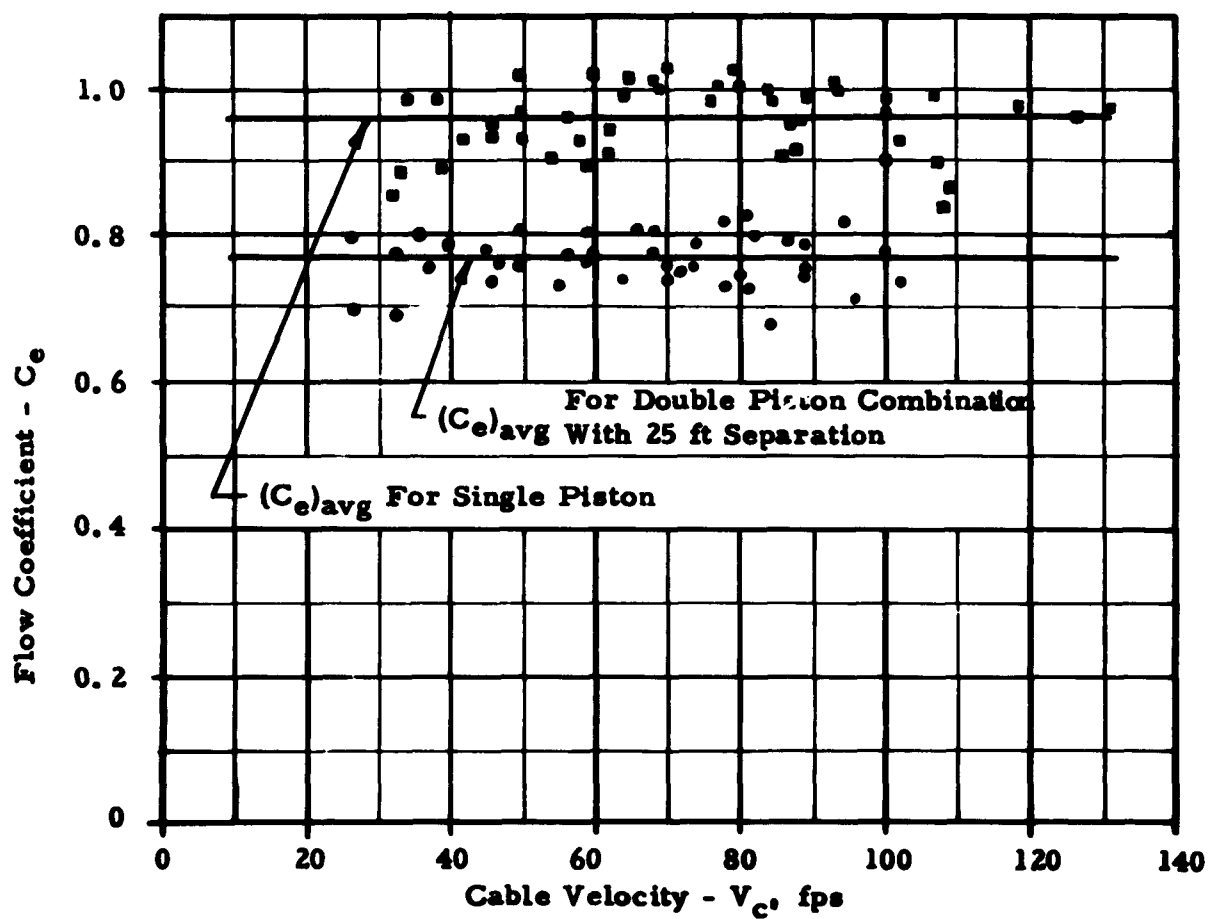
FIGURE 21: CALCULATED FLOW COEFFICIENT VERSUS CABLE VELOCITY FOR SINGLE AND DOUBLE PISTON
