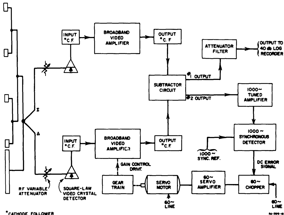
FIG. 15 BLOCK DIAGRAM OF RECEIVER WITH SIMPLE ELECTROMECHANICAL SERVO LOOP ADDED TO IT FOR CHANNEL SIGNAL BALANCING
