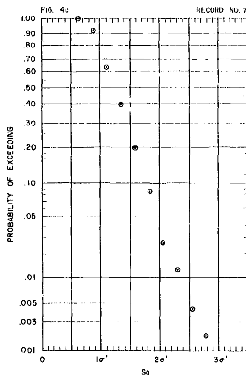
FIGURE 4 PROBABILITY INTEGRAL OF ALTERNATING STRESS PEAKS
