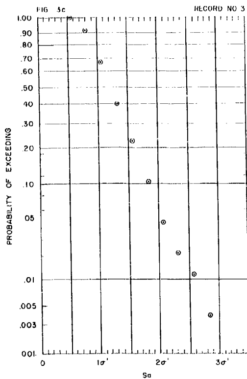
FIGURE 3 PROBABILITY INTEGRAL OF ALTERNATING STRESS PEAKS
