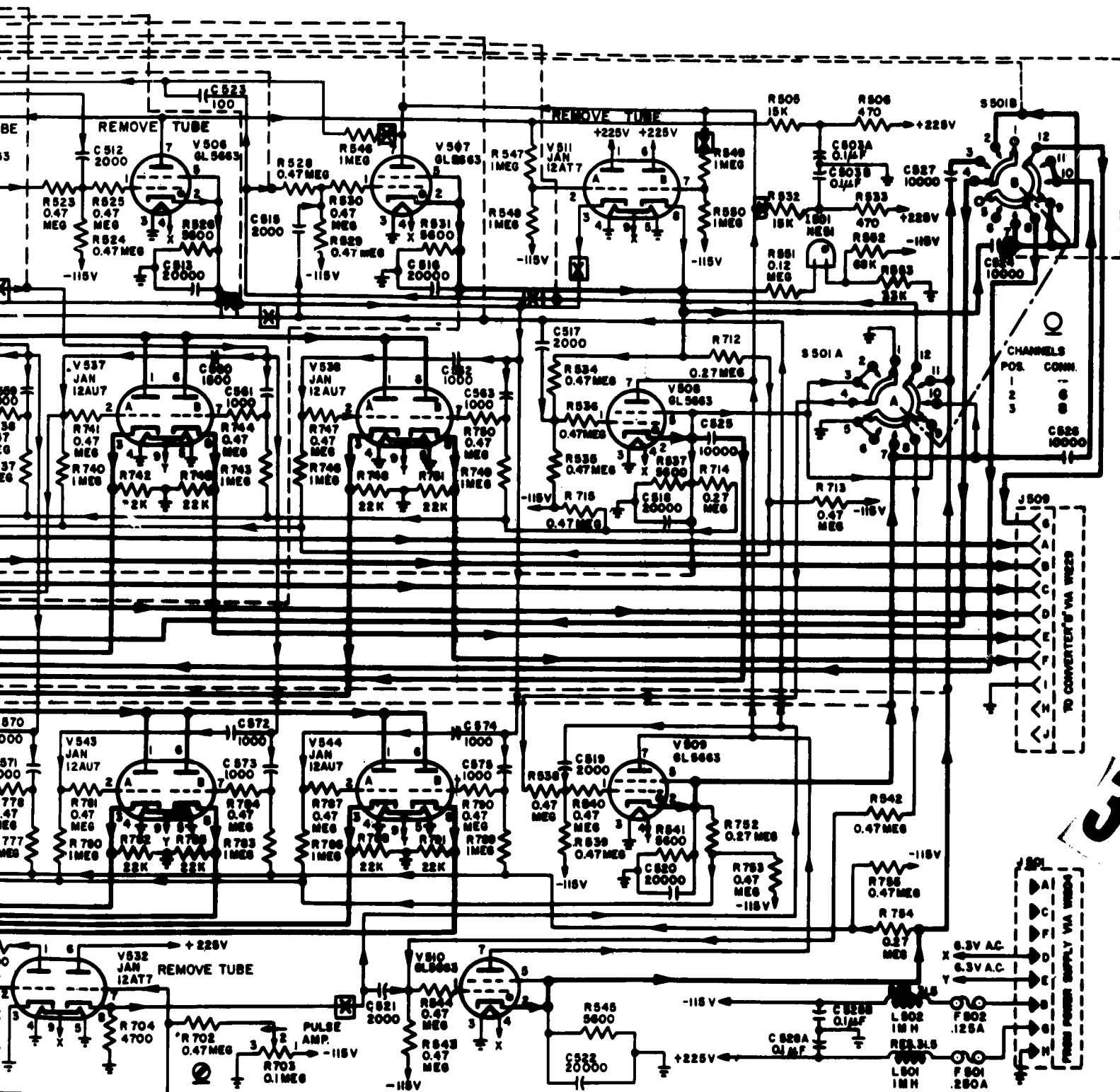
Figure 2-41. Receiving Signal Distributor TT-64/FGC-5, Unit No. 2, Modified Schematic Diagram For 8-Channel Operation
