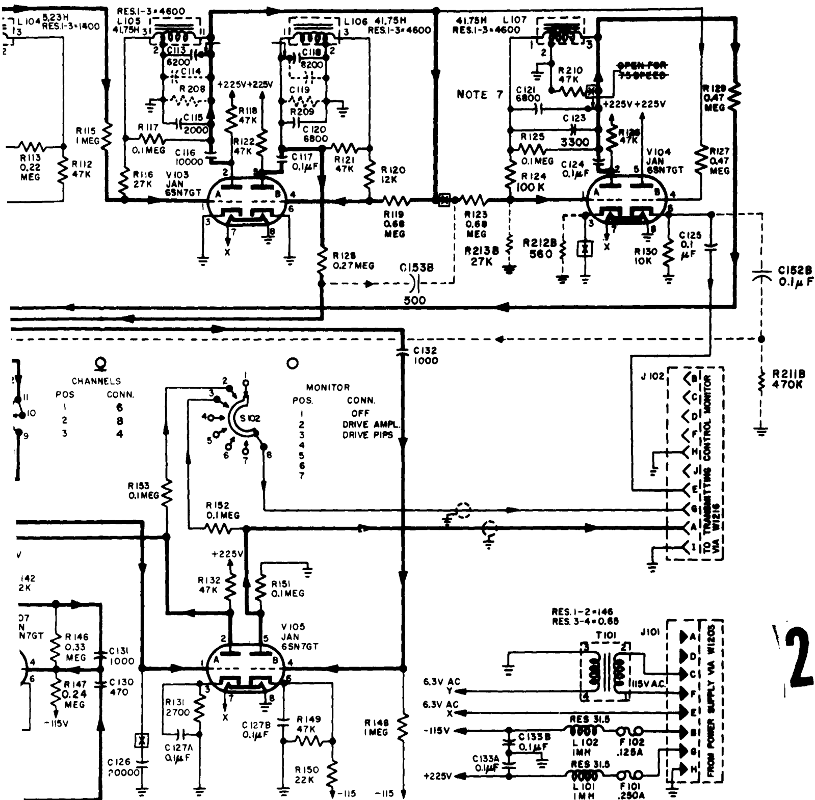
Figure 2-42. Transmitting Signal Distributor Drive O-101/FGC-5, Unit No. 1, Modified Schematic Diagram For 8-Channel Operation
