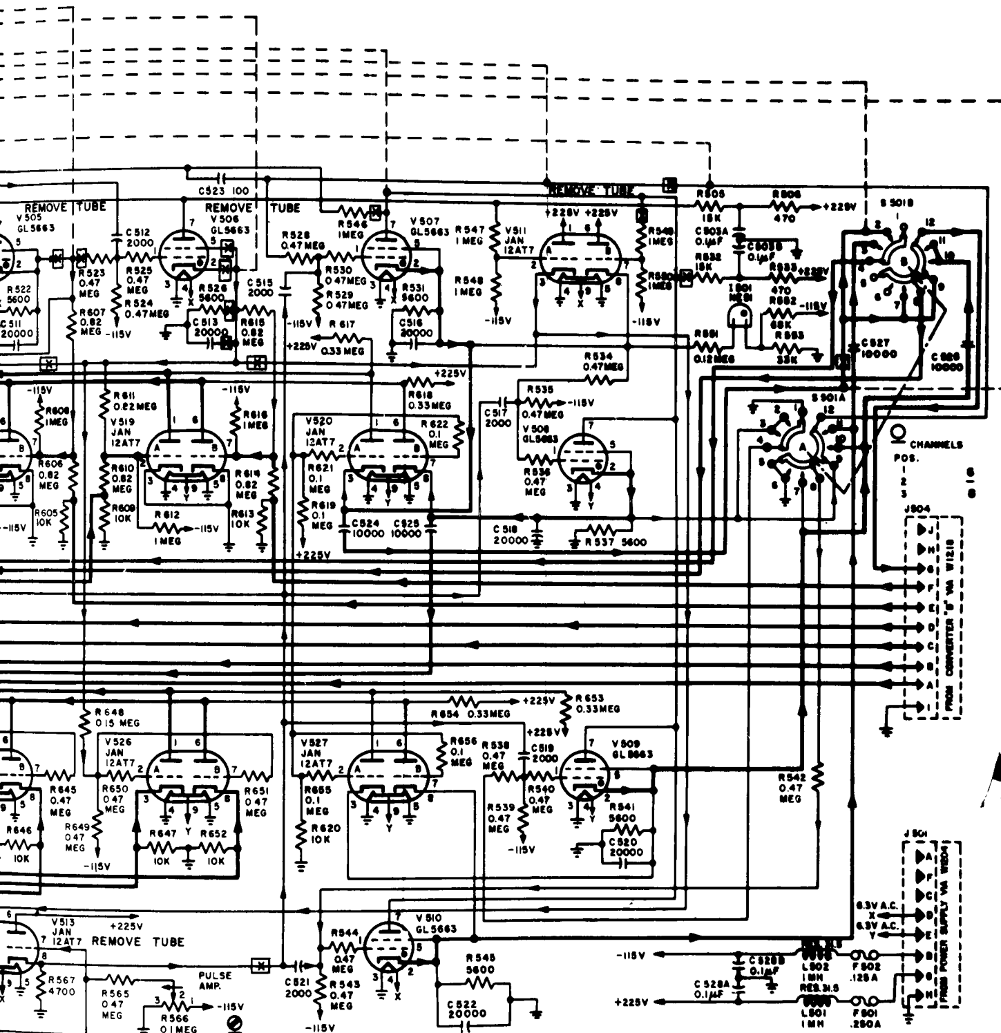
Figure 2-39. Transmitting Signal Distributor TT-58/FGC-5, Unit No. 2, Modified Schematic Diagram For 8-Channel Operation
