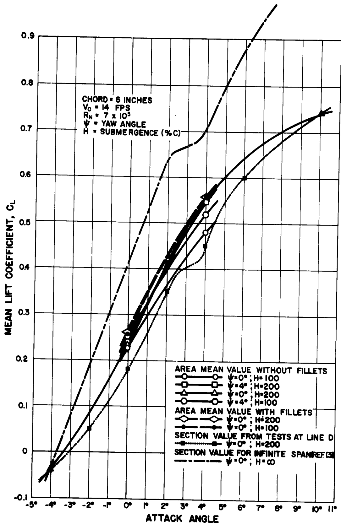
Fig. 8 - Mean Pressure Lift Coefficients of Foli 16-509 for the Area (Span = 2/3 Chord) Adjacent to a Center Strut 16-012
