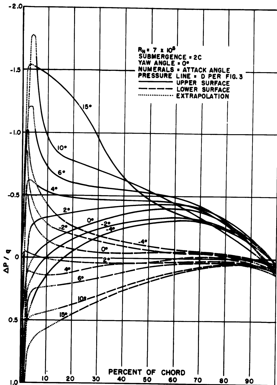
Fig. 10 - Pressure Profiles for Foil 16-509 at Tap Line D
