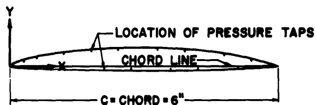
FOIL SECTION—NACA 16-509
