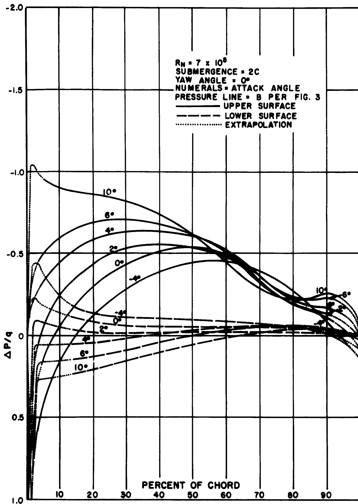
Fig. 11 - Pressure Profiles for Foil 16-509 Adjacent to an End Strut 16-012 With Fillet
