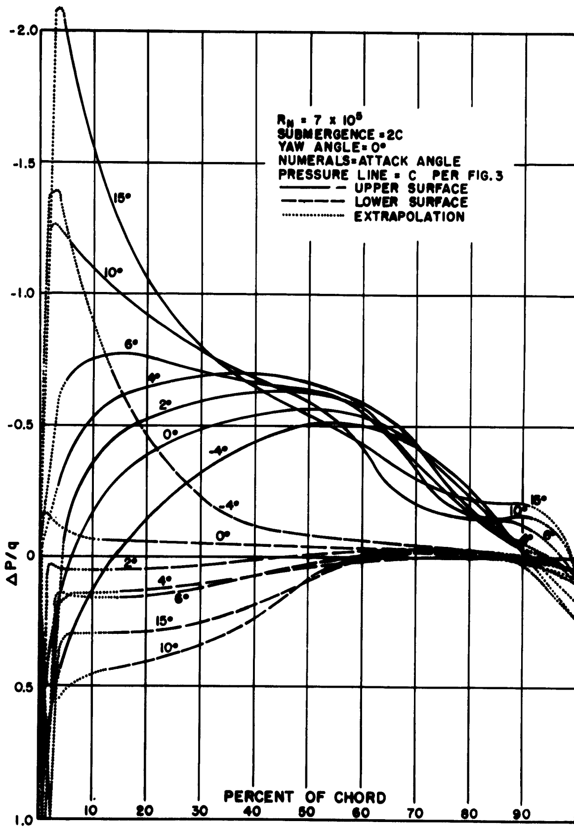
Fig. 12 - Pressure Profiles for Foil 16-509 Adjacent to a Center Strut 16-012 With Filllets
