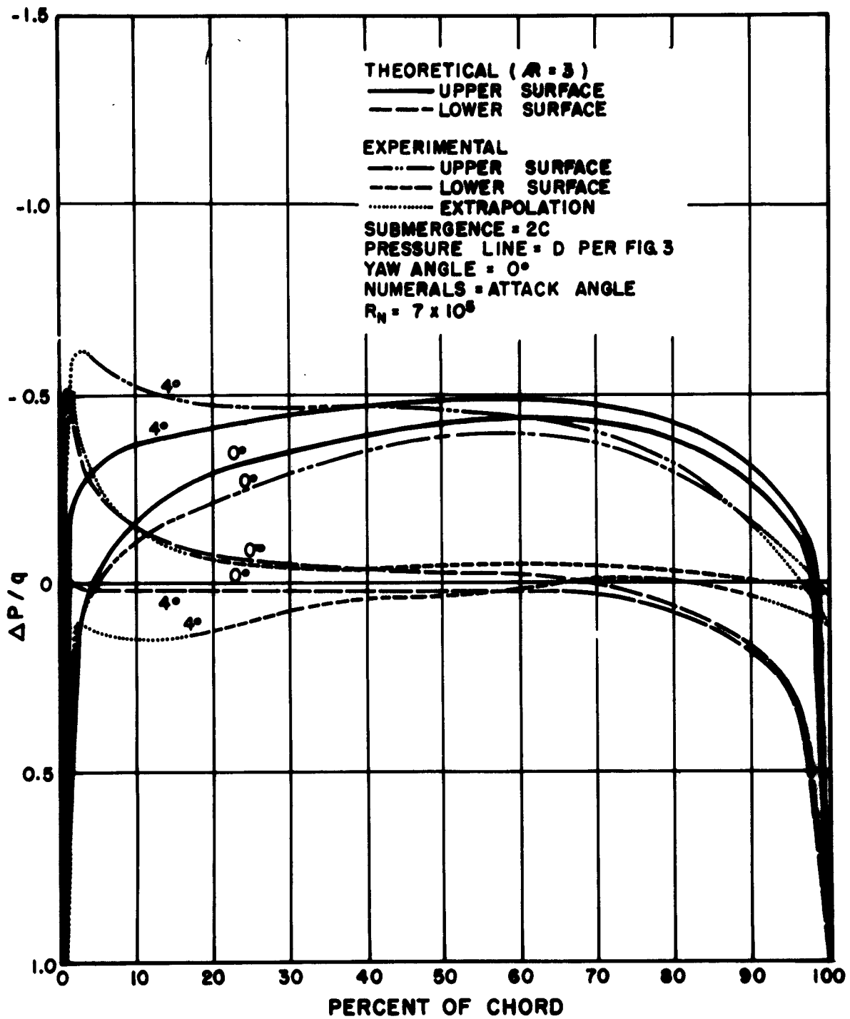
Fig. 15 - Comparative Pressure Profiles for Foil 16-509
