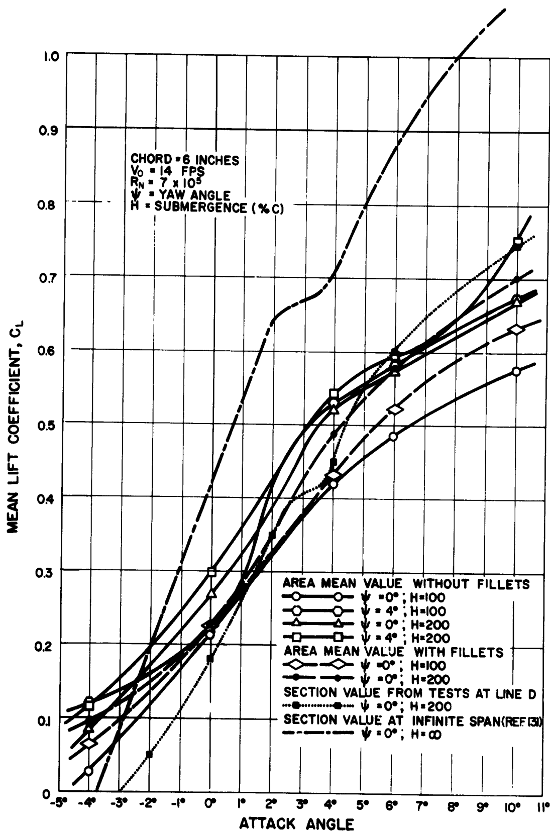
Fig. 6 - Mean Pressure Lift Coefficients of Foli 16-509 for the Area (Span = 2/3 Chord) Adjacent to an End Strut 16-012
