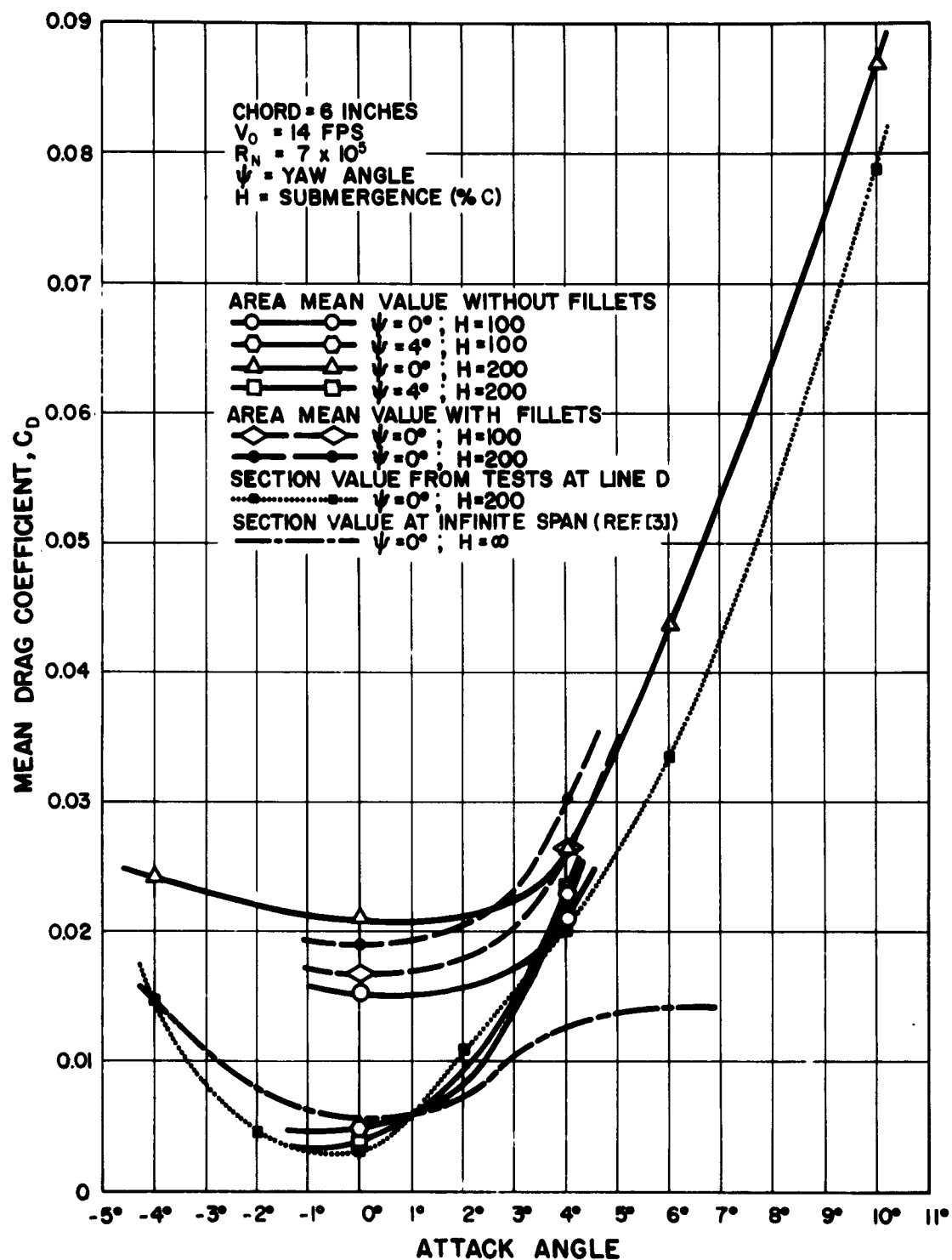
Fig. 7 - Mean Pressure Drag Coefficients of Foli 16-509 for the Area (Span = 2/3 Chord) Adjacent to an End Strut 16-012
