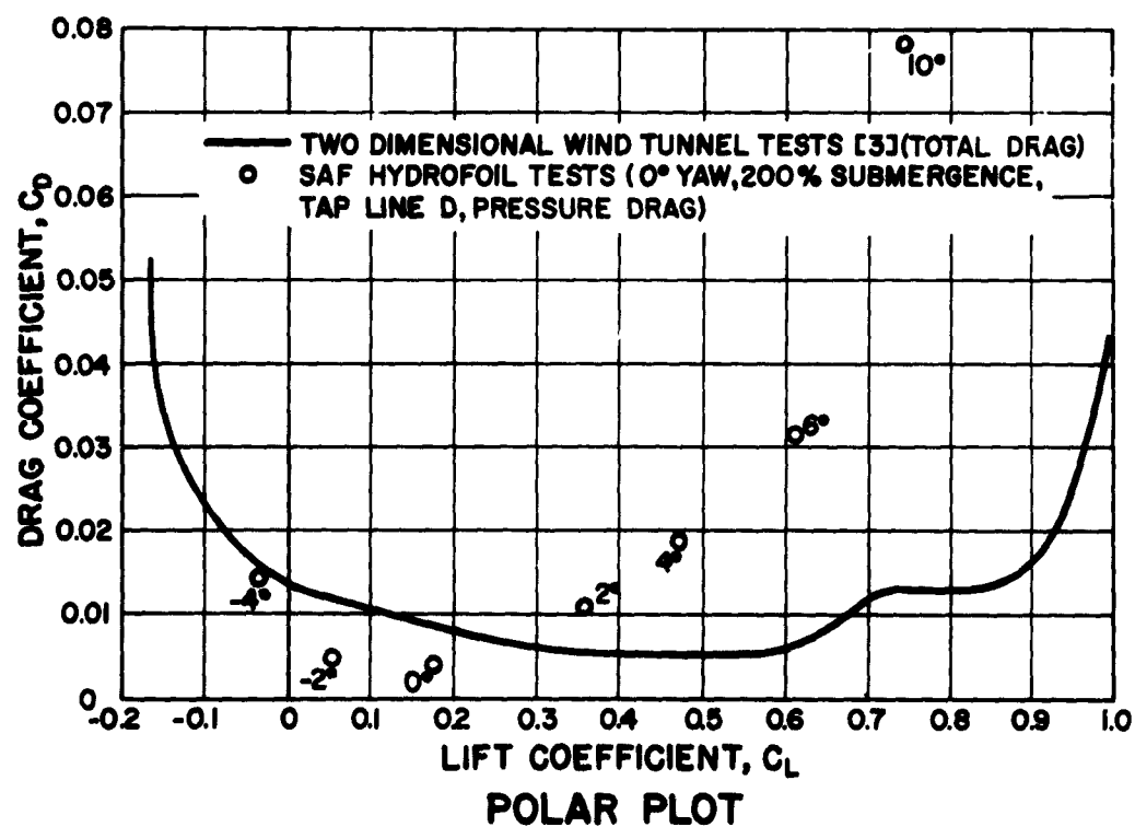
Fig. 14 - Comparative Lift and Drag Data for Foil 16-509 at Tap Line D
