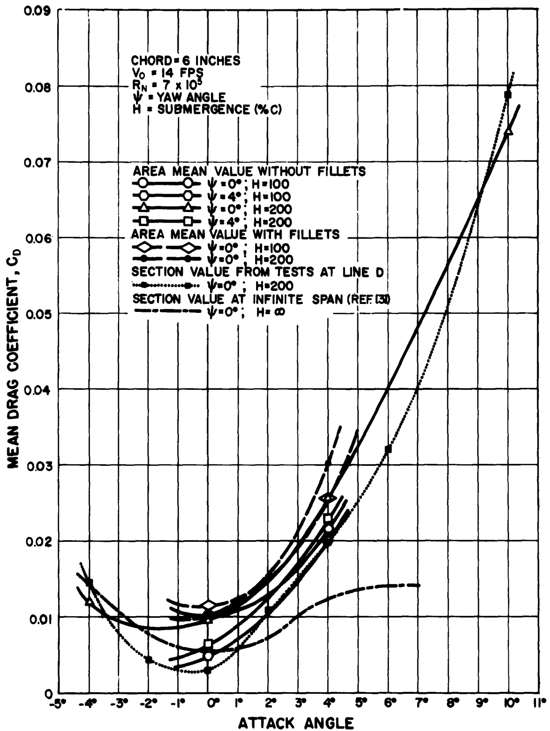
Fig. 9 - Mean Pressure Drag Coefficients of Foli 16-509 for the Area (Span = 2/3 Chord) Adjacent to a Center Strut 16-012
