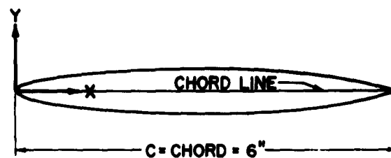
STRUT SECTION—NACA 16-012
