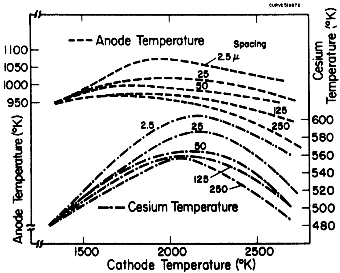
Fig.11-Optimum anode and cesium temperatures as a function of cathode temperature.
