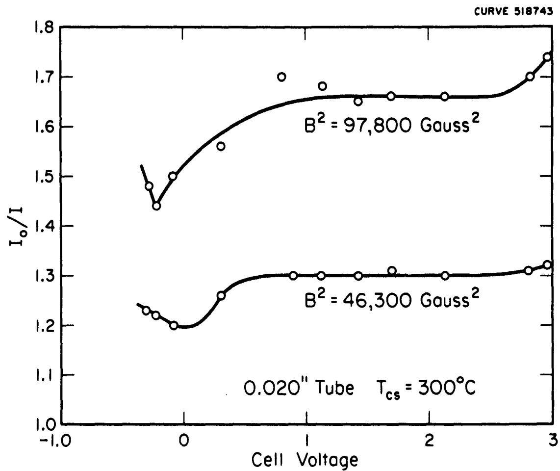
Fig. 5 - Dependence of I_o/I on cell potential for two different magnetic field strengths.
