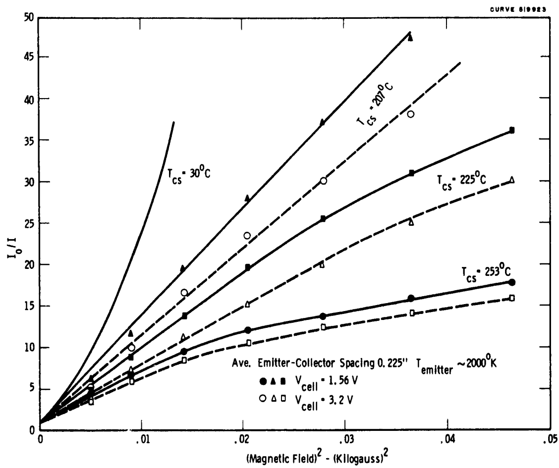
Fig. 3— I_0/I vs. (Magnetic Field) 2
