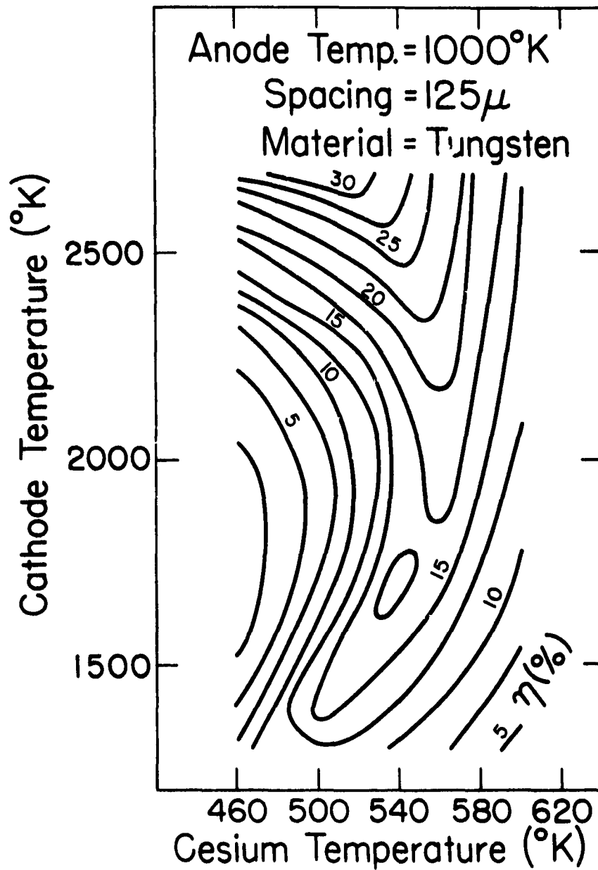
Fig.8 - Efficiency as a function of cathode and cesium temperatures
