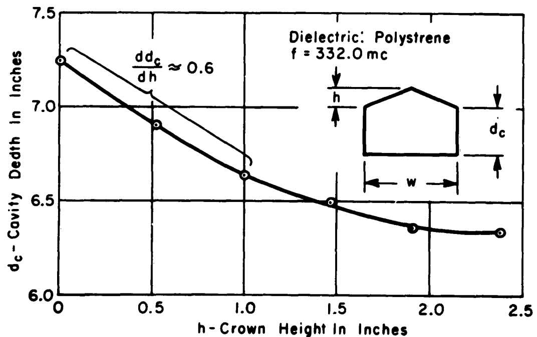
Fig. 17. Required cavity depth for various crown heights.
