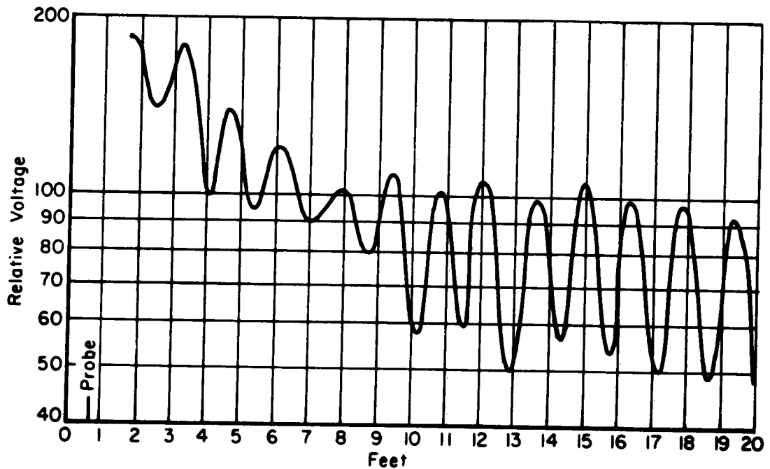
Fig. 33. Relative voltage along antenna aperture.
