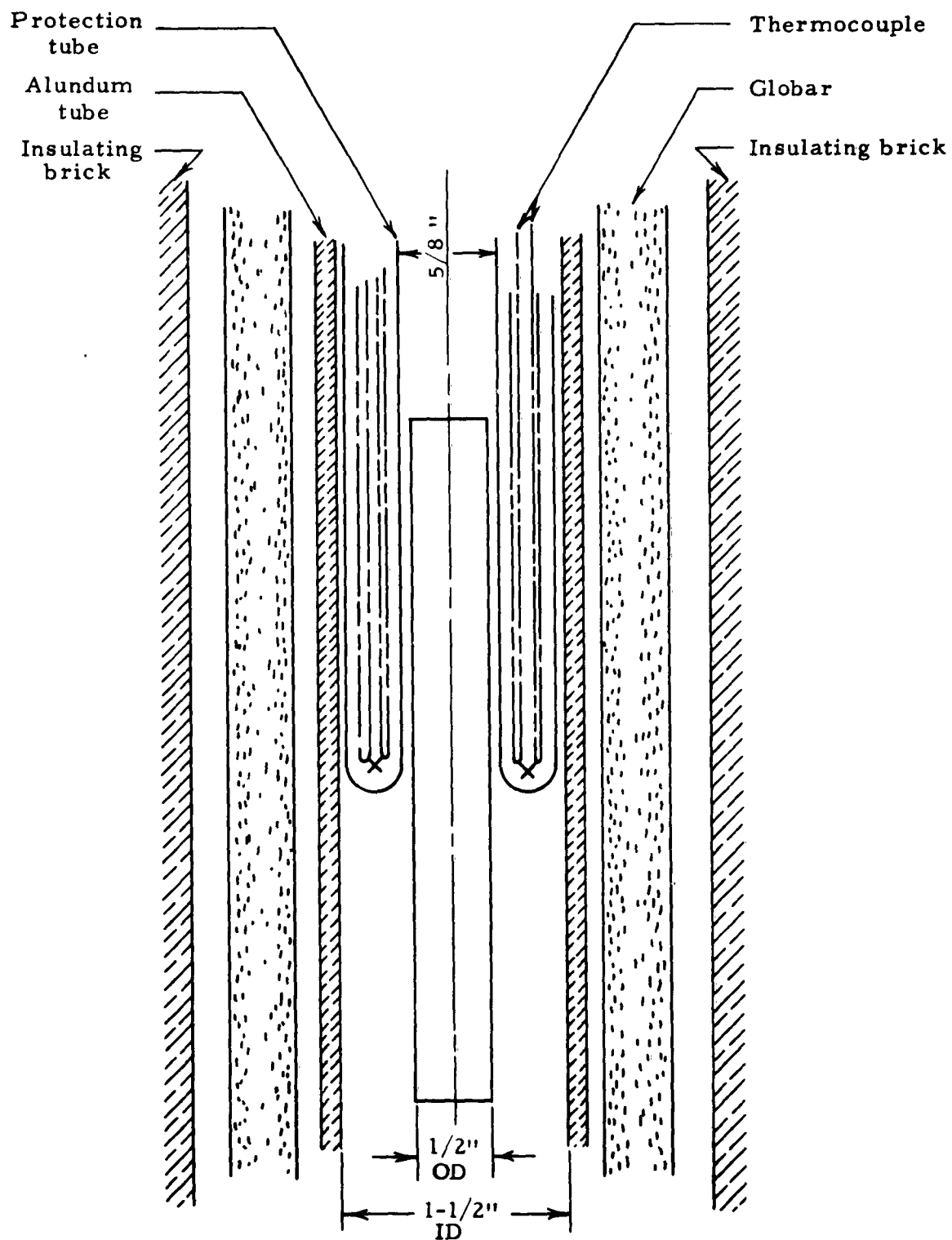
Figure 18 CROSS SECTIONAL VIEW OF SPECIFIC HEAT FURNACE
