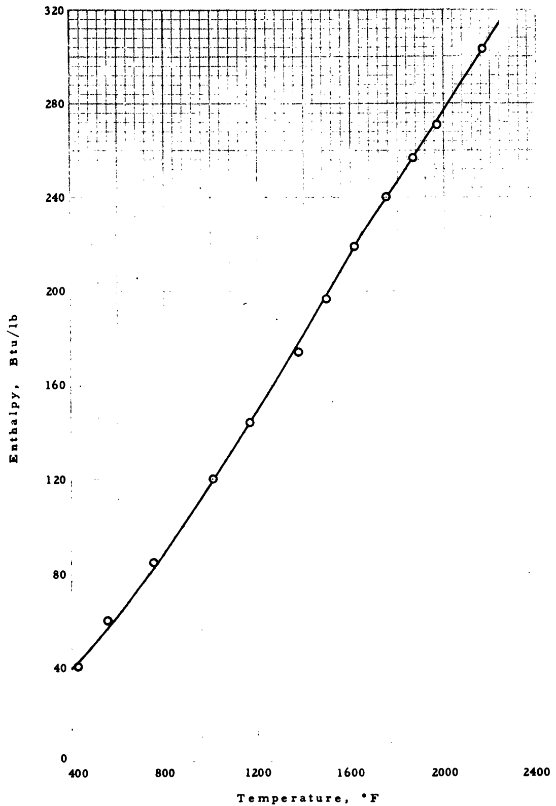
Figure 22 ENTHALPY OF CRUCIBLE HNM
