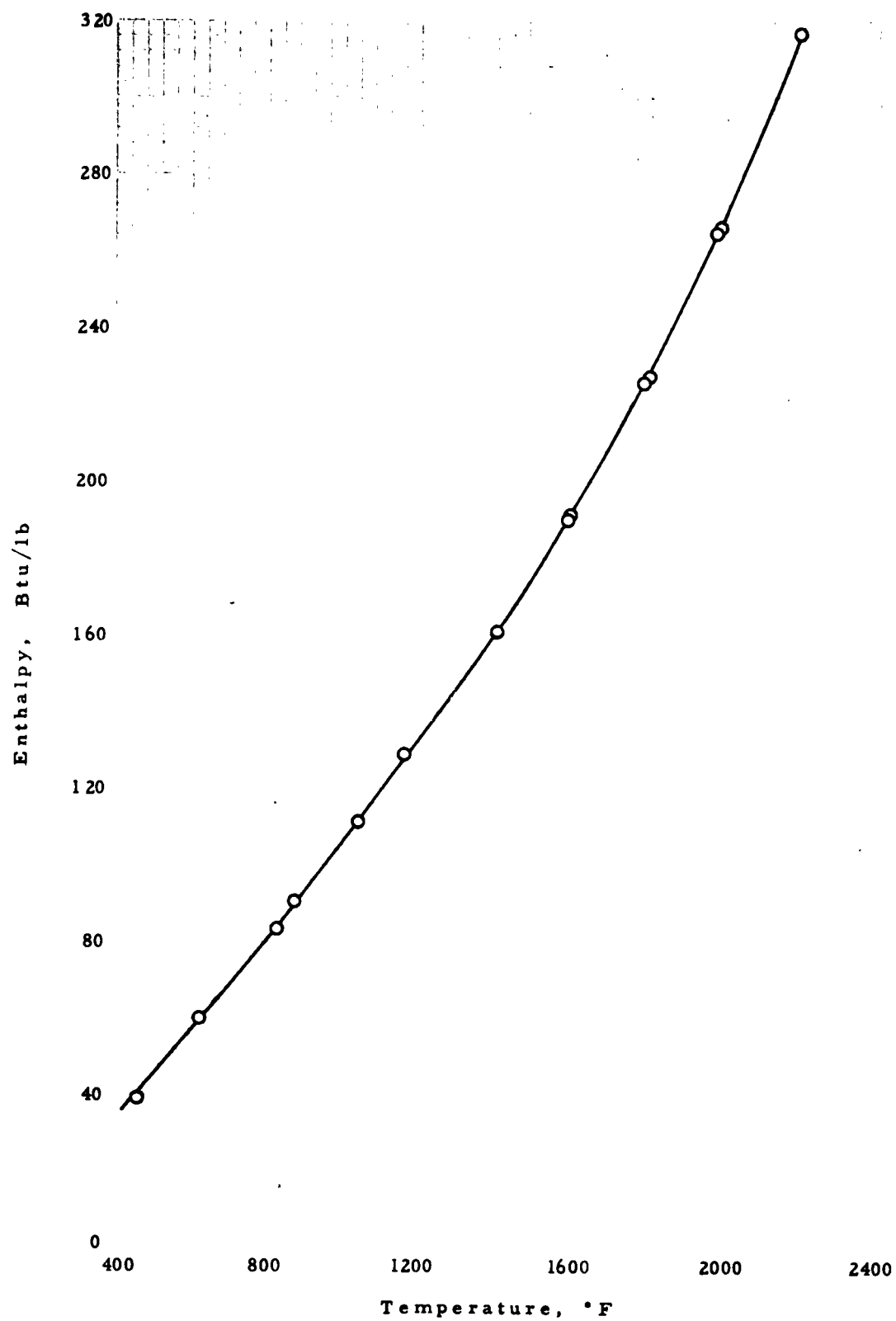
Figure 24 ENTHALPY OF INCO 713C
