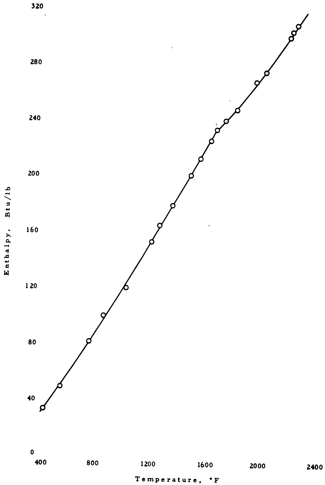
Figure 21 ENTHALPY OF AM 355
