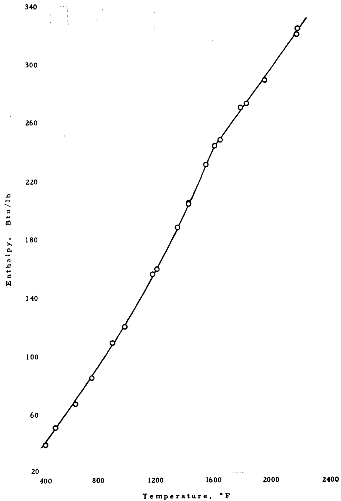
Figure 19 ENTHALPY OF STAINLESS STEEL TYPE 420
