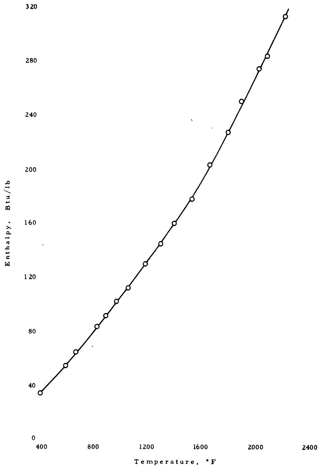
Figure 28 ENTHALPY OF RENE 41
