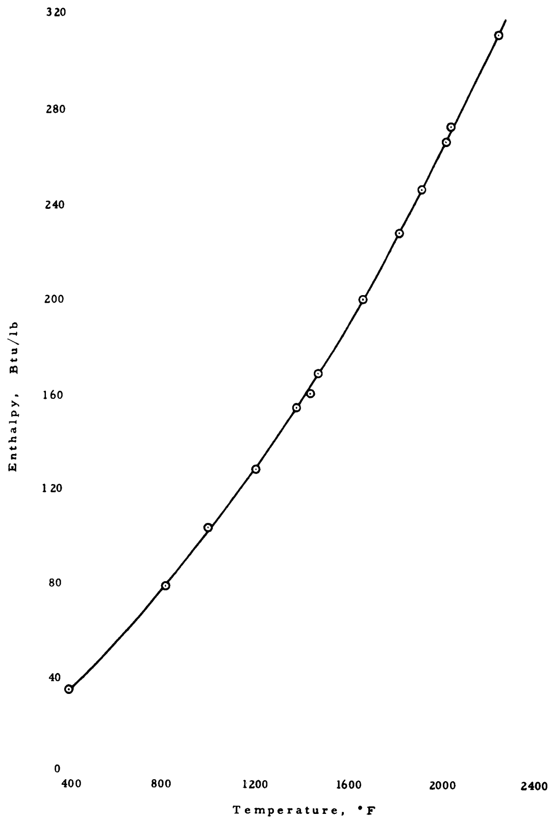
Figure 27 ENTHALPY OF M 252
