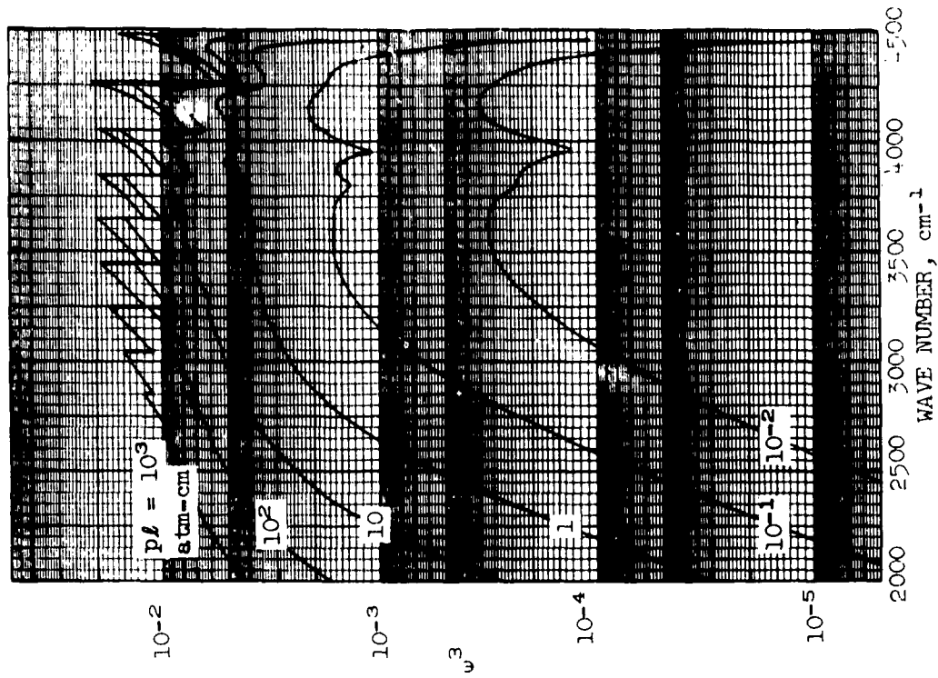
FIGURE 14. SPECTRAL EMISSIVITY OF HF AT T = 2000°K (Toppler Line Scope)
