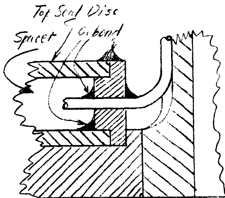
Spacers and Top Seal Disc in Place Fig. 27
