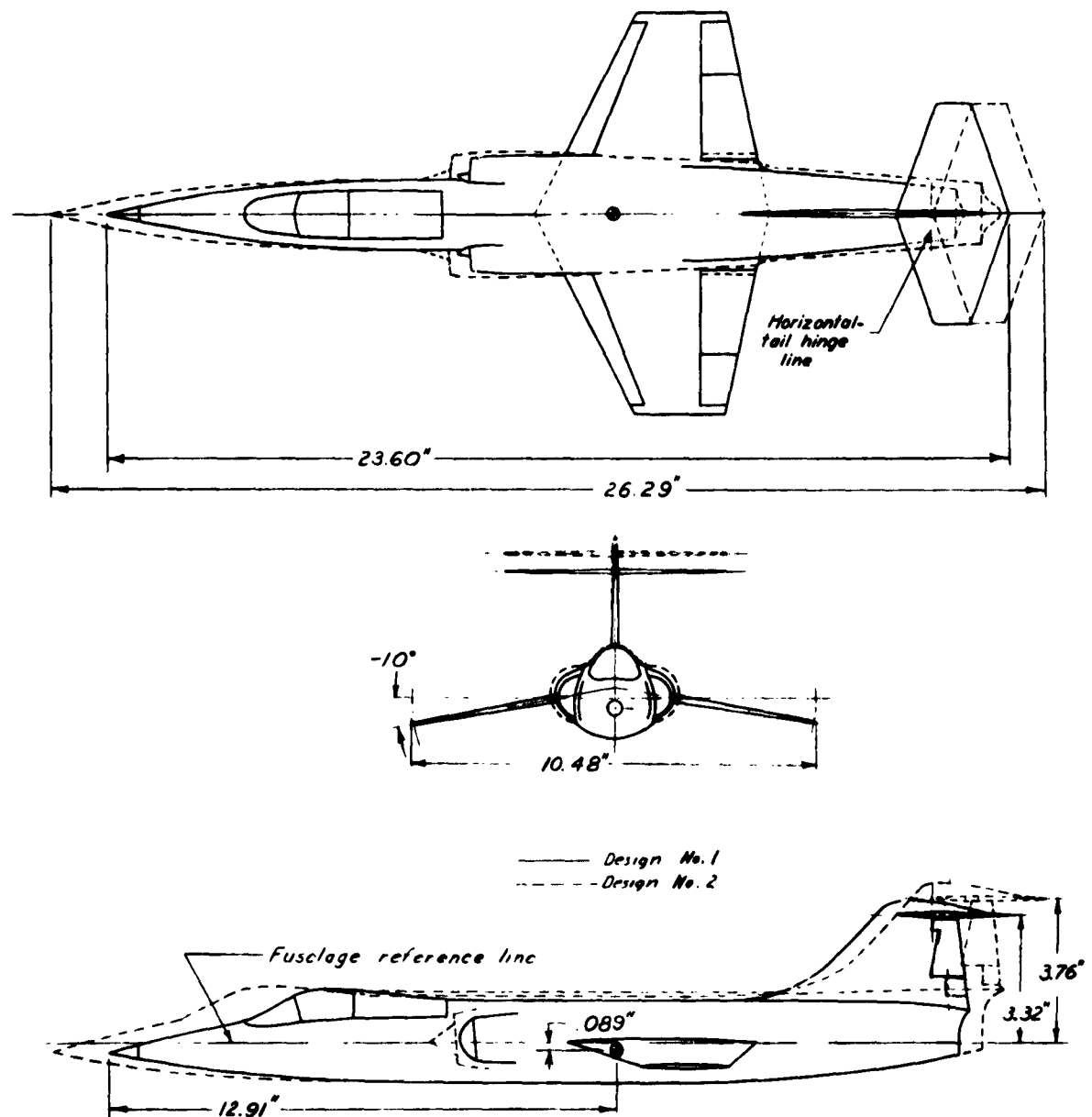
Figure 1.- Three-view drawings of the 1/25-scale models of design 1 and 2 as tested in the Langley 20-foot free-spinning tunnel. Center-of-gravity position shown is for the design 1 normal take-off loading.
