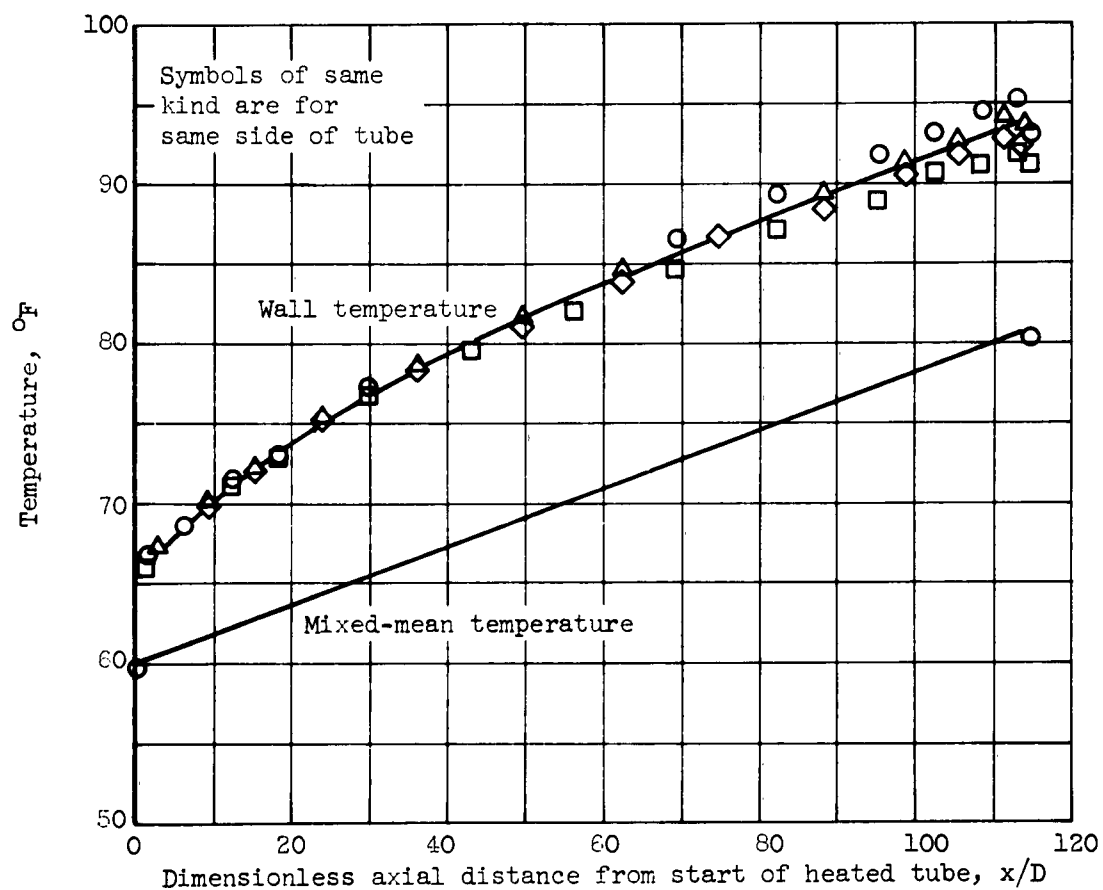
Figure 18. - Representative wall temperature profile for downflow with heating. Peclet number, 1130.
