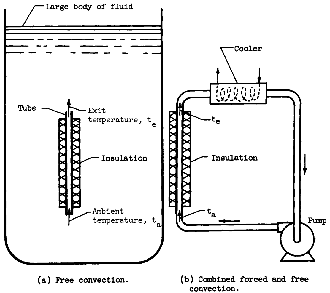
Figure 1. - Combined forced and free convection.
