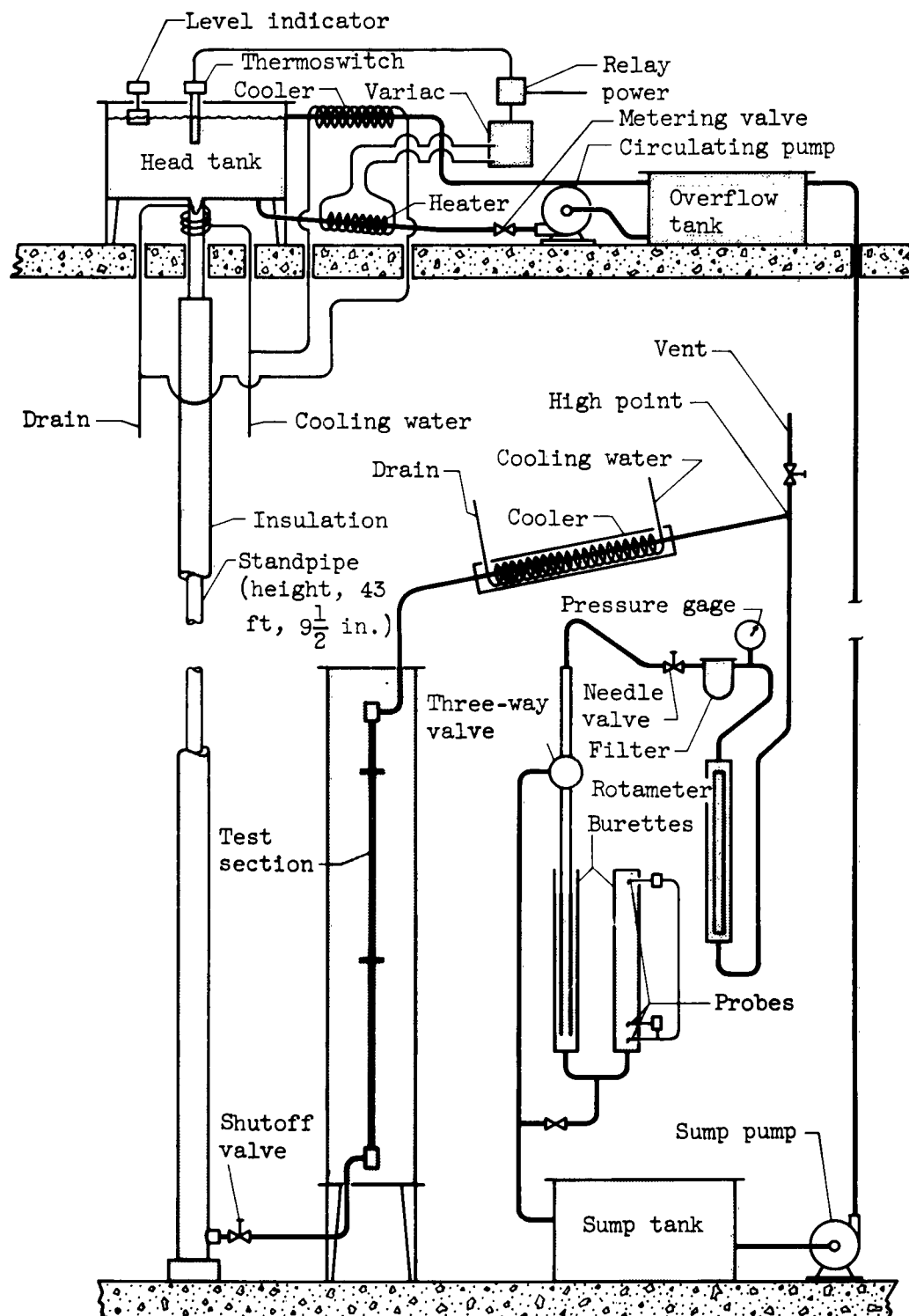
Figure 3. - Heat-transfer loop.
