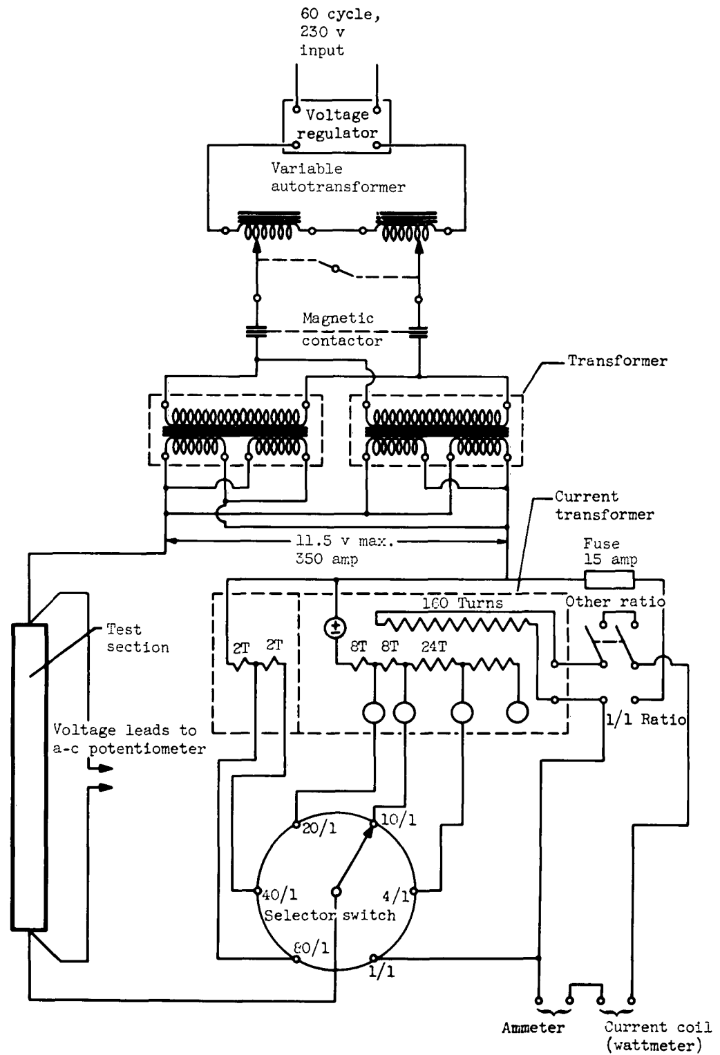
Figure 7. - Power circuit.
