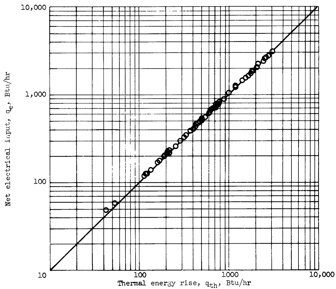
Figure 20. - Heat balance.
