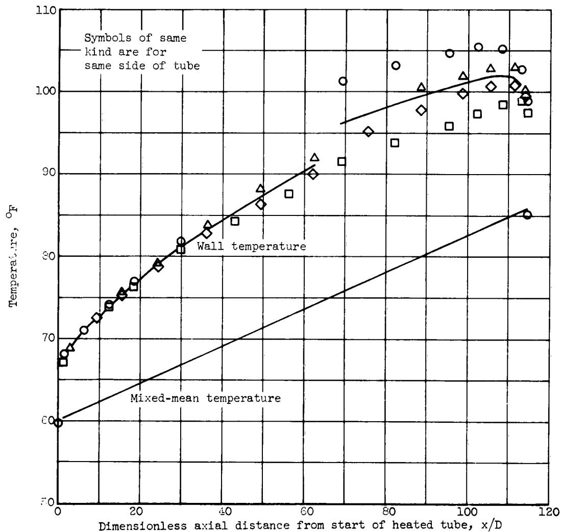
Figure 18. - Concluded. Representative wall temperature profile for down-flow with heating. Peclet number, 1130.
