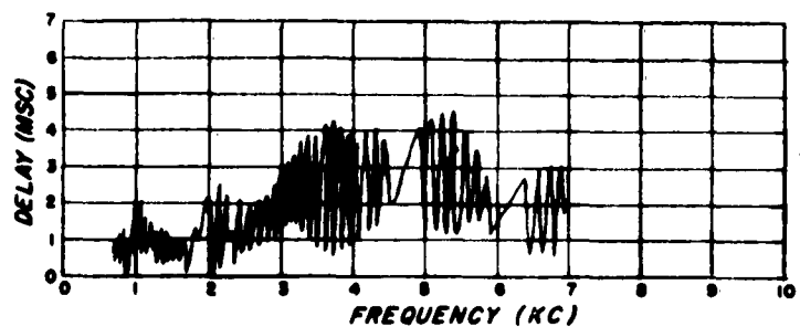
Figure 18. (continued) Test Delay Line Data Curves
