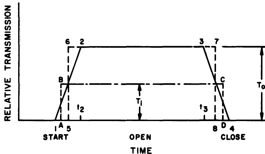
ROTARY SHUTTER CYCLE
