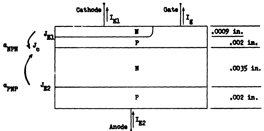
Figure 1- PNPN Structure
