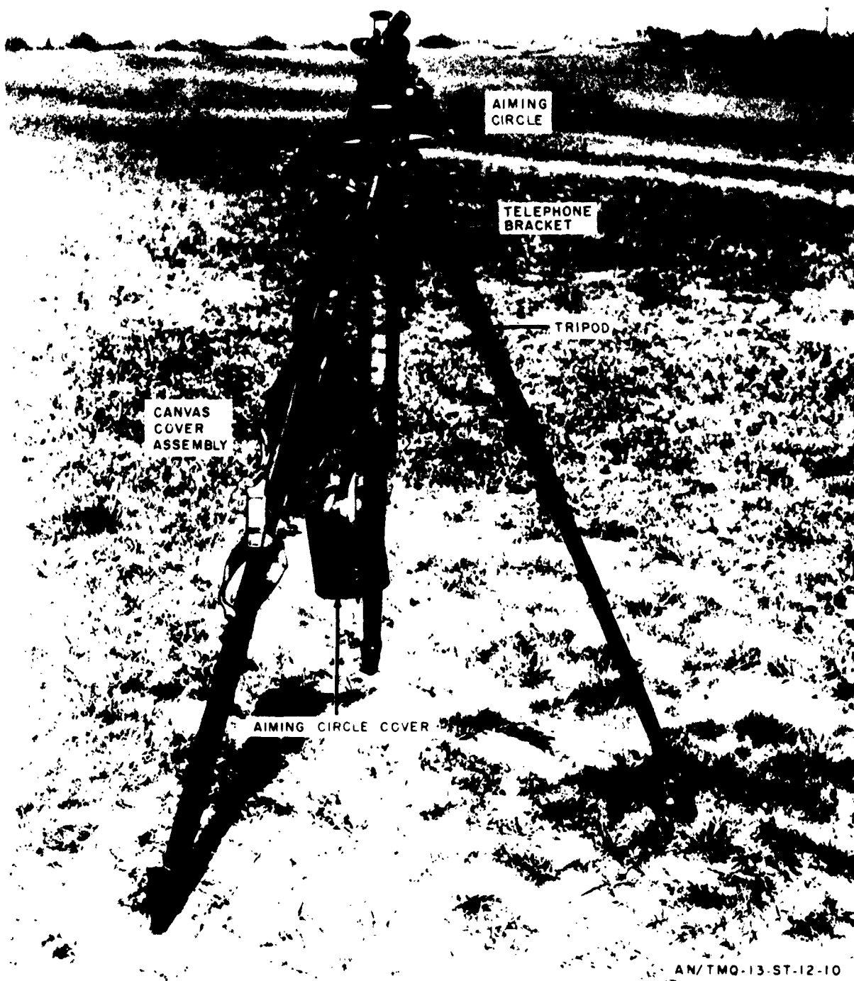
Fig. 3. Aiming Circle Mounted on Tripod
