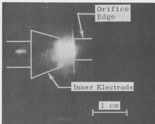
Fig. 13 Photograph of Internal Arc of Plasma Jet
