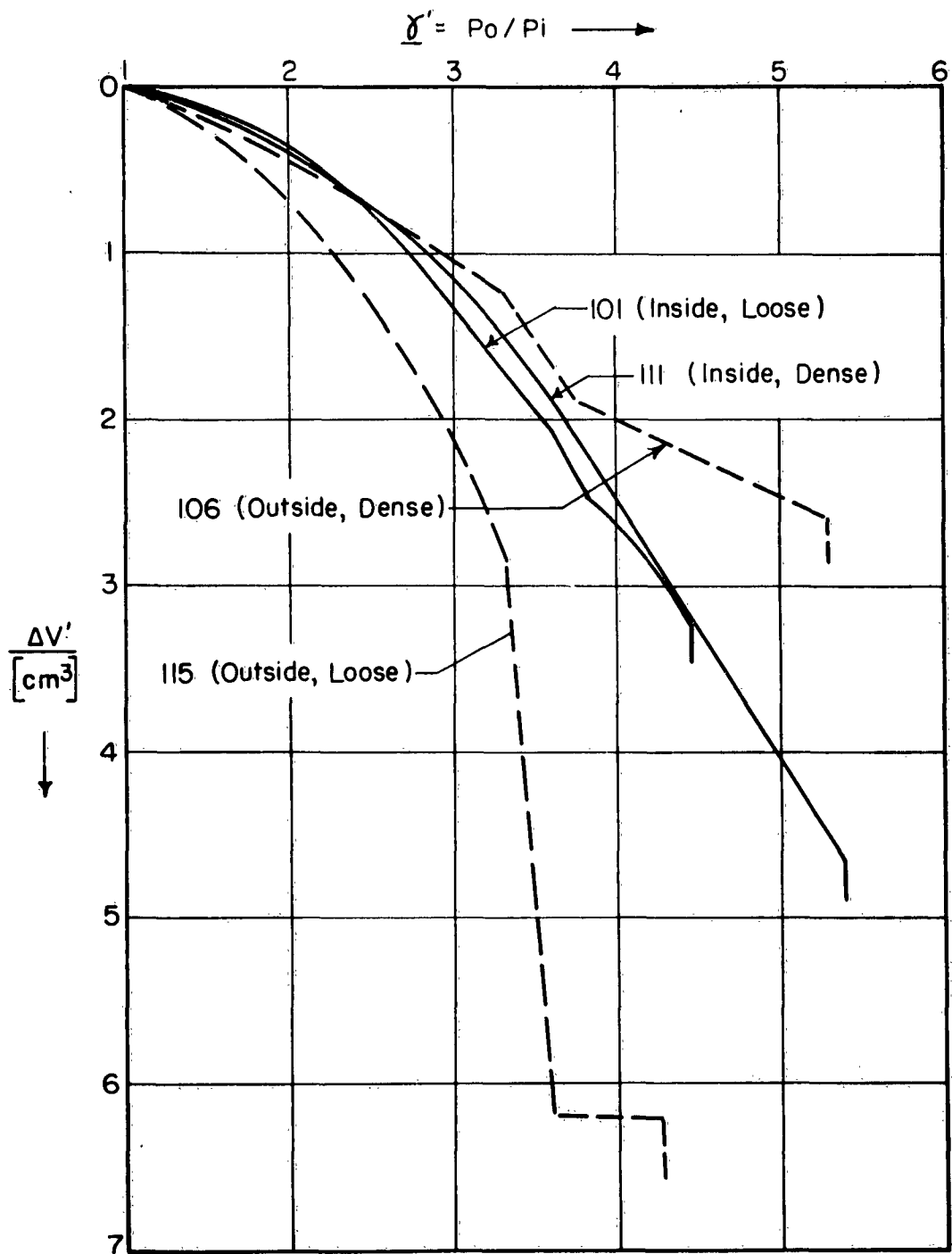
FIGURE K.8 TYPICAL VOLUME CHANGES DURING TEST DATA OF \frac{1}{4} " SAMPLES
