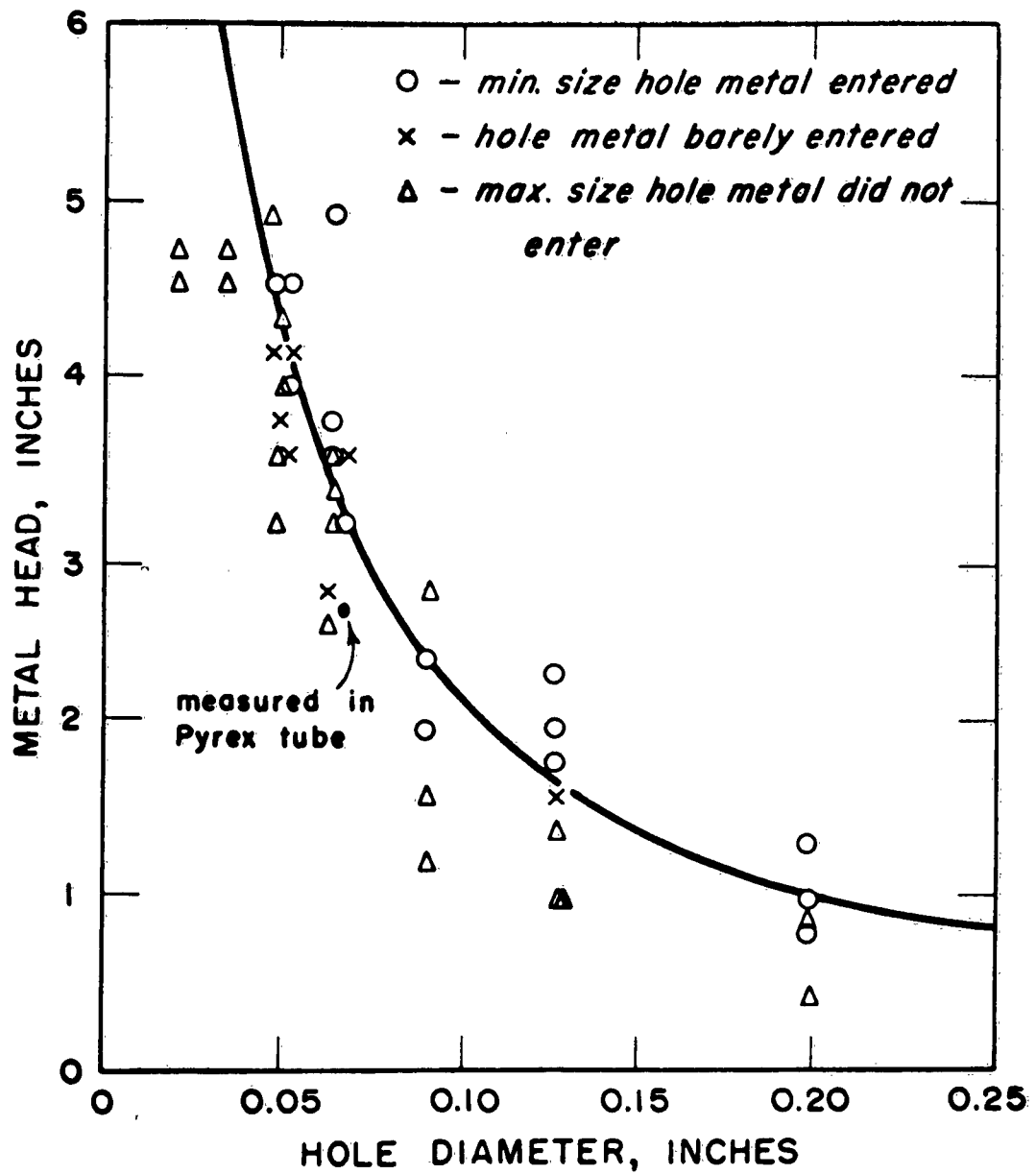
Figure 10. Minimum metal head necessary to force metal into small diameter holes. Curve corresponds to surface tension ( \gamma ) equal to 800 dynes/cm.
