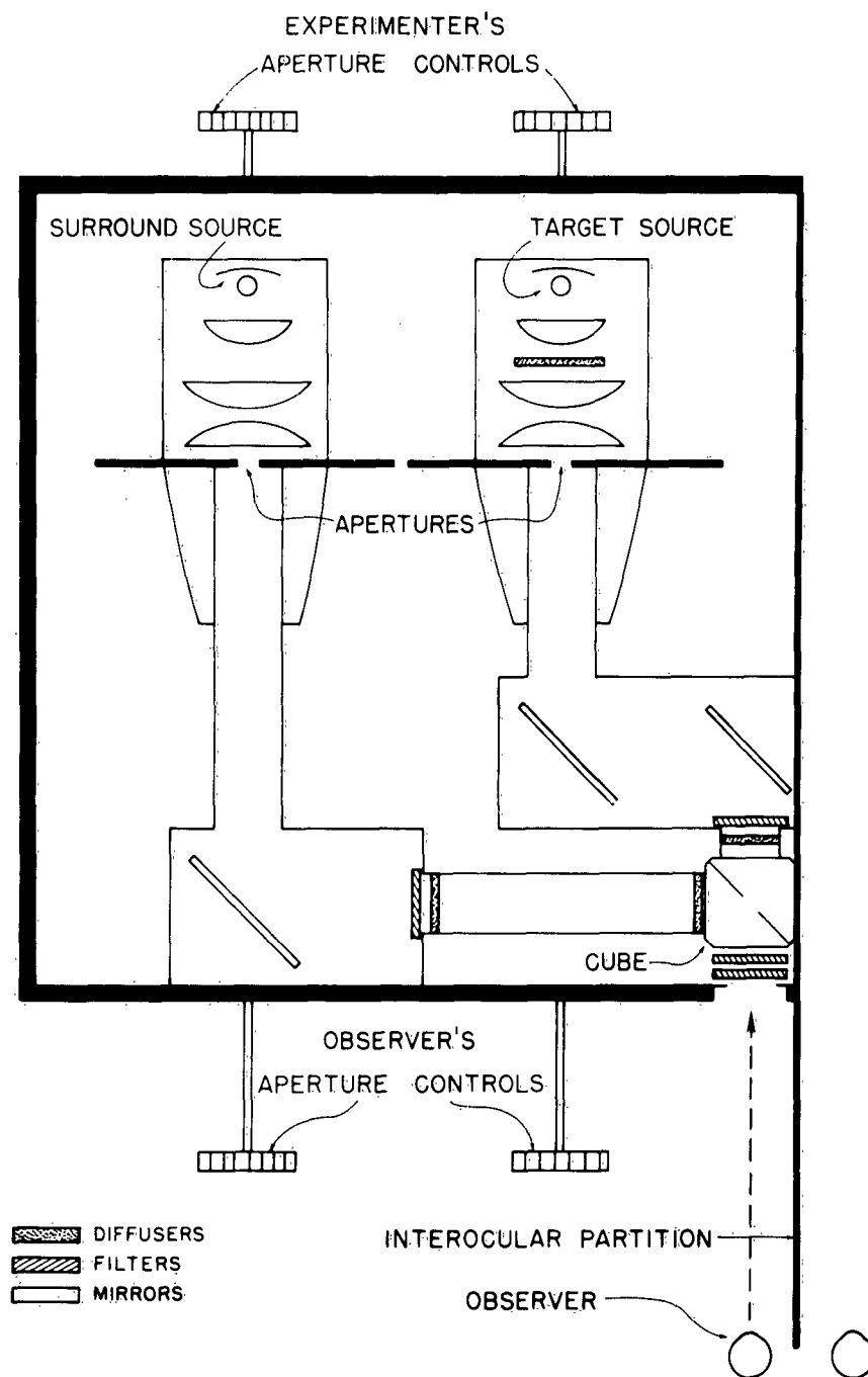
APPARATUS FOR THE STUDY OF CONTRAST
