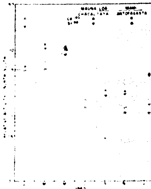
Fig. 10 - Effect of altitude on the relative fission product concentrations at various sites North and South of the equator.
