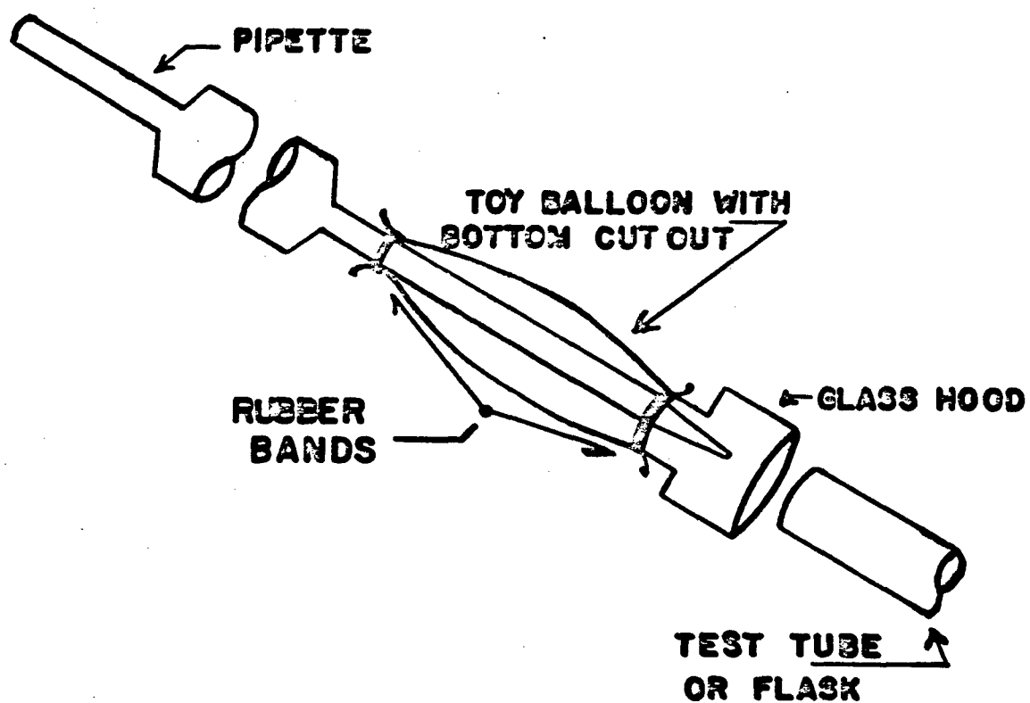
Figure 58. Pipette Hood Device.
