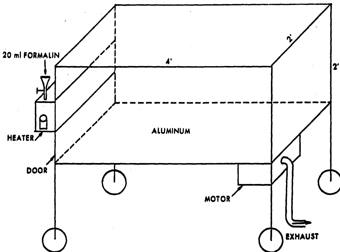
Figure 50. Formaldehyde Fumigation Box.
