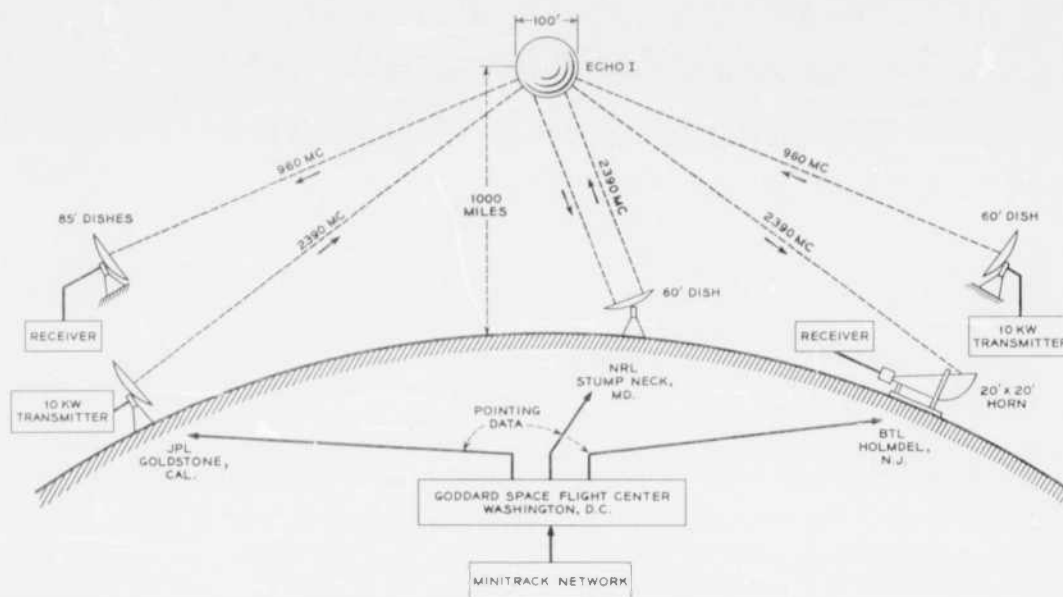
Figure 1 — General features of the Project Echo experiment
