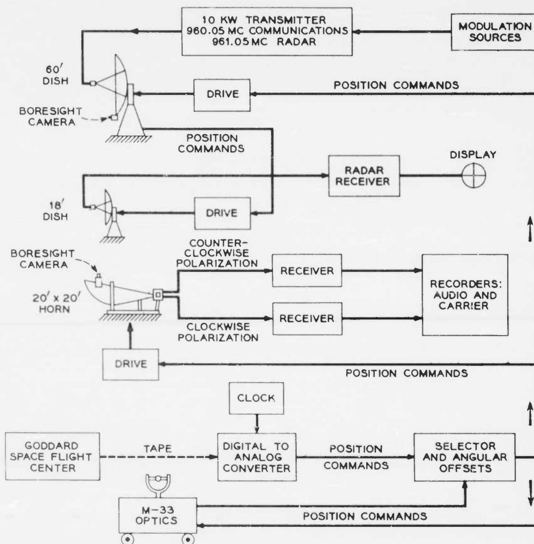
Figure 3 — Block diagram of the BTL facilities
