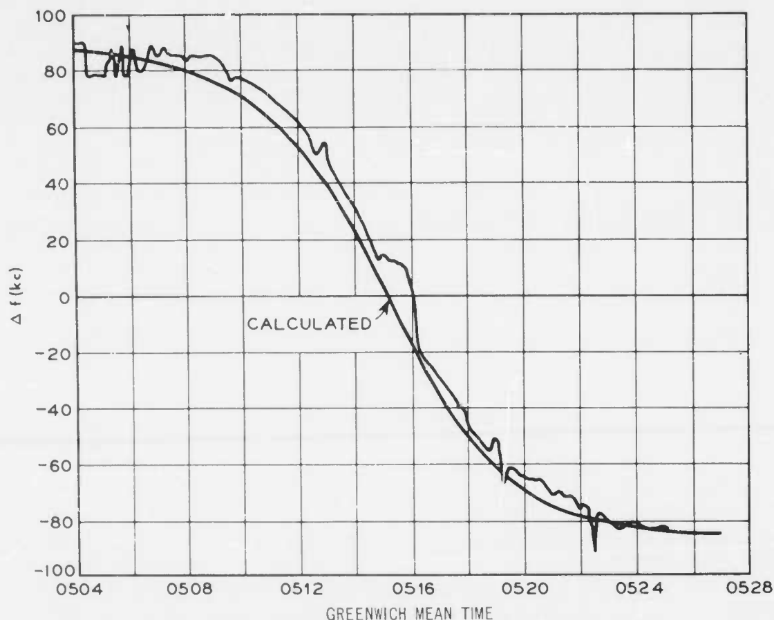
Figure 25 — Observed doppler shift on pass 217, NRL to BTL at 2390 Mc
