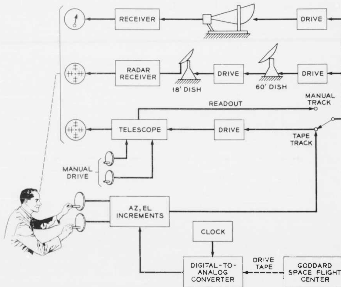
Figure 4 — Block diagram of BTL tracking modes
