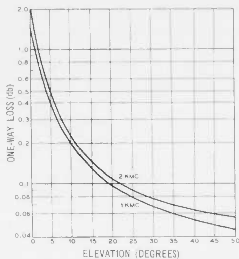
Figure 7 — Absorption due to atmospheric oxygen and water vapor
