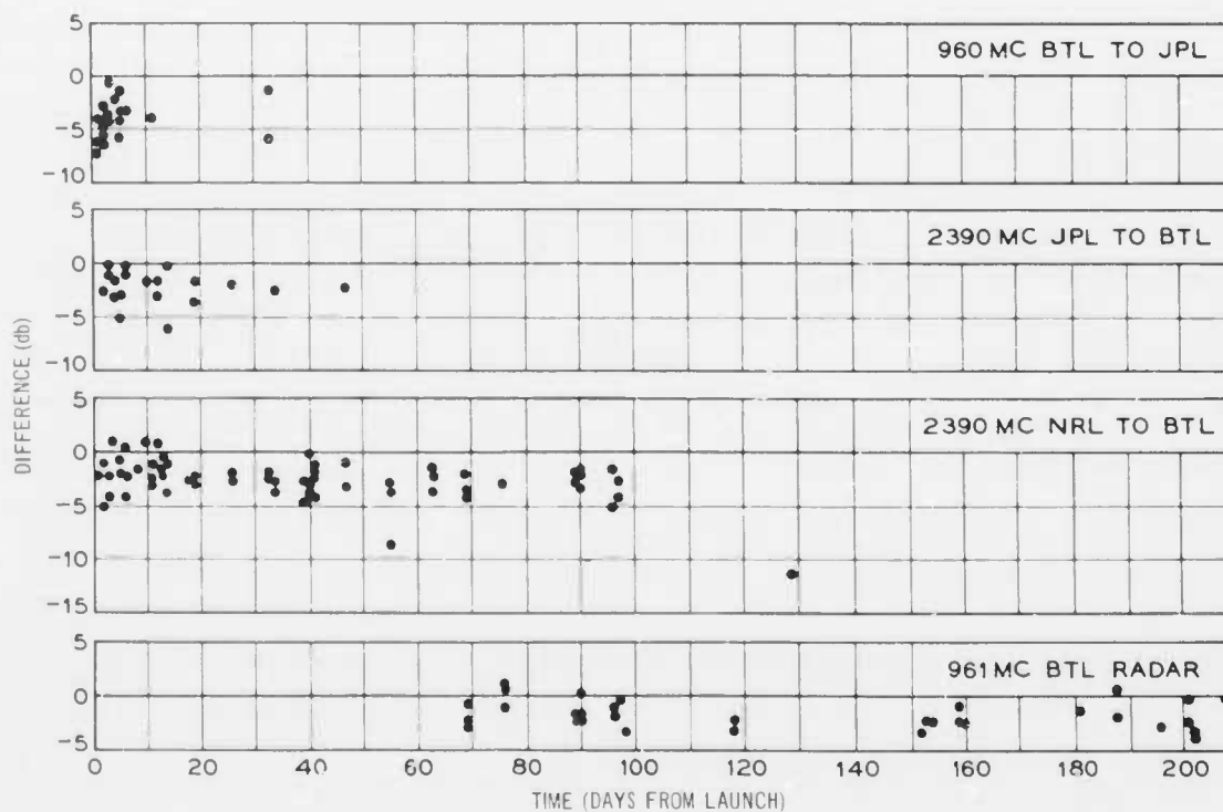
Figure 9 — Difference in decibels between predicted and observed signal power
