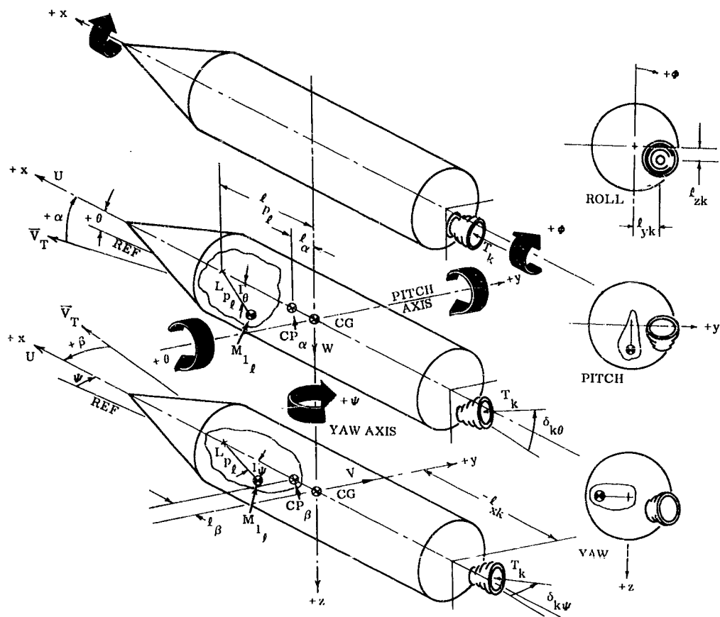
Figure 3-6. Three-Axes Schematic of a Boost Vehicle
