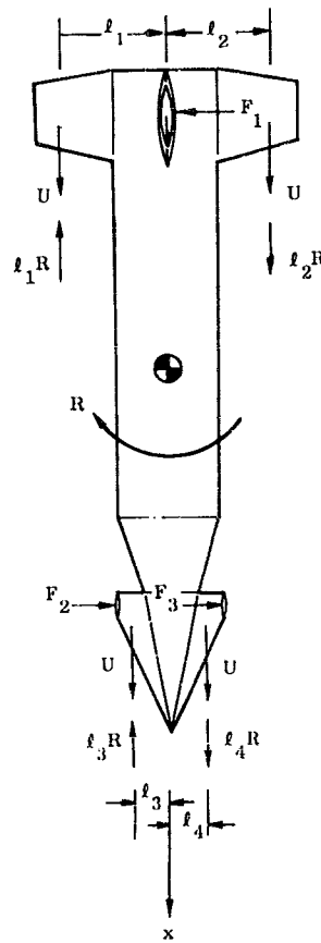
Figure 3-10. Aerodynamic Forces Due to Yaw Rate on a Ballistic Booster with Lifting Surfaces
