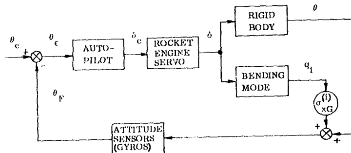
Figure 2-10. Block Diagram of Control System Including One Elastic Mode
