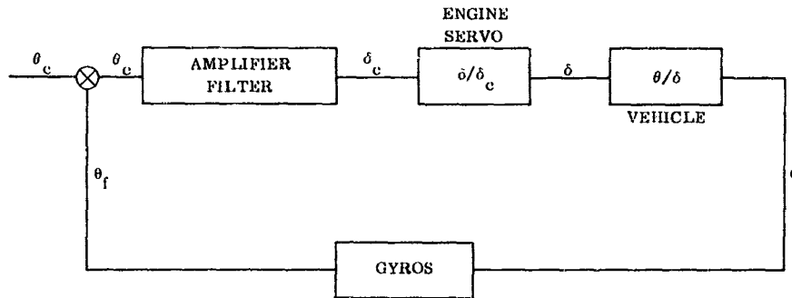
Figure 4-16. Rigid Body and Sloshing Stability Control Loop
