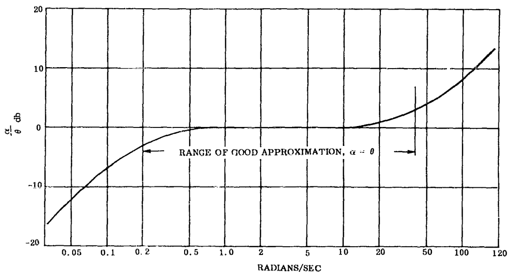
Figure 4-18. Log - Amplitude vs. Frequency Plot of \alpha/\theta Transfer Function for a Large Booster in Flight
