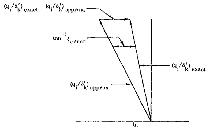
Figure 4-7. Evaluation of Direct Modal Coupling
