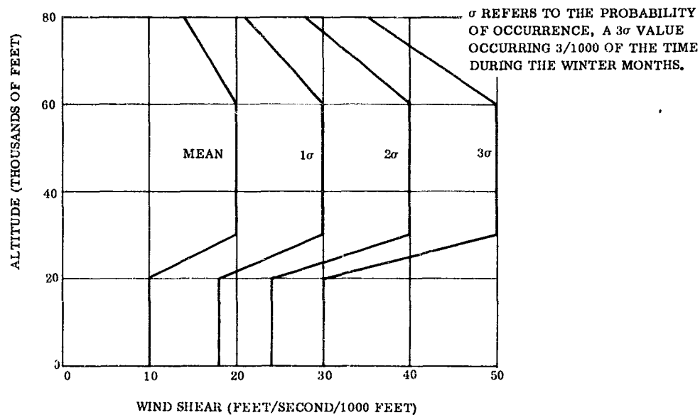
Figure 2-23. Variation of Wind Shear Intensities Versus Altitude for Various Probabilities of Occurrence Over the North American Continent
