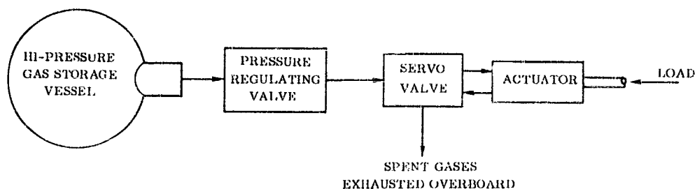
Figure B-37. Stored Gas System
