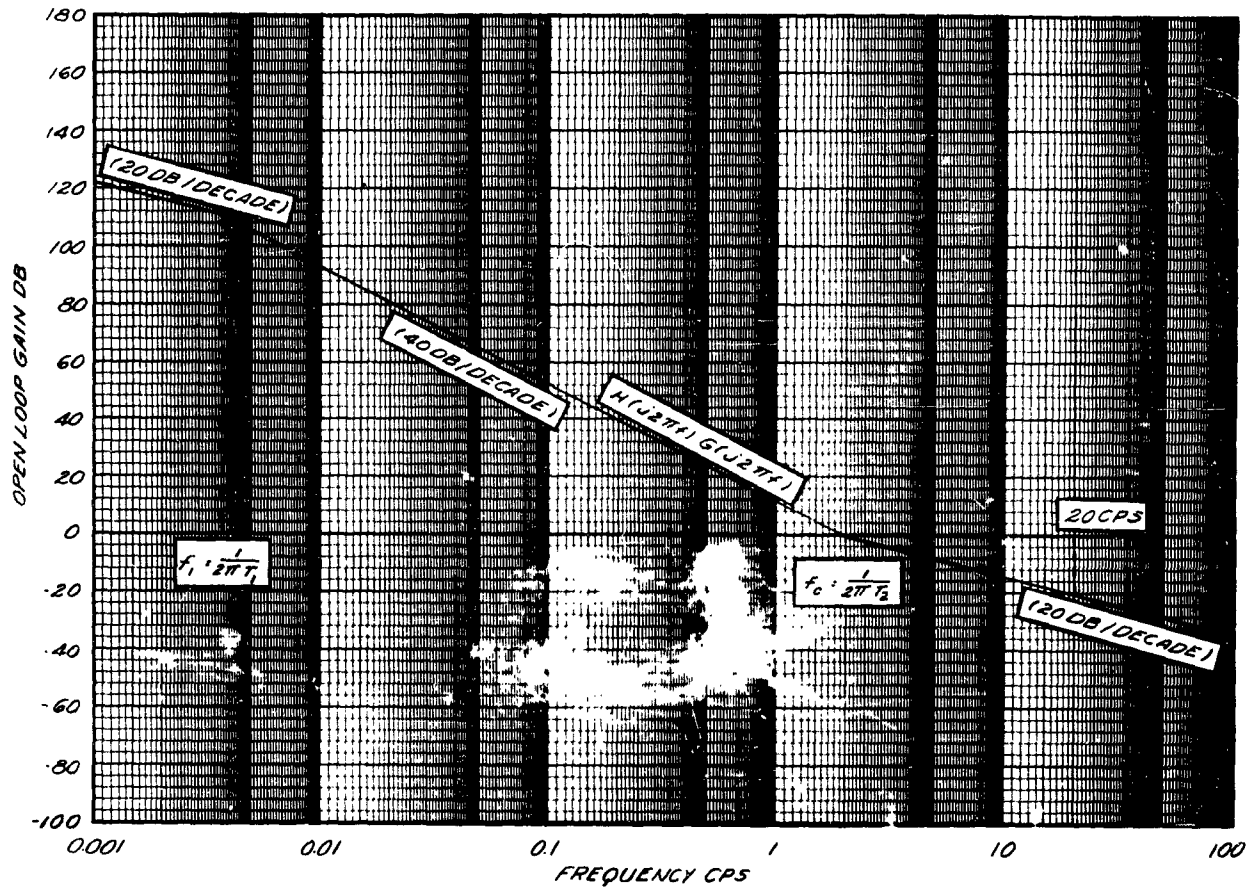
Figure 54. Idealized Open Loop Gain Curve
