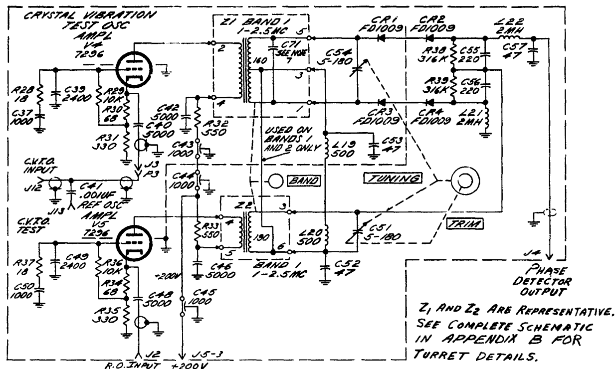
Figure 12. 1-Mc to 110-Mc Tunable Phase Detector, Schematic Diagram
