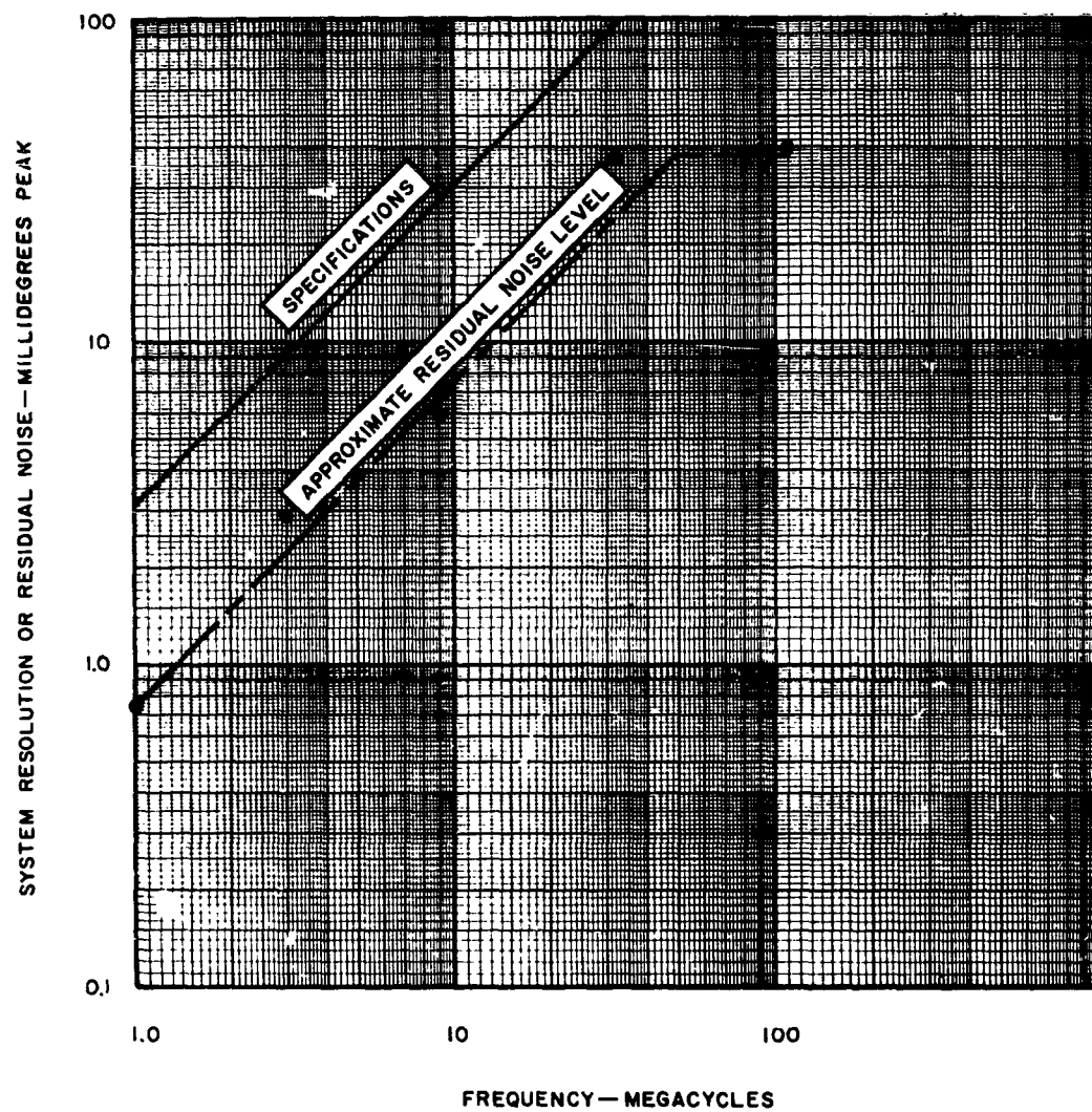
Figure 59. System Performance
