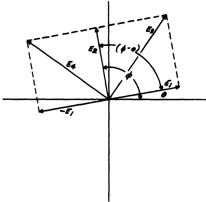
Figure 17. Phase Detector, Phasor Diagram
