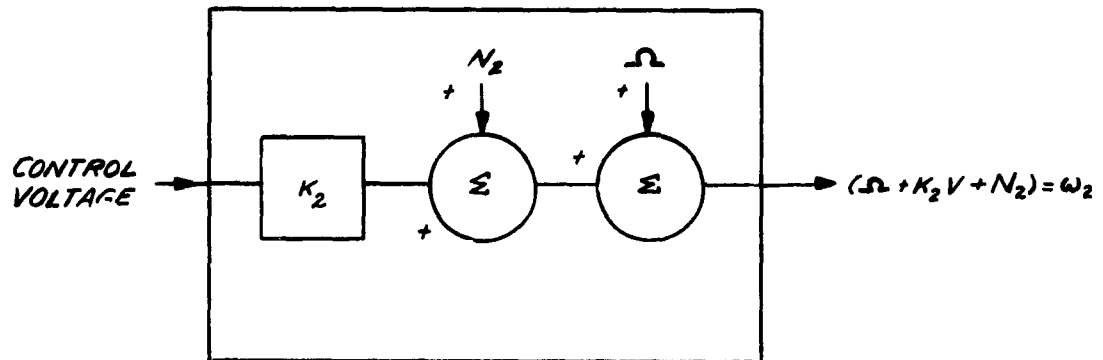
Figure 47. Mathematical Equivalent of Reference Oscillator
