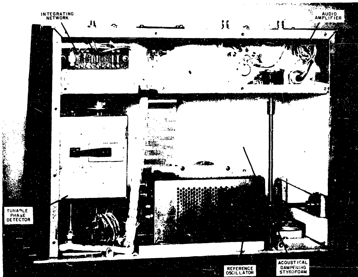
Figure 7. Main Chassis, Bottom View
