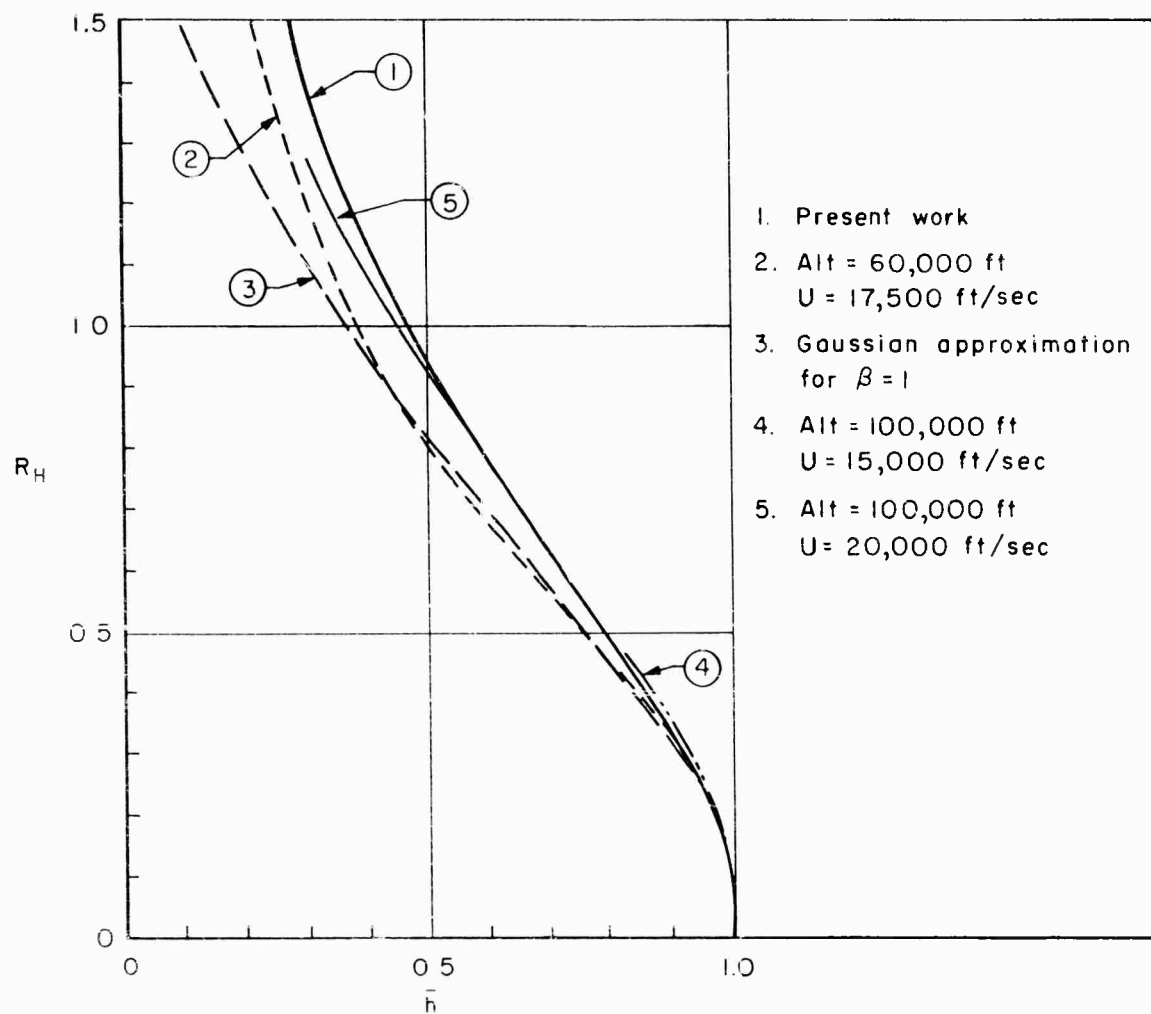
Fig. 4 — The universal enthalpy profile compared with profiles obtained by the method of characteristics in Ref. 1
